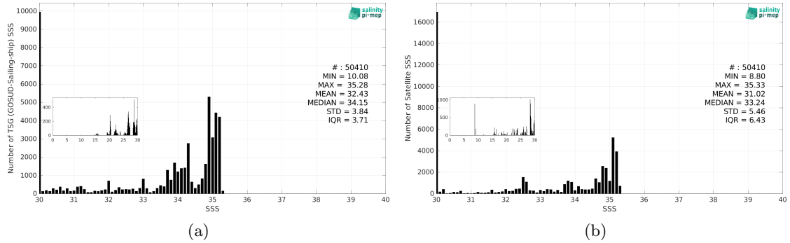
Figure 3: Histograms of SSS from TSG (GOSUD-Sailing-ship) (a) and CCI SSS L4 Merged-OI v4.41 - 7-day running (ESA) (b) considering all match-up pairs per bins of 0.1 over the Arctic Ocean Pi-MEP region and for the full satellite product period.
