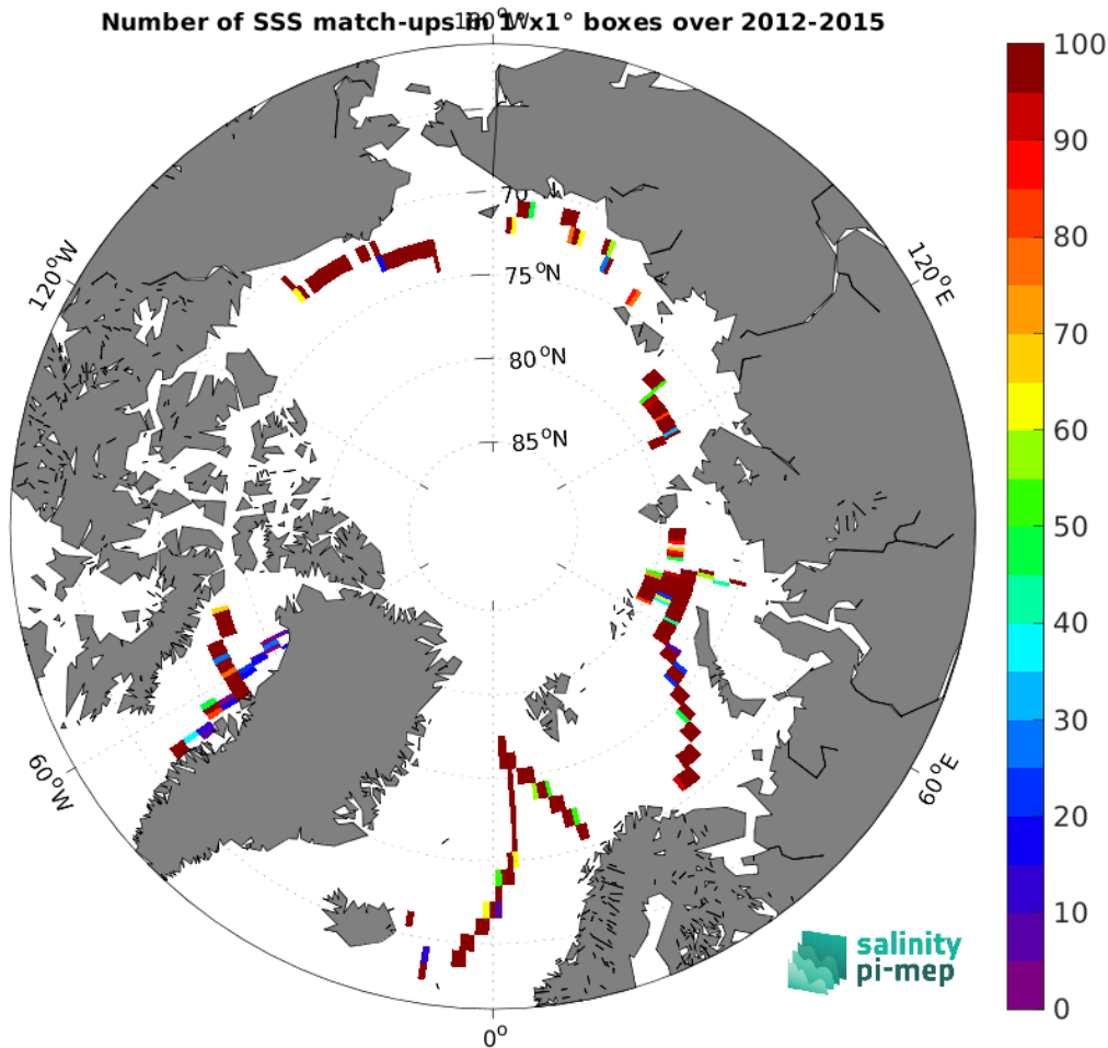
Figure 5: Number of SSS match-ups between TSG (GOSUD-Sailing-ship) SSS and the CCI SSS L4 Merged-OI v4.41 - 7-day running (ESA) SSS product for the Arctic Ocean Pi-MEP region over 1^\circ \times 1^\circ boxes and for the full satellite product period.
