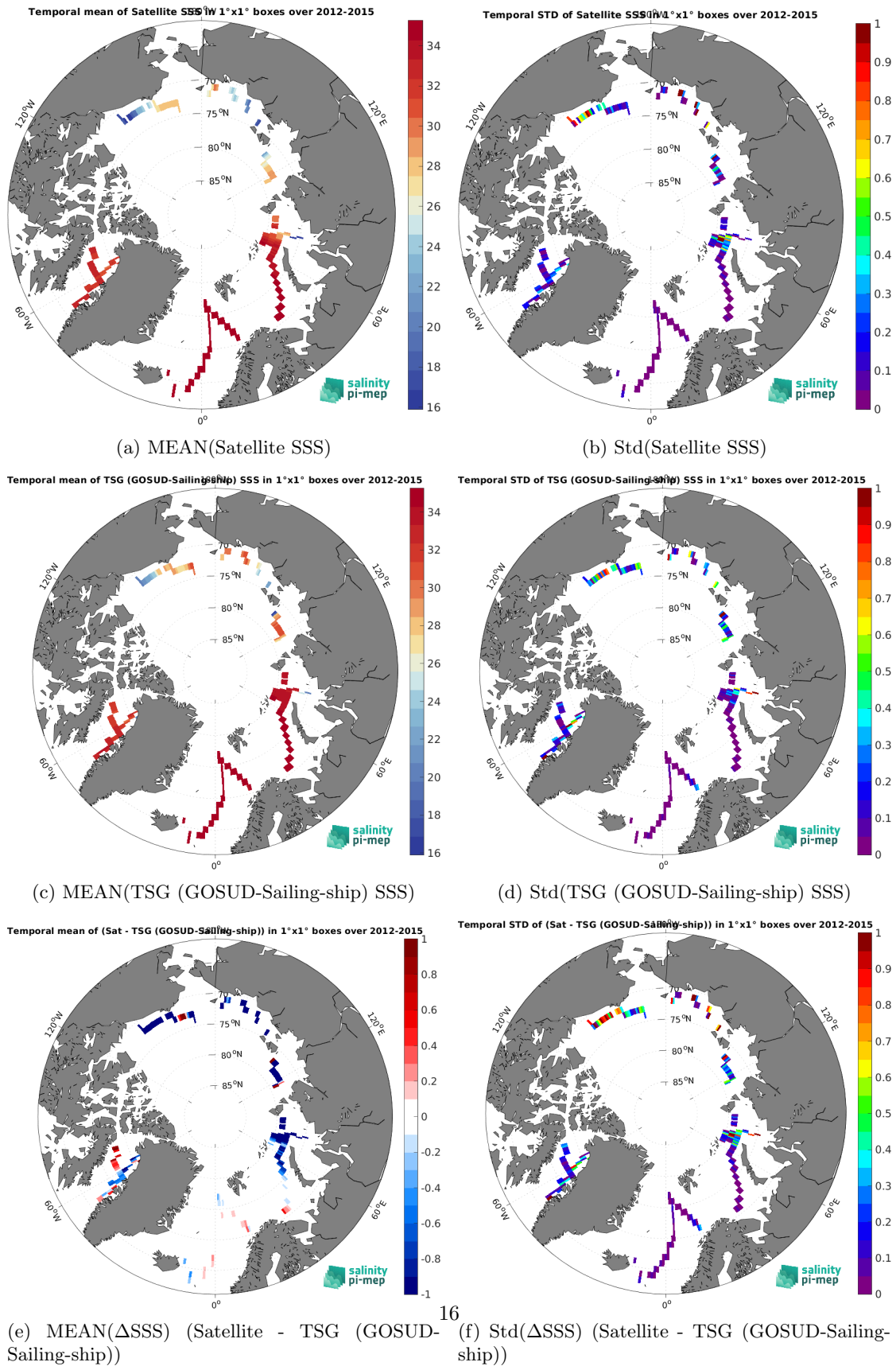
Figure 7: Temporal mean (left) and Std (right) of SSS from CCI SSS L4 Merged-OI v4.41 - 7-day running (ESA) (top), TSG (GOSUD-Sailing-ship) (middle), and of \Delta SSS (Satellite - TSG (GOSUD-Sailing-ship)). Only match-up pairs are used to generate these maps.
