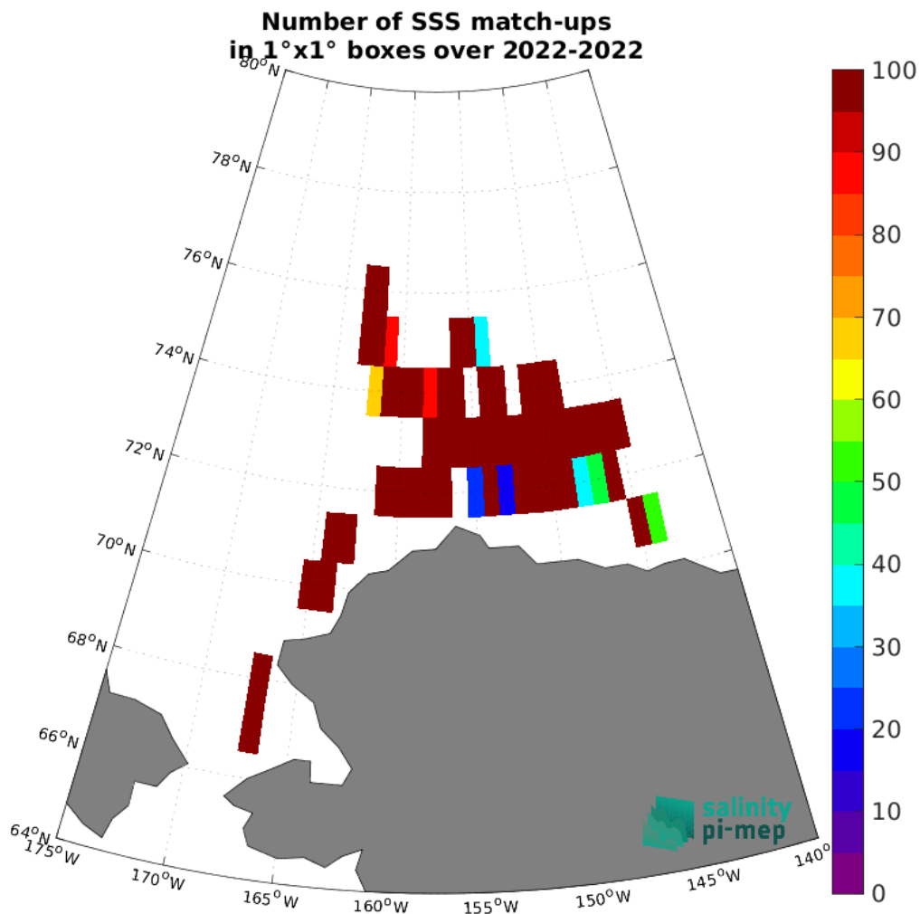
Figure 5: Number of SSS match-ups between SASSIE SSS and the CCI SSS L4 Merged-OI v4.41 - 7-day running (ESA) SSS product for the Arctic Ocean Pi-MEP region over 1^\circ \times 1^\circ boxes and for the full satellite product period.
