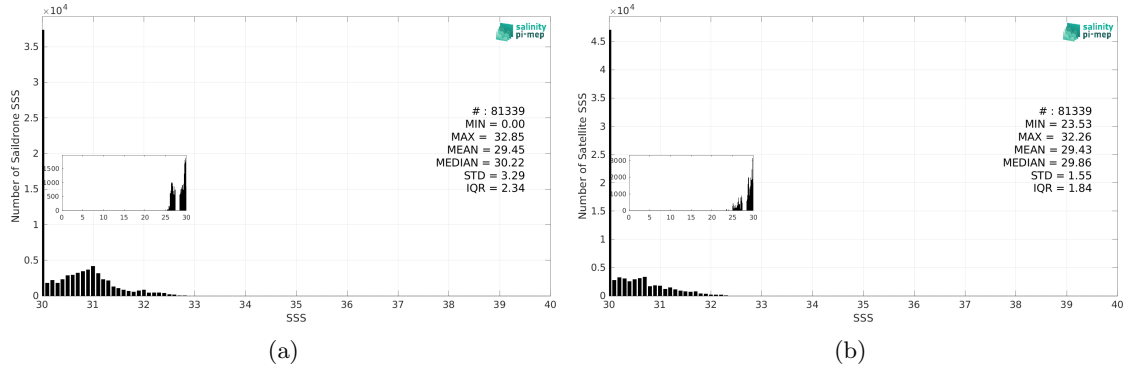
Figure 3: Histograms of SSS from Sairdrone (a) and CCI SSS L4 Merged-OI v4.41 - 7-day running (ESA) (b) considering all match-up pairs per bins of 0.1 over the Arctic Ocean Pi-MEP region and for the full satellite product period.
