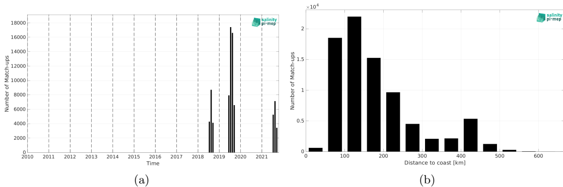
Figure 2: Number of match-ups between Saildrone and CCI SSS L4 Merged-OI v4.41 - 7-day running (ESA) SSS as a function of time (a) and as function of the distance to coast (b) over the Arctic Ocean Pi-MEP region and for the full satellite product period.
