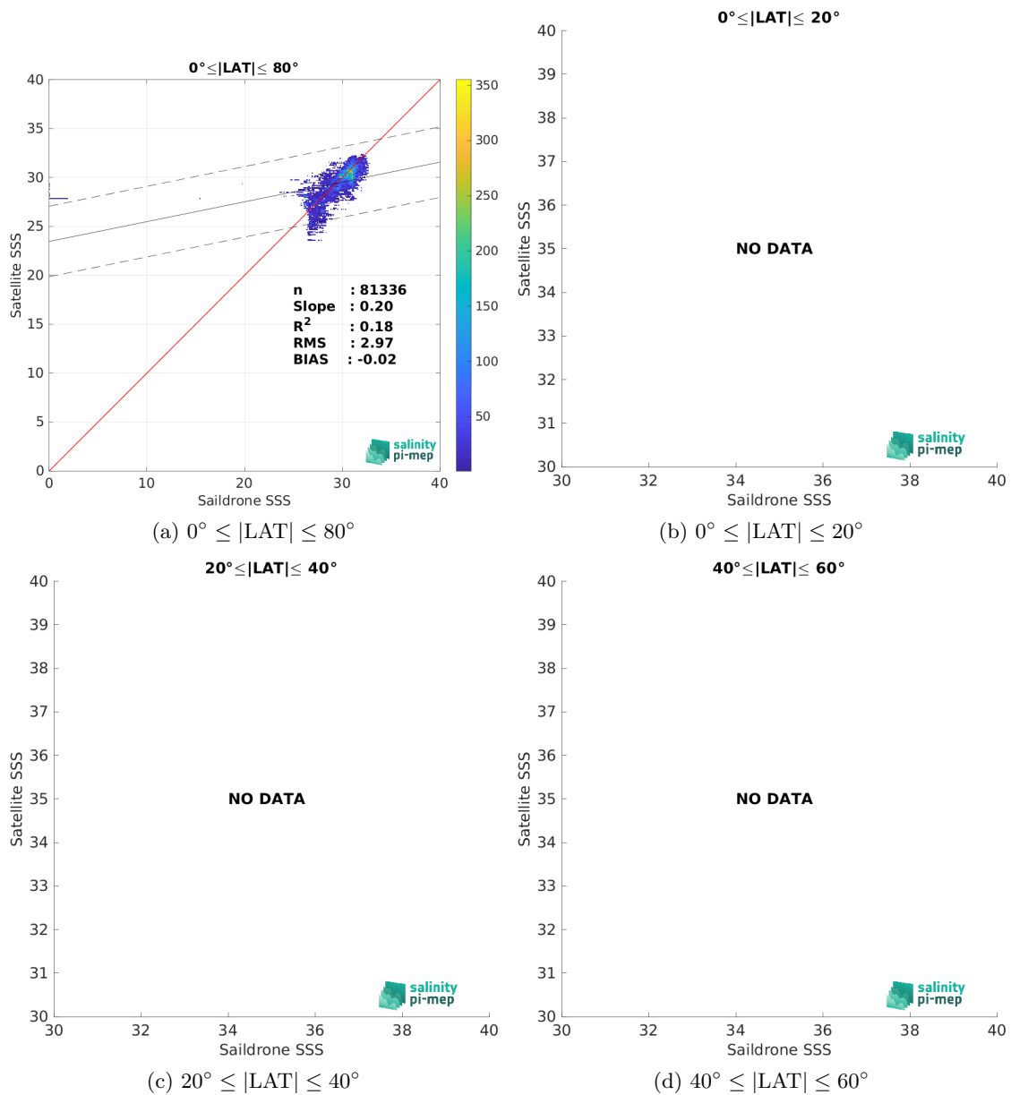
Figure 10: Contour maps of the concentration of CCI SSS L4 Merged-OI v4.41 - 7-day running (ESA) SSS (y-axis) versus Sailldrone SSS (x-axis) at match-up pairs for different latitude bands. For each plot, the red line shows x=y . The black thin and dashed lines indicate a linear fit through the data cloud and the \pm 95\% confidence levels, respectively. The number match-up pairs n , the slope and R^2 coefficient of the linear fit, the root mean square (RMS) and the mean bias between satellite and in situ data are indicated for each latitude band in each plots.
