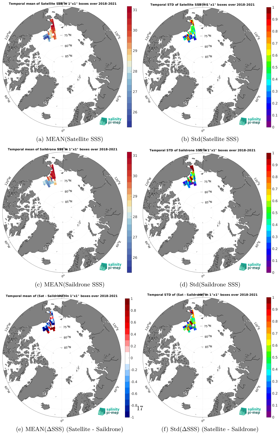
Figure 7: Temporal mean (left) and Std (right) of SSS from CCI SSS L4 Merged-OI v4.41 - 7-day running (ESA) (top), Saildrone (middle), and of \Delta SSS (Satellite - Saildrone). Only match-up pairs are used to generate these maps.
