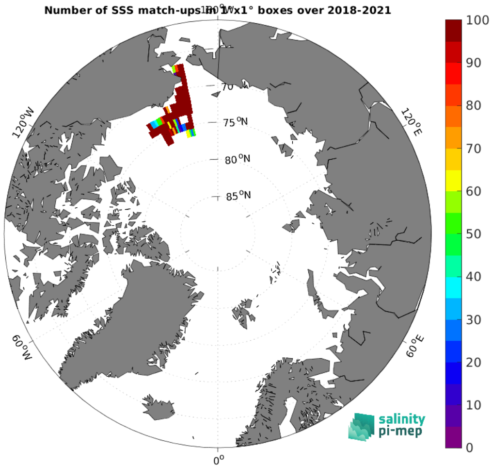
Figure 5: Number of SSS match-ups between Saildrone SSS and the CCI SSS L4 Merged-OI v4.41 - 7-day running (ESA) SSS product for the Arctic Ocean Pi-MEP region over 1^\circ \times 1^\circ boxes and for the full satellite product period.
