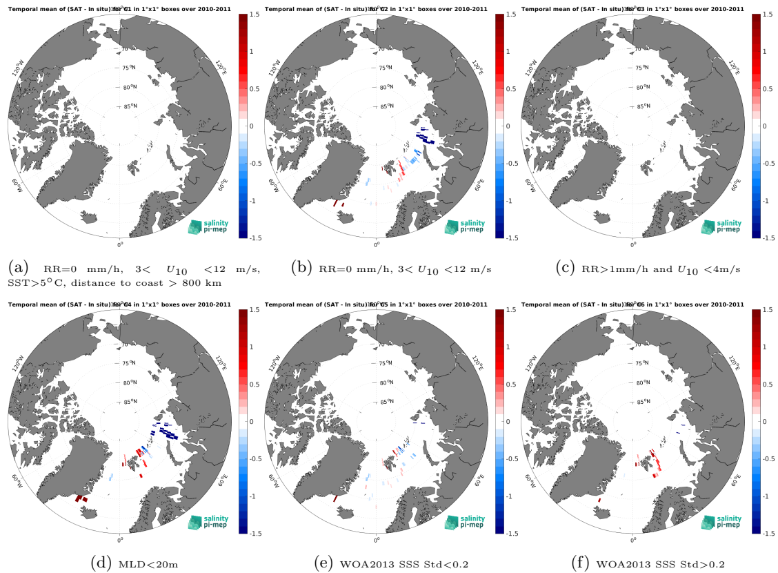
Figure 14: Temporal mean gridded over spatial boxes of size 1^\circ \times 1^\circ of \Delta SSS (CCI SSS L4 Merged-OI v4.41 - 7-day running (ESA) - Marine mammals) for 6 different subdatasets corresponding to:RR=0 mm/h, 3 < U_{10} < 12 m/s, SST >5^\circ C, distance to coast > 800 km (a), RR=0 mm/h, 3 < U_{10} < 12 m/s (b), RR >1 mm/h and U_{10} < 4 m/s (c),MLD <20 m (d),WOA2013 SSS Std <0.2 (e),WOA2013 SSS Std >0.2 (f).
