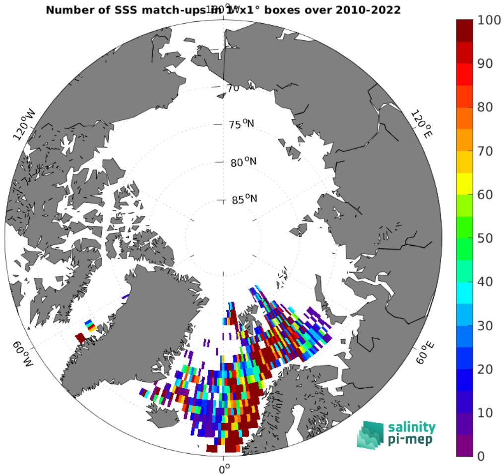
Figure 5: Number of SSS match-ups between ICES SSS and the CCI SSS L4 Merged-OI v4.41 - 7-day running (ESA) SSS product for the Arctic Ocean Pi-MEP region over 1^\circ \times 1^\circ boxes and for the full satellite product period.
