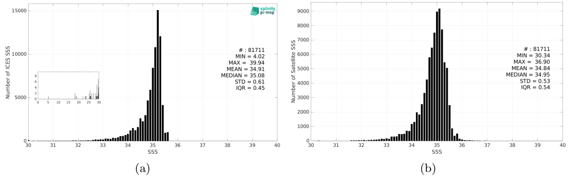
Figure 3: Histograms of SSS from ICES (a) and CCI SSS L4 Merged-OI v4.41 - 7-day running (ESA) (b) considering all match-up pairs per bins of 0.1 over the Arctic Ocean Pi-MEP region and for the full satellite product period.
