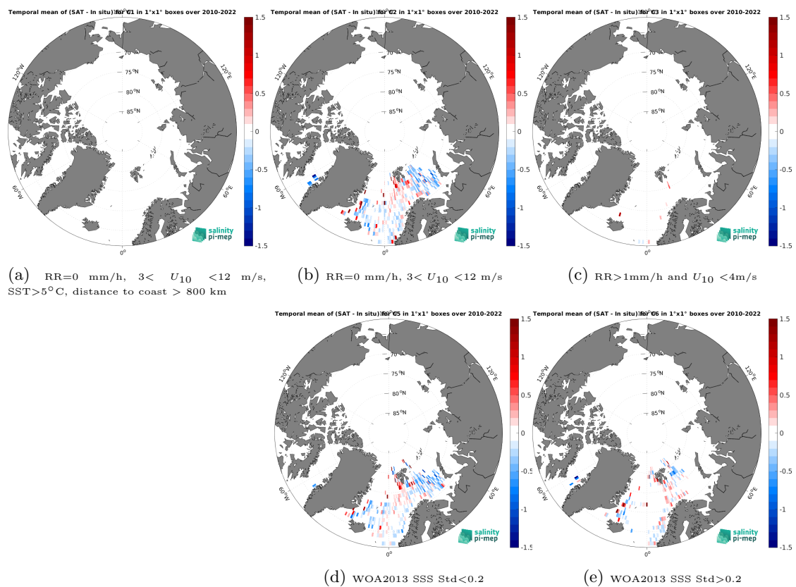
Figure 14: Temporal mean gridded over spatial boxes of size 1^\circ \times 1^\circ of \Delta SSS (CCI SSS L4 Merged-OI v4.41 - 7-day running (ESA) - ICES) for 5 different subdatasets corresponding to:RR=0 mm/h, 3 < U_{10} < 12 m/s, SST > 5^\circ C, distance to coast > 800 km (a), RR=0 mm/h, 3 < U_{10} < 12 m/s (b), RR > 1 mm/h and U_{10} < 4 m/s (c), WOA2013 SSS Std < 0.2 (d), WOA2013 SSS Std > 0.2 (e).
