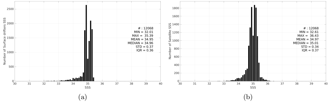
Figure 3: Histograms of SSS from Surface drifters (a) and CCI SSS L4 Merged-OI v4.41 - 7-day running (ESA) (b) considering all match-up pairs per bins of 0.1 over the Arctic Ocean Pi-MEP region and for the full satellite product period.
