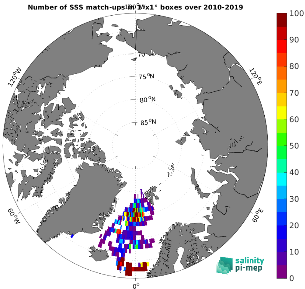
Figure 4: Number of SSS match-ups between Surface drifters SSS and the CCI SSS L4 Merged-OI v4.41 - 7-day running (ESA) SSS product for the Arctic Ocean Pi-MEP region over 1^\circ \times 1^\circ boxes and for the full satellite product period.
