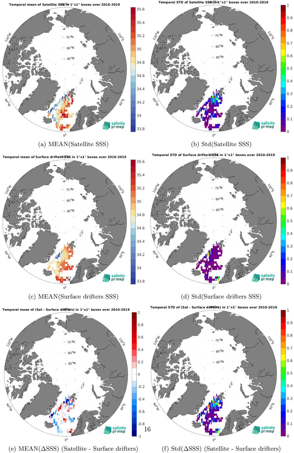
Figure 6: Temporal mean (left) and Std (right) of SSS from CCI SSS L4 Merged-OI v4.41 - 7-day running (ESA) (top), Surface drifters (middle), and of \Delta SSS (Satellite - Surface drifters). Only match-up pairs are used to generate these maps.
