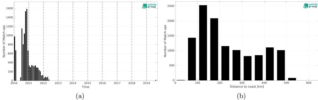
Figure 2: Number of match-ups between Surface drifters and CCI SSS L4 Merged-OI v4.41 - 7-day running (ESA) SSS as a function of time (a) and as function of the distance to coast (b) over the Arctic Ocean Pi-MEP region and for the full satellite product period.
