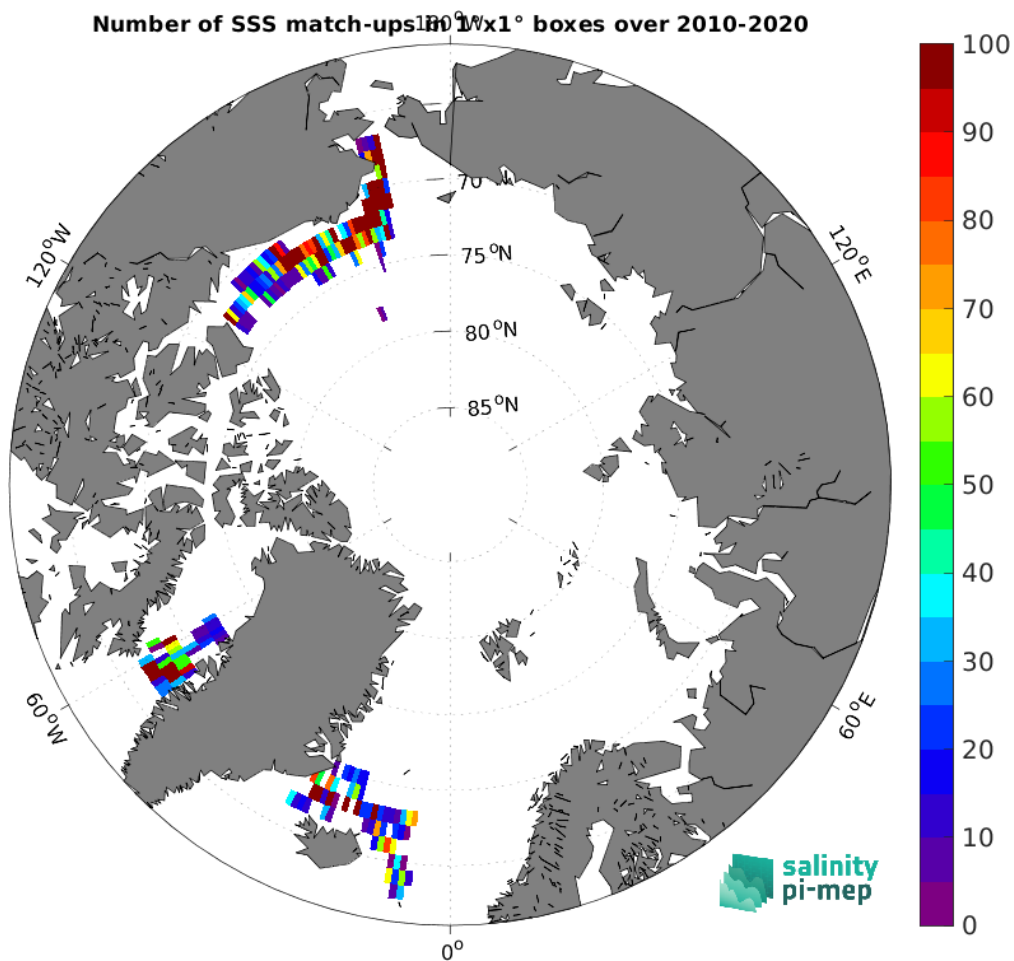
Figure 5: Number of SSS match-ups between TSG (SAMOS) SSS and the CCI SSS L4 Merged-OI v4.41 - 30-day running (ESA) SSS product for the Arctic Ocean Pi-MEP region over 1^\circ \times 1^\circ boxes and for the full satellite product period.
