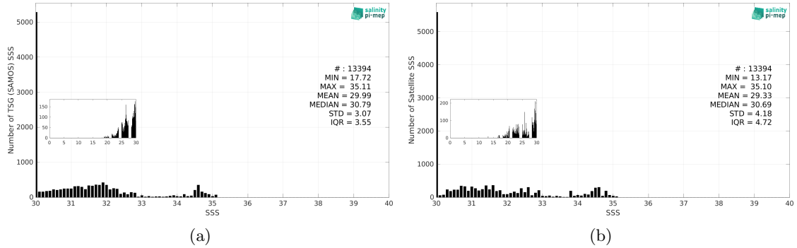
Figure 3: Histograms of SSS from TSG (SAMOS) (a) and CCI SSS L4 Merged-OI v4.41 - 30-day running (ESA) (b) considering all match-up pairs per bins of 0.1 over the Arctic Ocean Pi-MEP region and for the full satellite product period.
