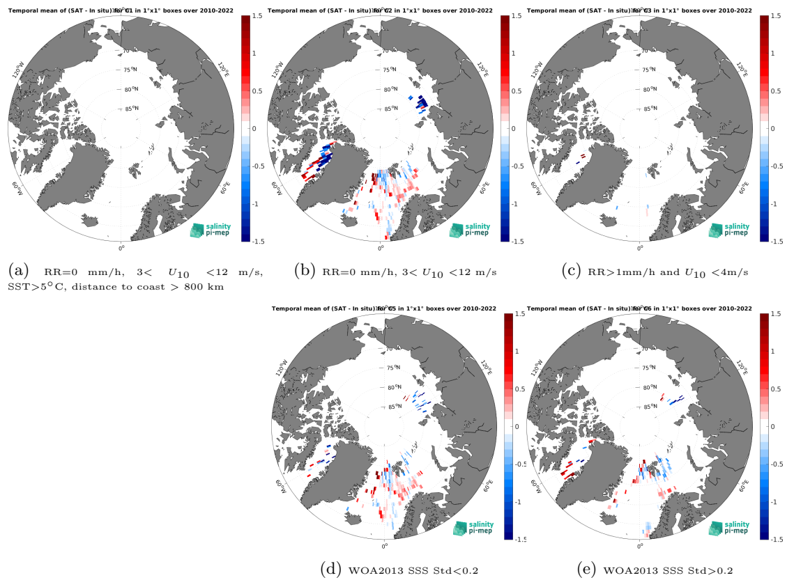
Figure 14: Temporal mean gridded over spatial boxes of size 1^\circ \times 1^\circ of \Delta SSS (CCI SSS L4 Merged-OI v4.41 - 30-day running (ESA) - TSG (Polarstern)) for 5 different subdatasets corresponding to:RR=0 mm/h, 3 < U_{10} < 12 m/s, SST >5^\circ C, distance to coast > 800 km (a), RR=0 mm/h, 3 < U_{10} < 12 m/s (b), RR >1 mm/h and U_{10} < 4 m/s (c), WOA2013 SSS Std <0.2 (d), WOA2013 SSS Std >0.2 (e).
