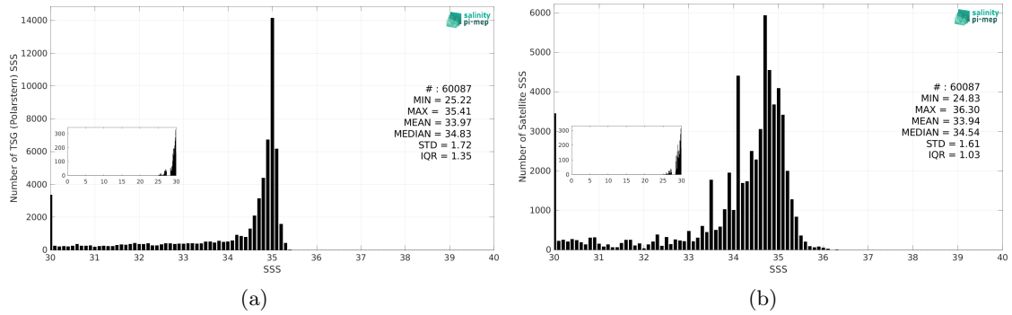
Figure 3: Histograms of SSS from TSG (Polarstern) (a) and CCI SSS L4 Merged-OI v4.41 - 30-day running (ESA) (b) considering all match-up pairs per bins of 0.1 over the Arctic Ocean Pi-MEP region and for the full satellite product period.
