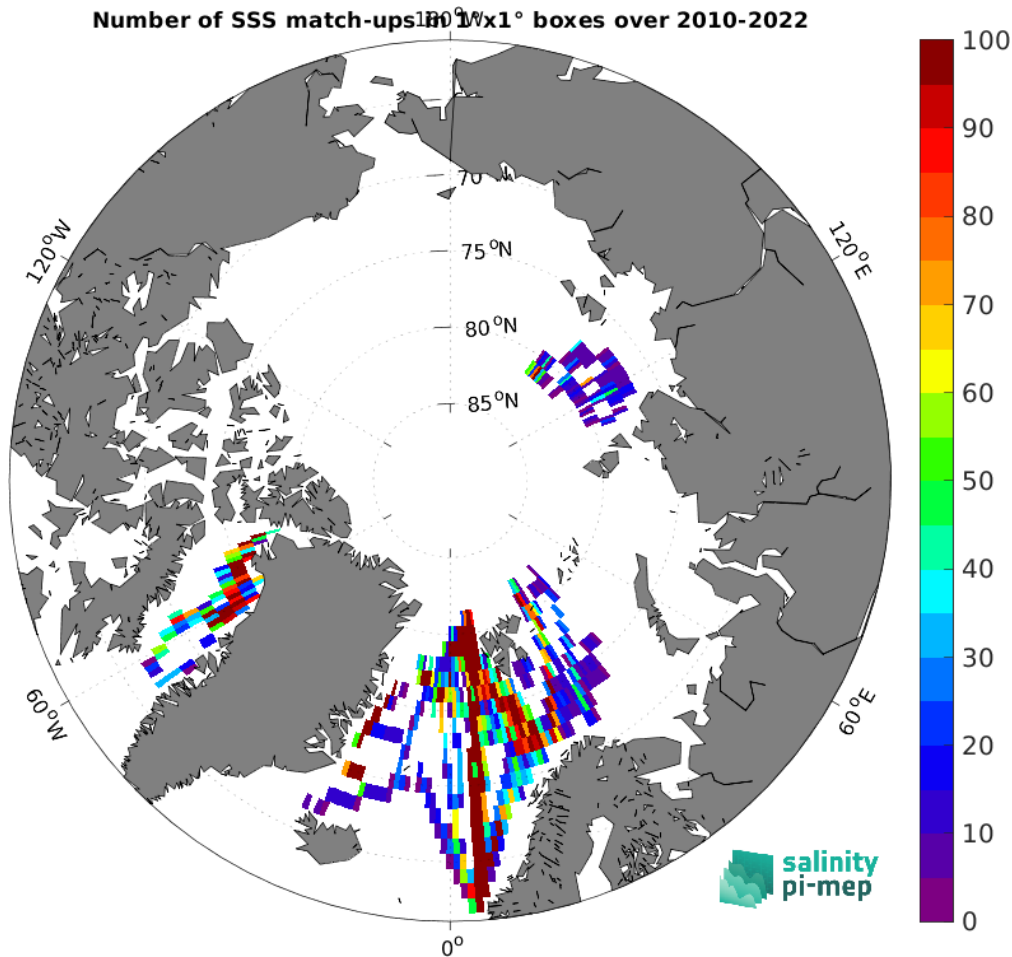
Figure 5: Number of SSS match-ups between TSG (Polarstern) SSS and the CCI SSS L4 Merged-OI v4.41 - 30-day running (ESA) SSS product for the Arctic Ocean Pi-MEP region over 1^\circ \times 1^\circ boxes and for the full satellite product period.
