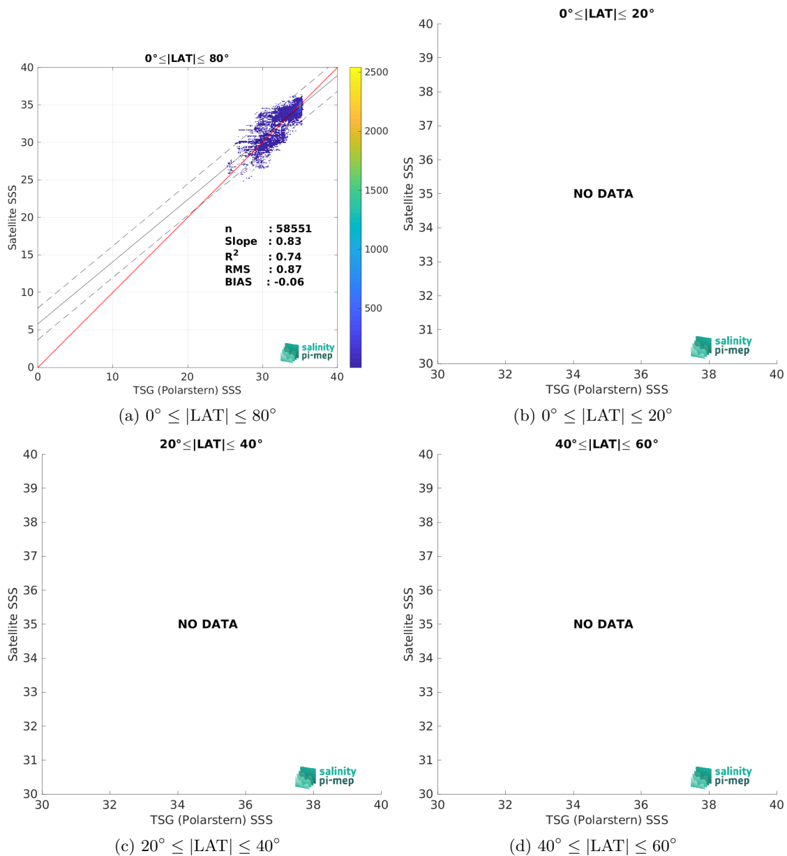
Figure 10: Contour maps of the concentration of CCI SSS L4 Merged-OI v4.41 - 30-day running (ESA) SSS (y-axis) versus TSG (Polarstern) SSS (x-axis) at match-up pairs for different latitude bands. For each plot, the red line shows x=y . The black thin and dashed lines indicate a linear fit through the data cloud and the \pm 95\% confidence levels, respectively. The number match-up pairs n , the slope and R^2 coefficient of the linear fit, the root mean square (RMS) and the mean bias between satellite and in situ data are indicated for each latitude band in each plots.
