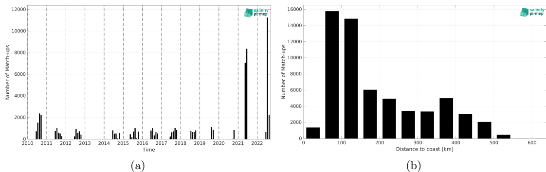
Figure 2: Number of match-ups between TSG (Polarstern) and CCI SSS L4 Merged-OI v4.41 - 30-day running (ESA) SSS as a function of time (a) and as function of the distance to coast (b) over the Arctic Ocean Pi-MEP region and for the full satellite product period.
