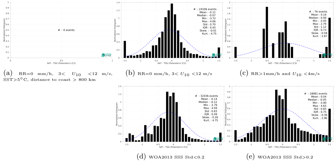
Figure 15: Normalized histogram of \Delta SSS (CCI SSS L4 Merged-OI v4.41 - 30-day running (ESA) - TSG (Polarstern)) for 5 different subdatasets corresponding to: RR=0 mm/h, 3 < U_{10} < 12 m/s, SST > 5°C, distance to coast > 800 km (a), RR=0 mm/h, 3 < U_{10} < 12 m/s (b), RR > 1mm/h and U_{10} < 4 m/s (c), WOA2013 SSS Std < 0.2 (d), WOA2013 SSS Std > 0.2 (e).
