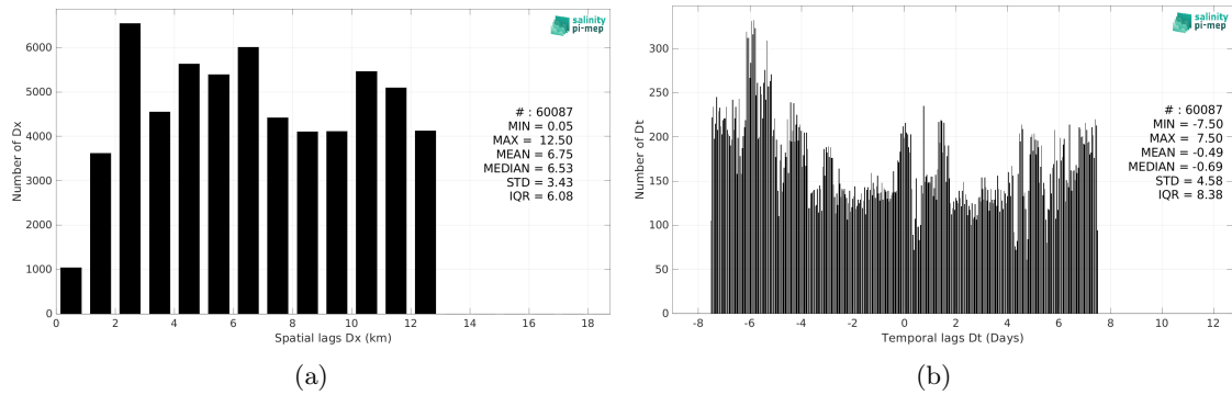
Figure 6: Histograms of the spatial (a) and temporal (b) lags between the location/time of the TSG (Polarstern) measurement and the date of the corresponding CCI SSS L4 Merged-OI v4.41 - 30-day running (ESA) SSS pixel.
