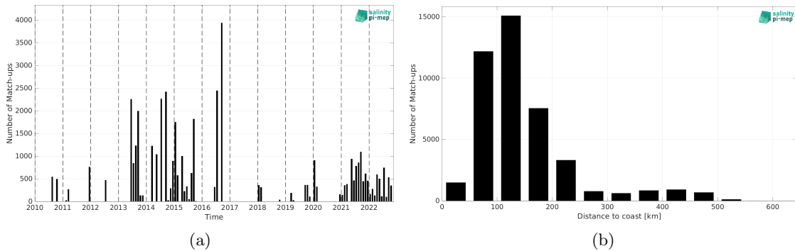
Figure 2: Number of match-ups between TSG (LEGOS-DM) and CCI SSS L4 Merged-OI v4.41 - 30-day running (ESA) SSS as a function of time (a) and as function of the distance to coast (b) over the Arctic Ocean Pi-MEP region and for the full satellite product period.
