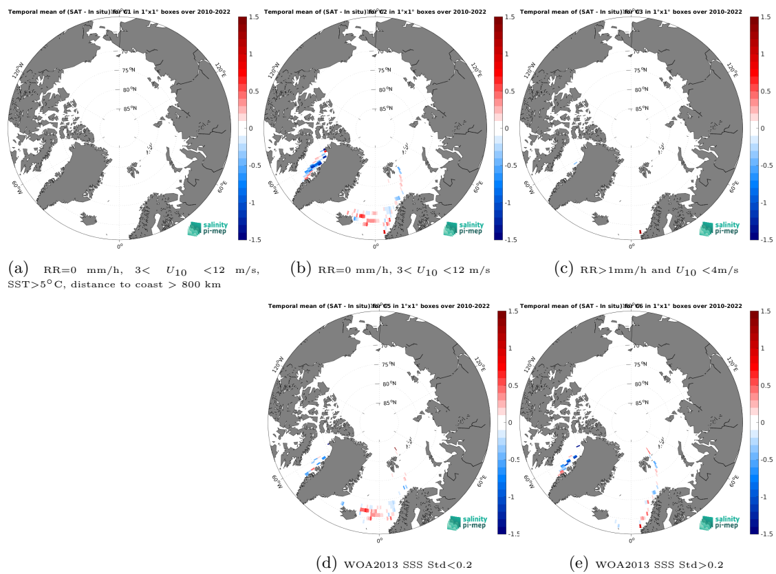
Figure 14: Temporal mean gridded over spatial boxes of size 1^\circ \times 1^\circ of \Delta\text{SSS} (CCI SSS L4 Merged-OI v4.41 - 30-day running (ESA) - TSG (LEGOS-DM)) for 5 different subdatasets corresponding to: RR=0 mm/h, 3 < U_{10} < 12 m/s, SST > 5^\circ\text{C} , distance to coast > 800 km (a), RR=0 mm/h, 3 < U_{10} < 12 m/s (b), RR > 1 mm/h and U_{10} < 4 m/s (c), WOA2013 SSS Std < 0.2 (d), WOA2013 SSS Std > 0.2 (e).
