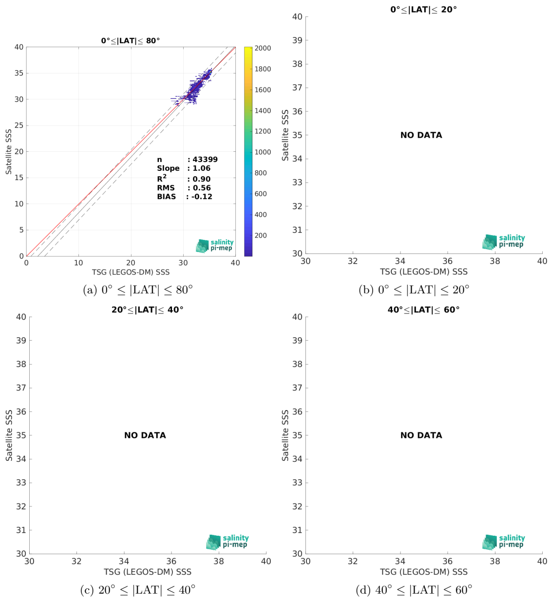
Figure 10: Contour maps of the concentration of CCI SSS L4 Merged-OI v4.41 - 30-day running (ESA) SSS (y-axis) versus TSG (LEGOS-DM) SSS (x-axis) at match-up pairs for different latitude bands. For each plot, the red line shows x=y . The black thin and dashed lines indicate a linear fit through the data cloud and the \pm 95\% confidence levels, respectively. The number match-up pairs n , the slope and R^2 coefficient of the linear fit, the root mean square (RMS) and the mean bias between satellite and in situ data are indicated for each latitude band in each plots.
