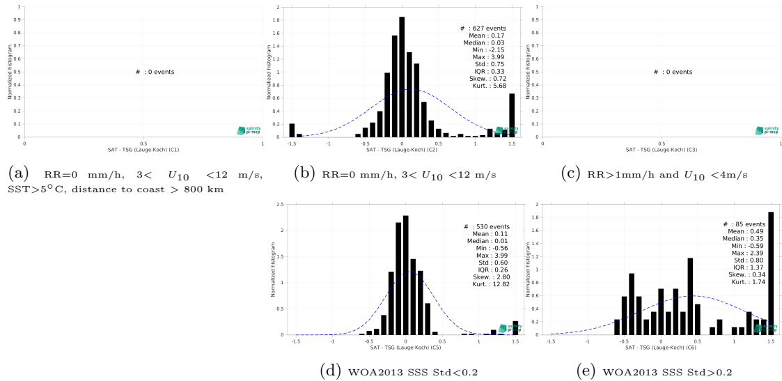
Figure 15: Normalized histogram of \Delta SSS (CCI SSS L4 Merged-OI v4.41 - 30-day running (ESA) - TSG (Lauge-Koch)) for 5 different subdatasets corresponding to: RR=0 mm/h, 3 < U_{10} < 12 m/s, SST>5°C, distance to coast > 800 km (a), RR=0 mm/h, 3 < U_{10} < 12 m/s (b), RR>1mm/h and U_{10} < 4 m/s (c), WOA2013 SSS Std<0.2 (d), WOA2013 SSS Std>0.2 (e).
