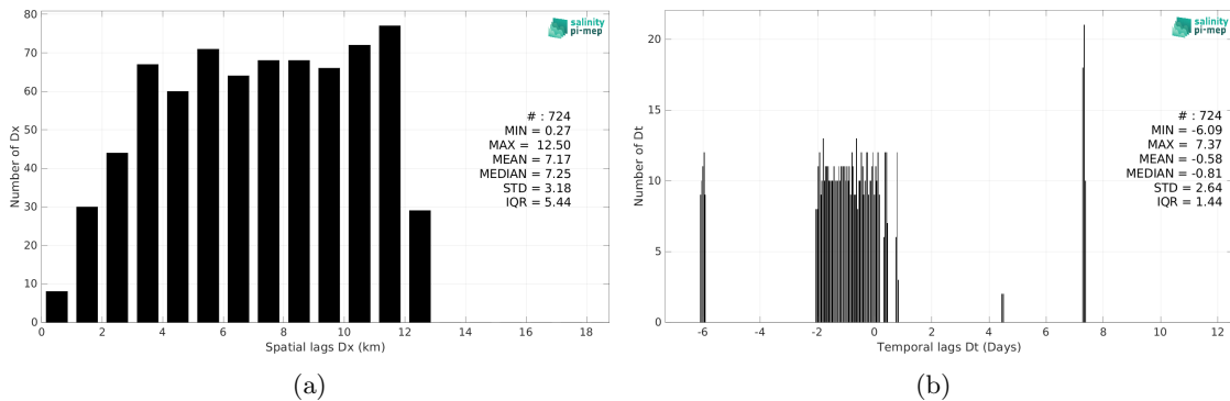
Figure 6: Histograms of the spatial (a) and temporal (b) lags between the location/time of the TSG (Lauge-Koch) measurement and the date of the corresponding CCI SSS L4 Merged-OI v4.41 - 30-day running (ESA) SSS pixel.
