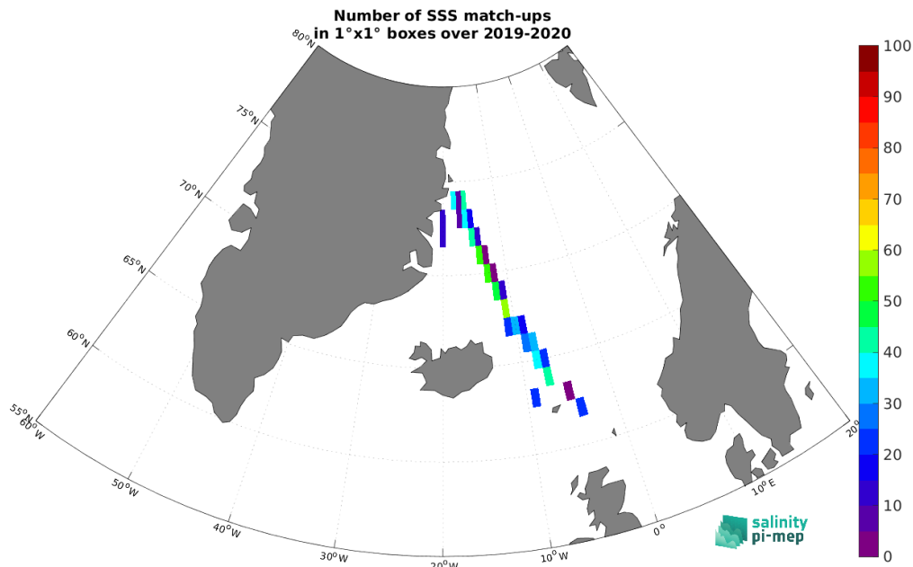
Figure 5: Number of SSS match-ups between TSG (Lauge-Koch) SSS and the CCI SSS L4 Merged-OI v4.41 - 30-day running (ESA) SSS product for the Arctic Ocean Pi-MEP region over 1^\circ \times 1^\circ boxes and for the full satellite product period.
