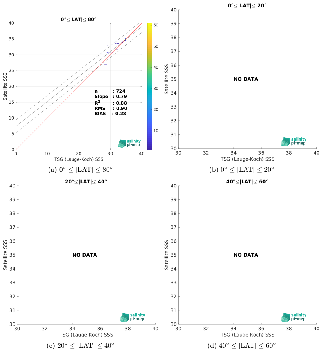
Figure 10: Contour maps of the concentration of CCI SSS L4 Merged-OI v4.41 - 30-day running (ESA) SSS (y-axis) versus TSG (Lauge-Koch) SSS (x-axis) at match-up pairs for different latitude bands. For each plot, the red line shows x=y . The black thin and dashed lines indicate a linear fit through the data cloud and the \pm 95\% confidence levels, respectively. The number match-up pairs n , the slope and R^2 coefficient of the linear fit, the root mean square (RMS) and the mean bias between satellite and in situ data are indicated for each latitude band in each plots.
