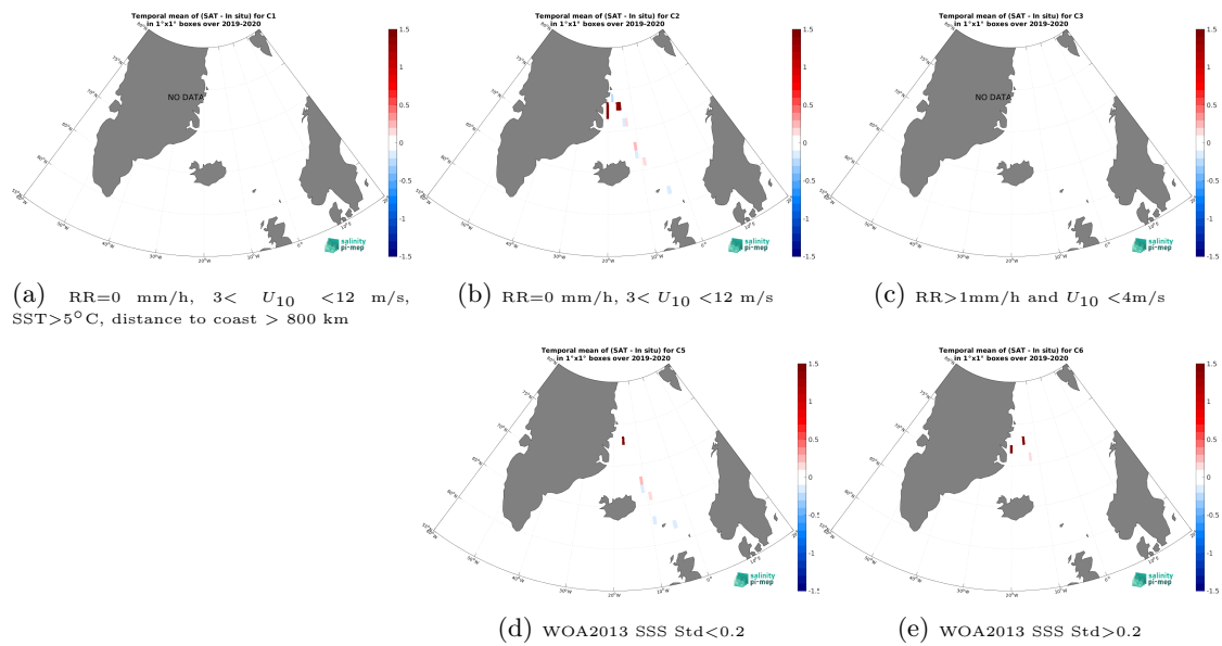
Figure 14: Temporal mean gridded over spatial boxes of size 1^\circ \times 1^\circ of \Delta SSS (CCI SSS L4 Merged-OI v4.41 - 30-day running (ESA) - TSG (Lauge-Koch)) for 5 different subdatasets corresponding to:RR=0 mm/h, 3 < U_{10} < 12 m/s, SST > 5^\circ C, distance to coast > 800 km (a), RR=0 mm/h, 3 < U_{10} < 12 m/s (b), RR > 1 mm/h and U_{10} < 4 m/s (c), WOA2013 SSS Std < 0.2 (d), WOA2013 SSS Std > 0.2 (e).
