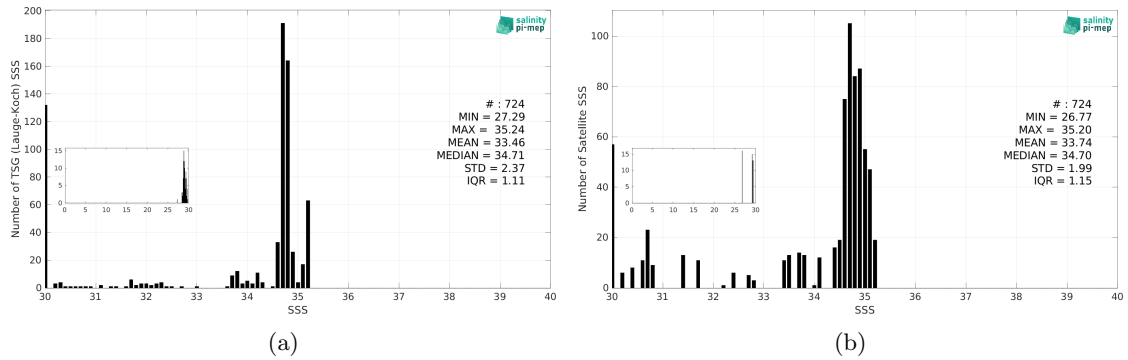
Figure 3: Histograms of SSS from TSG (Lauge-Koch) (a) and CCI SSS L4 Merged-OI v4.41 - 30-day running (ESA) (b) considering all match-up pairs per bins of 0.1 over the Arctic Ocean Pi-MEP region and for the full satellite product period.
