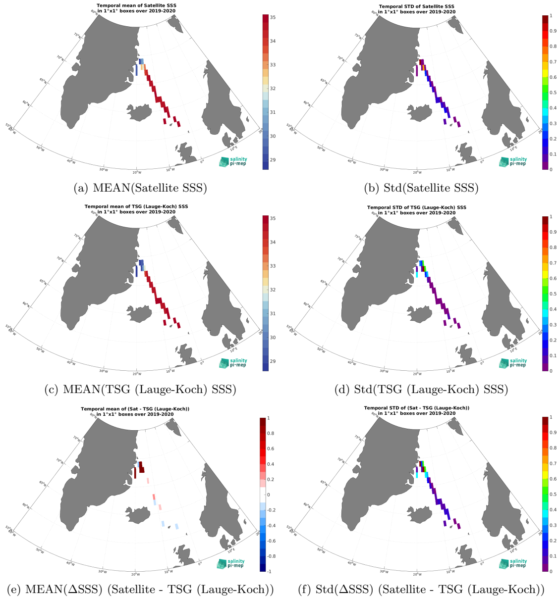
Figure 7: Temporal mean (left) and Std (right) of SSS from CCI SSS L4 Merged-OI v4.41 - 30-day running (ESA) (top), TSG (Lauge-Koch) (middle), and of \Delta SSS (Satellite - TSG (Lauge-Koch)). Only match-up pairs are used to generate these maps.
