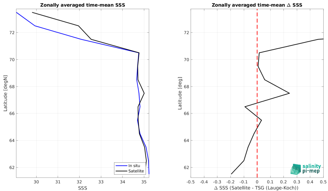
Figure 9: Left panel: Zonal mean SSS from CCI SSS L4 Merged-OI v4.41 - 30-day running (ESA) satellite product (black) and from TSG (Lauge-Koch) (blue). Right panel: Zonal mean of \Delta SSS (Satellite - TSG (Lauge-Koch)) for all the collected Pi-MEP match-up pairs estimated over the full satellite product period.
