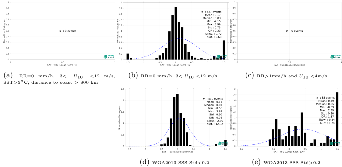
Figure 15: Normalized histogram of \Delta SSS (CCI SSS L4 Merged-OI v4.41 - 30-day running (ESA) - TSG (Lauge-Koch)) for 5 different subdatasets corresponding to: RR=0 mm/h, 3 < U_{10} < 12 m/s, SST > 5°C, distance to coast > 800 km (a), RR=0 mm/h, 3 < U_{10} < 12 m/s (b), RR > 1mm/h and U_{10} < 4 m/s (c), WOA2013 SSS Std < 0.2 (d), WOA2013 SSS Std > 0.2 (e).
