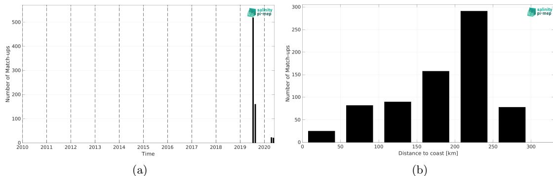
Figure 2: Number of match-ups between TSG (Lauge-Koch) and CCI SSS L4 Merged-OI v4.41 - 30-day running (ESA) SSS as a function of time (a) and as function of the distance to coast (b) over the Arctic Ocean Pi-MEP region and for the full satellite product period.
