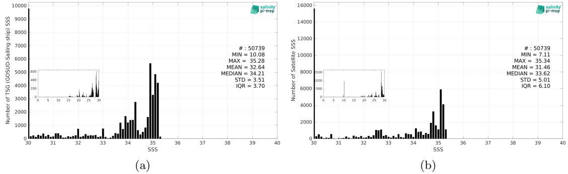
Figure 3: Histograms of SSS from TSG (GOSUD-Sailing-ship) (a) and CCI SSS L4 Merged-OI v4.41 - 30-day running (ESA) (b) considering all match-up pairs per bins of 0.1 over the Arctic Ocean Pi-MEP region and for the full satellite product period.
