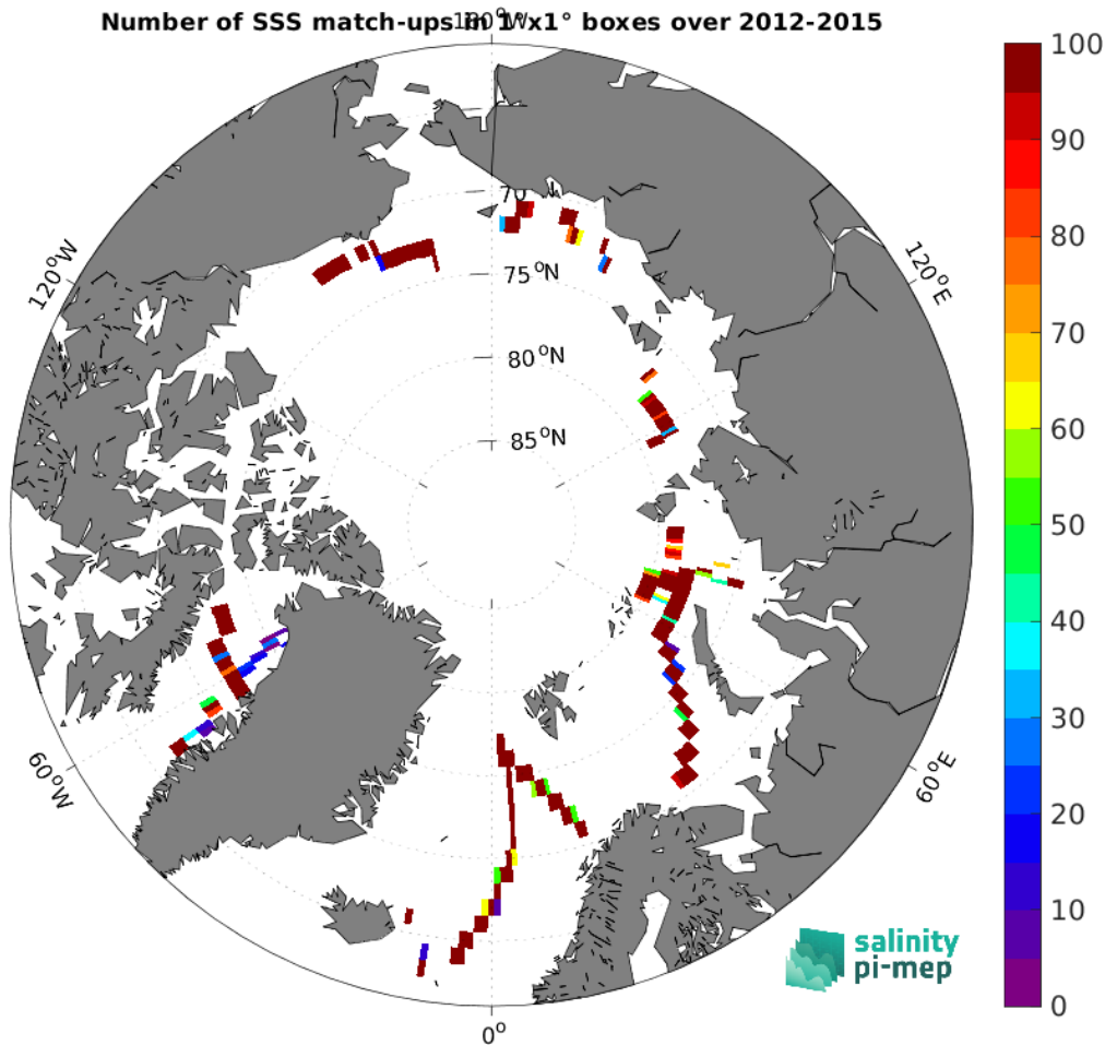
Figure 5: Number of SSS match-ups between TSG (GOSUD-Sailing-ship) SSS and the CCI SSS L4 Merged-OI v4.41 - 30-day running (ESA) SSS product for the Arctic Ocean Pi-MEP region over 1^\circ \times 1^\circ boxes and for the full satellite product period.
