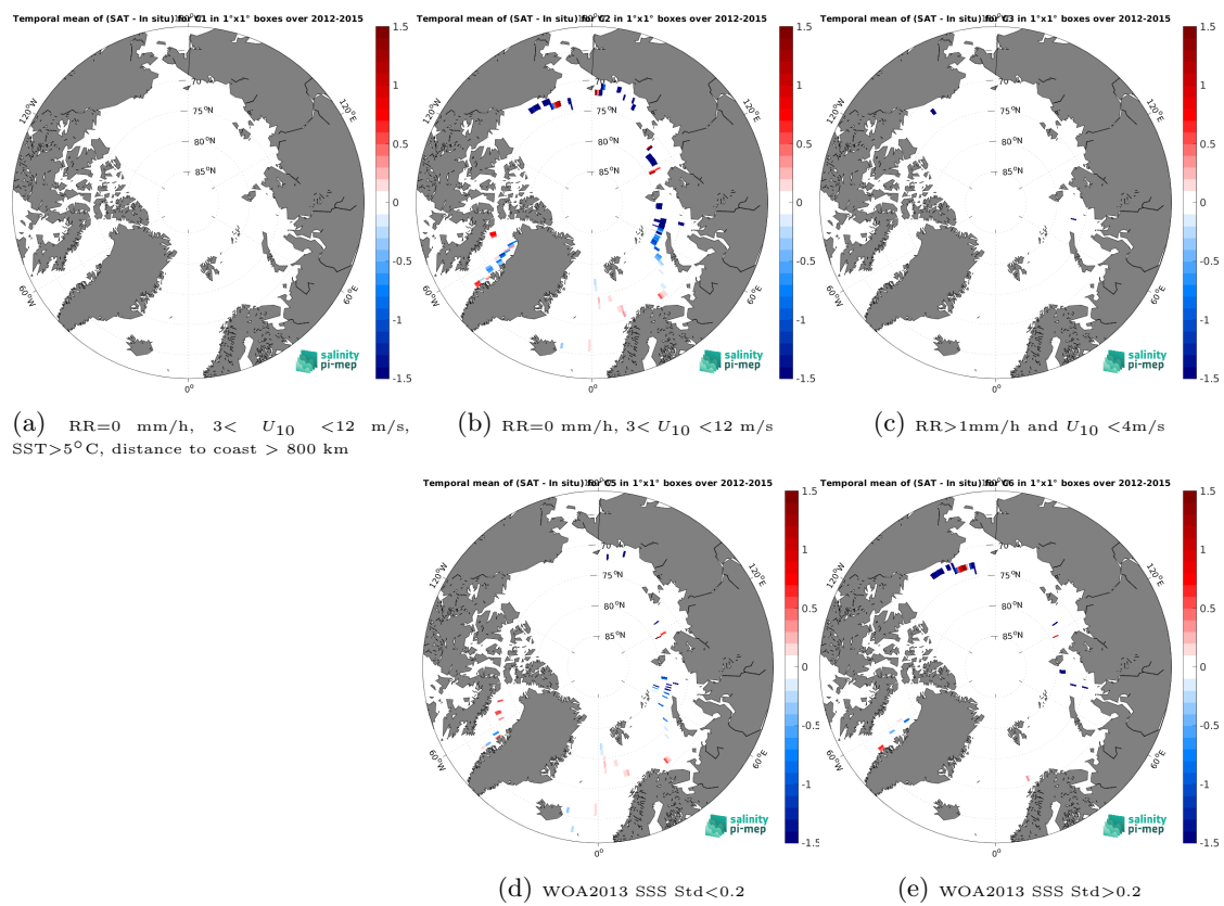
Figure 14: Temporal mean gridded over spatial boxes of size 1^\circ \times 1^\circ of \Delta SSS (CCI SSS L4 Merged-OI v4.41 - 30-day running (ESA) - TSG (GOSUD-Sailing-ship)) for 5 different subdatasets corresponding to: RR=0 mm/h, 3 < U_{10} < 12 m/s, SST > 5^\circ\text{C} , distance to coast > 800 km (a), RR=0 mm/h, 3 < U_{10} < 12 m/s (b), RR > 1 mm/h and U_{10} < 4 m/s (c), WOA2013 SSS Std < 0.2 (d), WOA2013 SSS Std > 0.2 (e).
