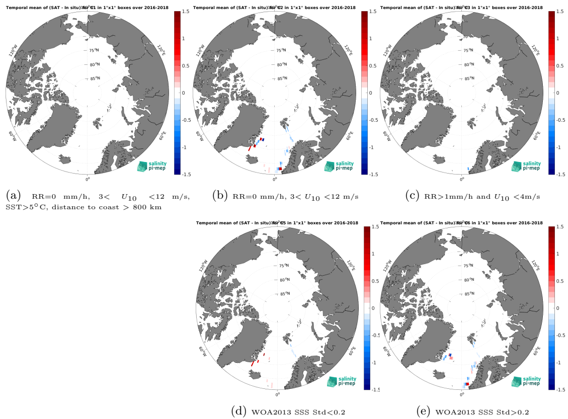
Figure 14: Temporal mean gridded over spatial boxes of size 1^\circ \times 1^\circ of \Delta\text{SSS} (CCI SSS L4 Merged-OI v4.41 - 30-day running (ESA) - TSG (GOSUD-Research-vessel)) for 5 different subdatasets corresponding to: RR=0 mm/h, 3 < U_{10} < 12 m/s, SST > 5°C, distance to coast > 800 km (a), RR=0 mm/h, 3 < U_{10} < 12 m/s (b), RR > 1mm/h and U_{10} < 4 m/s (c), WOA2013 SSS Std < 0.2 (d), WOA2013 SSS Std > 0.2 (e).
