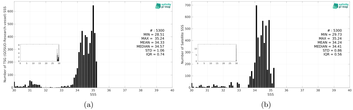
Figure 3: Histograms of SSS from TSG (GOSUD-Research-vessel) (a) and CCI SSS L4 Merged-OI v4.41 - 30-day running (ESA) (b) considering all match-up pairs per bins of 0.1 over the Arctic Ocean Pi-MEP region and for the full satellite product period.
