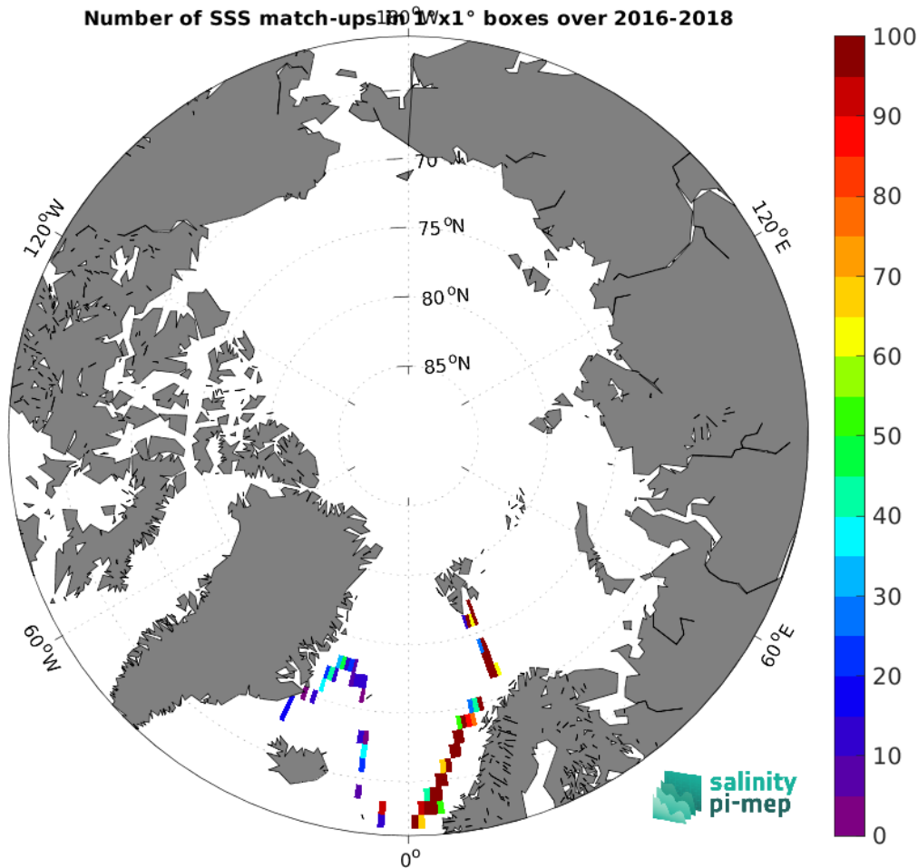
Figure 5: Number of SSS match-ups between TSG (GOSUD-Research-vessel) SSS and the CCI SSS L4 Merged-OI v4.41 - 30-day running (ESA) SSS product for the Arctic Ocean Pi-MEP region over 1^\circ \times 1^\circ boxes and for the full satellite product period.
