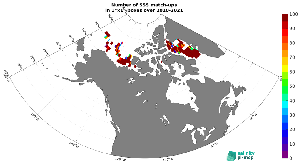
Figure 5: Number of SSS match-ups between TSG (Amundsen) SSS and the CCI SSS L4 Merged-OI v4.41 - 30-day running (ESA) SSS product for the Arctic Ocean Pi-MEP region over 1^\circ \times 1^\circ boxes and for the full satellite product period.
