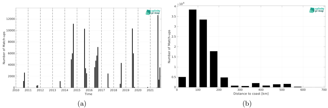
Figure 2: Number of match-ups between TSG (Amundsen) and CCI SSS L4 Merged-OI v4.41 - 30-day running (ESA) SSS as a function of time (a) and as function of the distance to coast (b) over the Arctic Ocean Pi-MEP region and for the full satellite product period.
