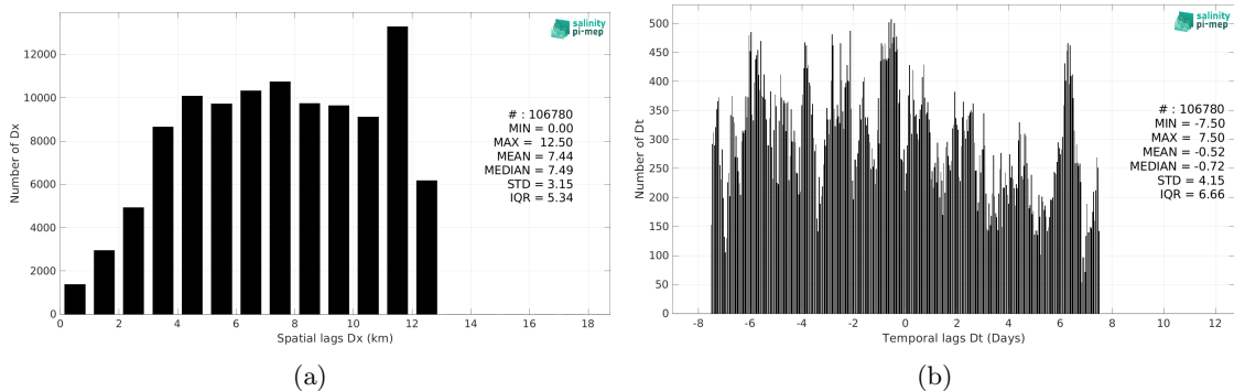
Figure 6: Histograms of the spatial (a) and temporal (b) lags between the location/time of the TSG (Amundsen) measurement and the date of the corresponding CCI SSS L4 Merged-OI v4.41 - 30-day running (ESA) SSS pixel.
