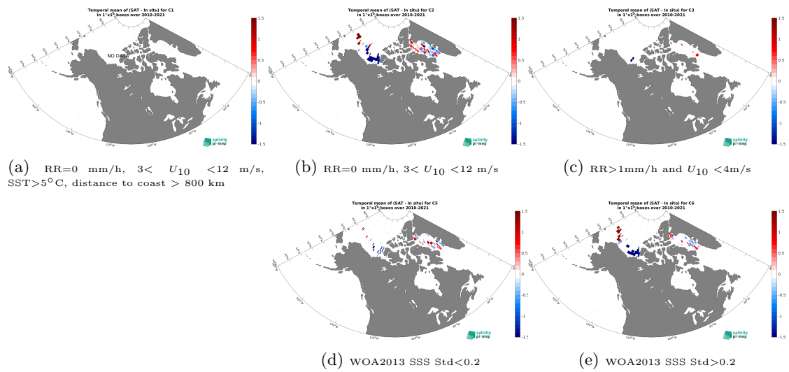
Figure 14: Temporal mean gridded over spatial boxes of size 1^\circ \times 1^\circ of \Delta\text{SSS} (CCI SSS L4 Merged-OI v4.41 - 30-day running (ESA) - TSG (Amundsen)) for 5 different subdatasets corresponding to: RR=0 mm/h, 3 < U_{10} < 12 m/s, SST > 5°C, distance to coast > 800 km (a), RR=0 mm/h, 3 < U_{10} < 12 m/s (b), RR > 1mm/h and U_{10} < 4 m/s (c), WOA2013 SSS Std < 0.2 (d), WOA2013 SSS Std > 0.2 (e).
