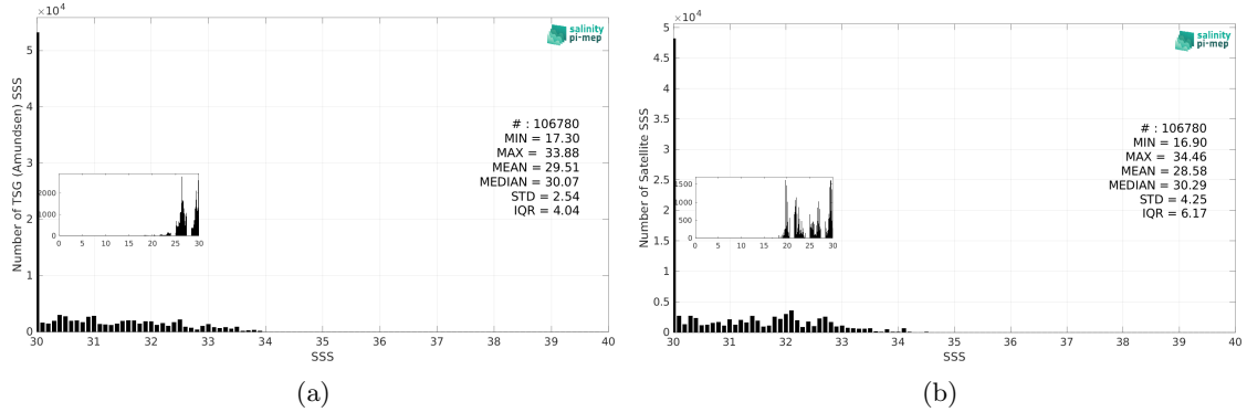
Figure 3: Histograms of SSS from TSG (Amundsen) (a) and CCI SSS L4 Merged-OI v4.41 - 30-day running (ESA) (b) considering all match-up pairs per bins of 0.1 over the Arctic Ocean Pi-MEP region and for the full satellite product period.
