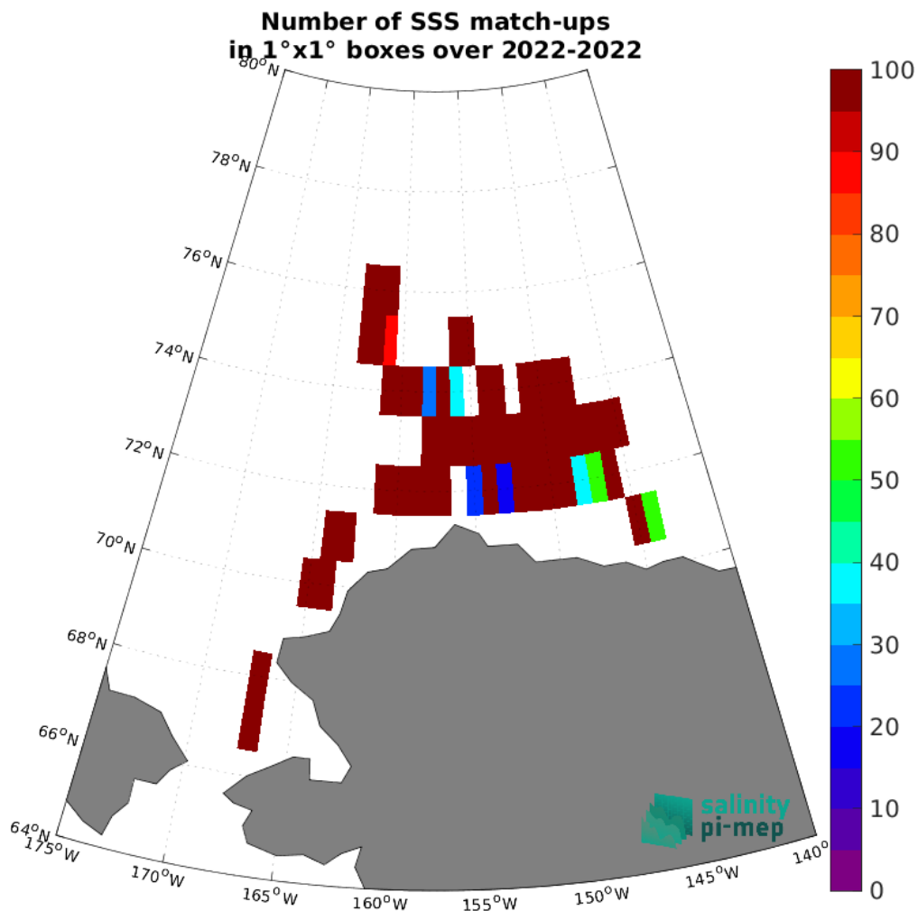
Figure 5: Number of SSS match-ups between SASSIE SSS and the CCI SSS L4 Merged-OI v4.41 - 30-day running (ESA) SSS product for the Arctic Ocean Pi-MEP region over 1^\circ \times 1^\circ boxes and for the full satellite product period.
