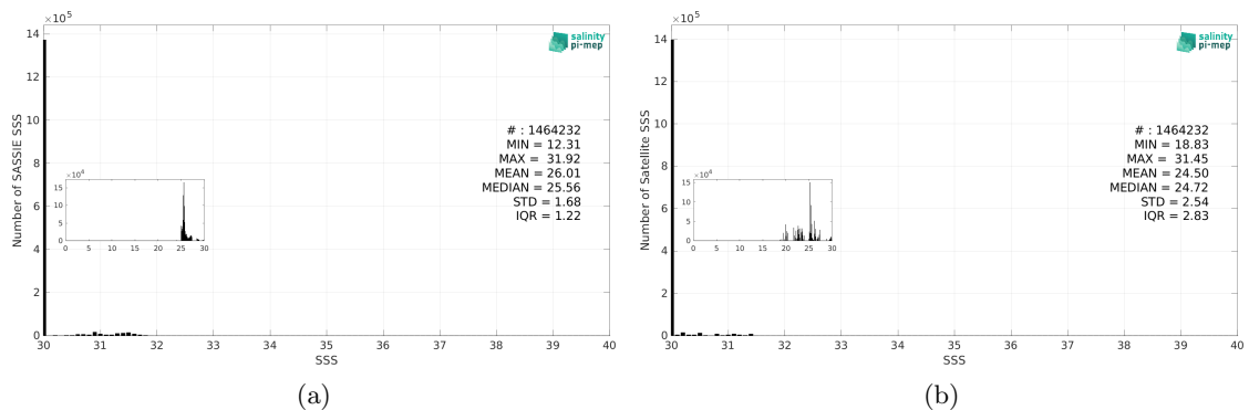
Figure 3: Histograms of SSS from SASSIE (a) and CCI SSS L4 Merged-OI v4.41 - 30-day running (ESA) (b) considering all match-up pairs per bins of 0.1 over the Arctic Ocean Pi-MEP region and for the full satellite product period.
