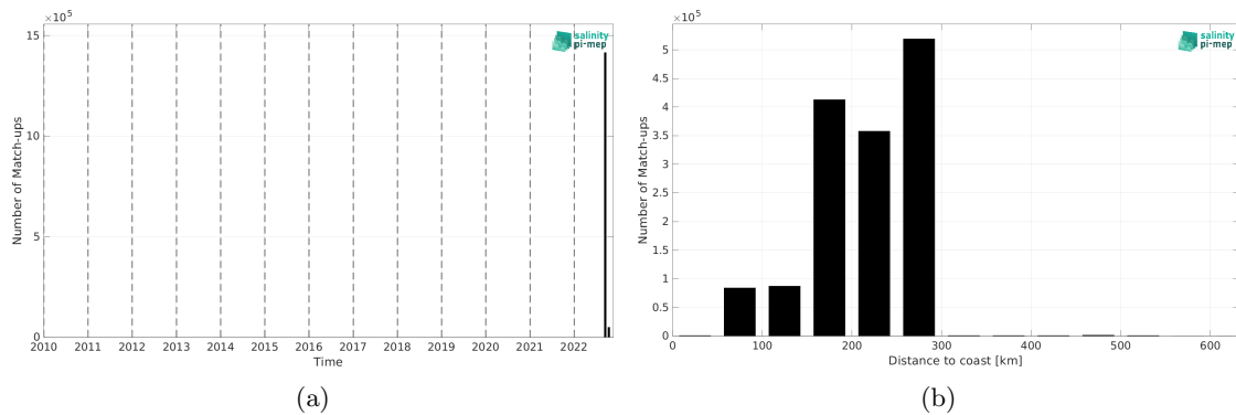
Figure 2: Number of match-ups between SASSIE and CCI SSS L4 Merged-OI v4.41 - 30-day running (ESA) SSS as a function of time (a) and as function of the distance to coast (b) over the Arctic Ocean Pi-MEP region and for the full satellite product period.
