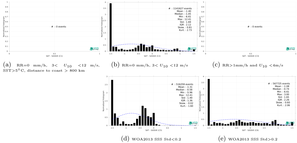
Figure 15: Normalized histogram of \Delta SSS (CCI SSS L4 Merged-OI v4.41 - 30-day running (ESA) - SASSIE) for 5 different subdatasets corresponding to: RR=0 mm/h, 3 < U_{10} < 12 m/s, SST > 5°C, distance to coast > 800 km (a), RR=0 mm/h, 3 < U_{10} < 12 m/s (b), RR > 1mm/h and U_{10} < 4 m/s (c), WOA2013 SSS Std < 0.2 (d), WOA2013 SSS Std > 0.2 (e).
