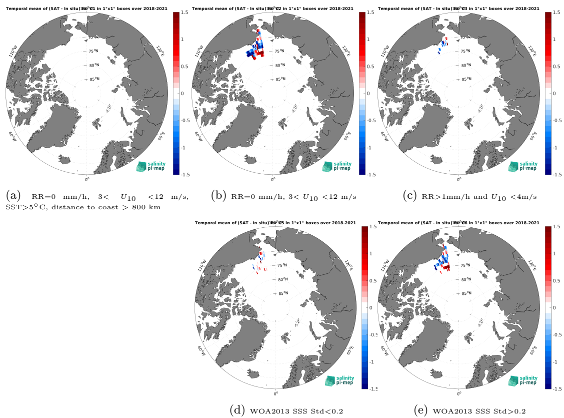
Figure 14: Temporal mean gridded over spatial boxes of size 1^\circ \times 1^\circ of \Delta SSS (CCI SSS L4 Merged-OI v4.41 - 30-day running (ESA) - Saildrone) for 5 different subdatasets corresponding to:RR=0 mm/h, 3 < U_{10} < 12 m/s, SST >5^\circ C, distance to coast > 800 km (a), RR=0 mm/h, 3 < U_{10} < 12 m/s (b), RR >1 mm/h and U_{10} < 4 m/s (c), WOA2013 SSS Std <0.2 (d), WOA2013 SSS Std >0.2 (e).
