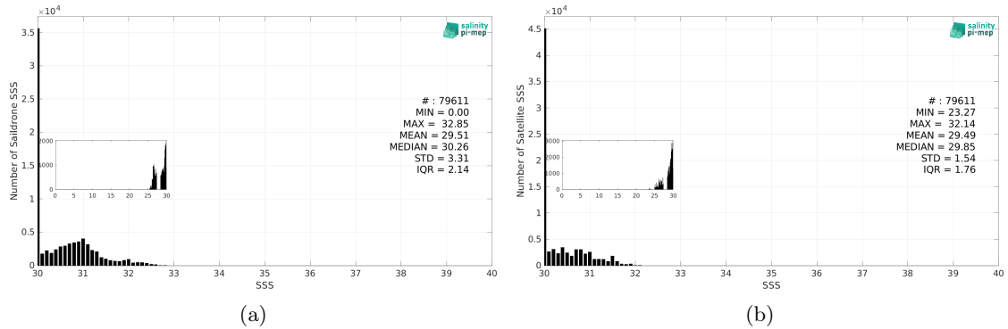
Figure 3: Histograms of SSS from Saildrone (a) and CCI SSS L4 Merged-OI v4.41 - 30-day running (ESA) (b) considering all match-up pairs per bins of 0.1 over the Arctic Ocean Pi-MEP region and for the full satellite product period.
