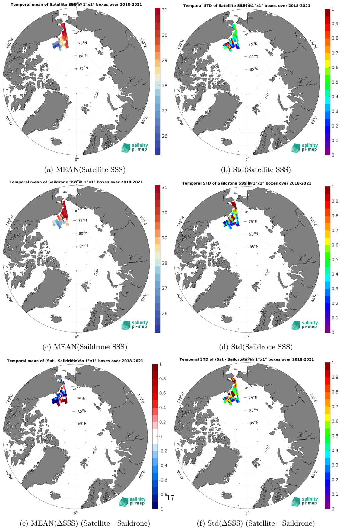
Figure 7: Temporal mean (left) and Std (right) of SSS from CCI SSS L4 Merged-OI v4.41 - 30-day running (ESA) (top), Saildrone (middle), and of \Delta SSS (Satellite - Saildrone). Only match-up pairs are used to generate these maps.
