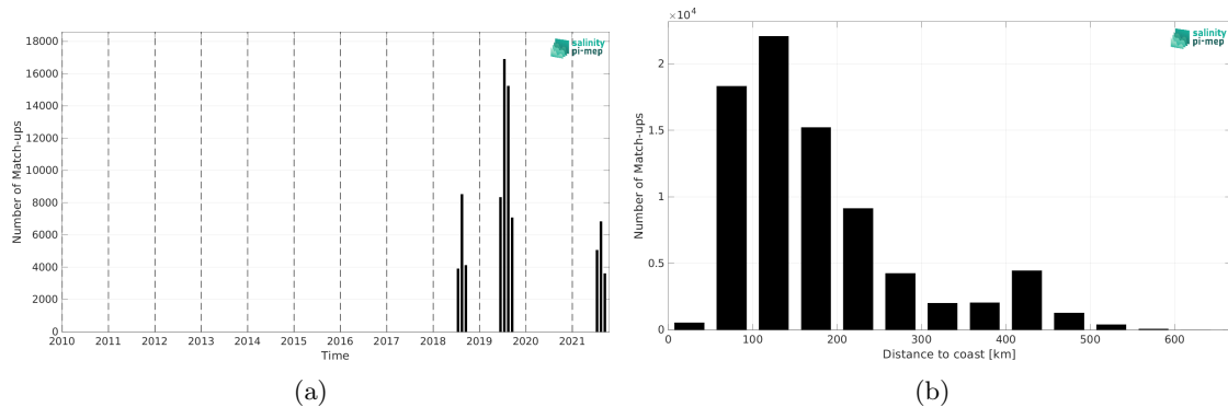
Figure 2: Number of match-ups between Saildrone and CCI SSS L4 Merged-OI v4.41 - 30-day running (ESA) SSS as a function of time (a) and as function of the distance to coast (b) over the Arctic Ocean Pi-MEP region and for the full satellite product period.
