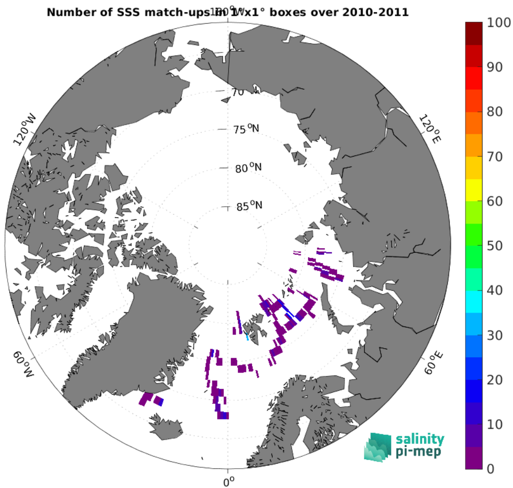
Figure 5: Number of SSS match-ups between Marine mammals SSS and the CCI SSS L4 Merged-OI v4.41 - 30-day running (ESA) SSS product for the Arctic Ocean Pi-MEP region over 1^{\circ} \times 1^{\circ} boxes and for the full satellite product period.
