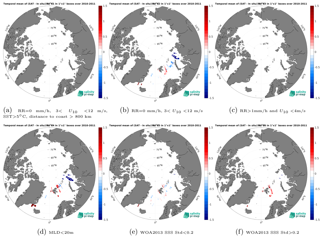
Figure 14: Temporal mean gridded over spatial boxes of size 1^\circ \times 1^\circ of \Delta SSS (CCI SSS L4 Merged-OI v4.41 - 30-day running (ESA) - Marine mammals) for 6 different subdatasets corresponding to:RR=0 mm/h, 3 < U_{10} < 12 m/s, SST>5°C, distance to coast > 800 km (a), RR=0 mm/h, 3 < U_{10} < 12 m/s (b), RR>1mm/h and U_{10} < 4 m/s (c),MLD<20m (d),WOA2013 SSS Std<0.2 (e),WOA2013 SSS Std>0.2 (f).
