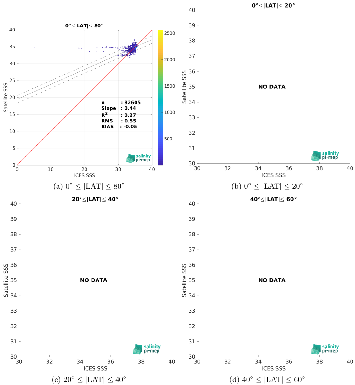
Figure 10: Contour maps of the concentration of CCI SSS L4 Merged-OI v4.41 - 30-day running (ESA) SSS (y-axis) versus ICES SSS (x-axis) at match-up pairs for different latitude bands. For each plot, the red line shows x=y . The black thin and dashed lines indicate a linear fit through the data cloud and the \pm 95\% confidence levels, respectively. The number match-up pairs n , the slope and R^2 coefficient of the linear fit, the root mean square (RMS) and the mean bias between satellite and in situ data are indicated for each latitude band in each plots.
