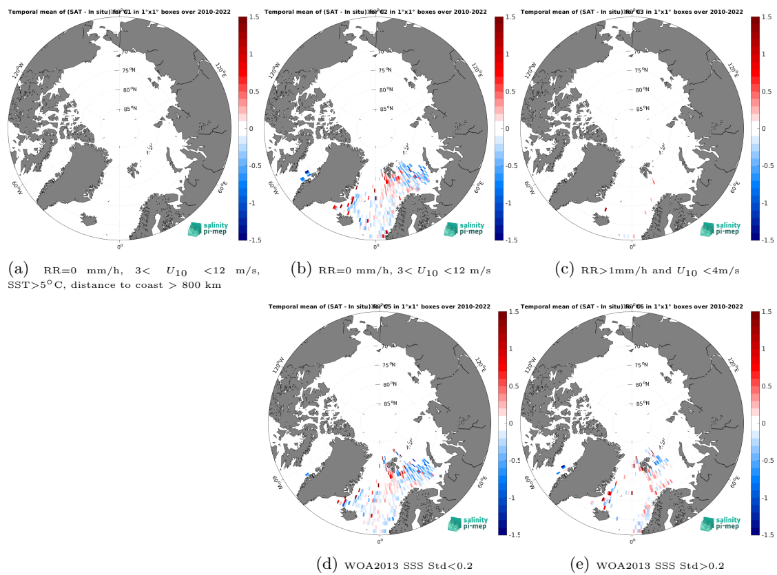
Figure 14: Temporal mean gridded over spatial boxes of size 1^\circ \times 1^\circ of \Delta SSS (CCI SSS L4 Merged-OI v4.41 - 30-day running (ESA) - ICES) for 5 different subdatasets corresponding to: RR=0 mm/h, 3 < U_{10} < 12 m/s, SST > 5^\circ\text{C} , distance to coast > 800 km (a), RR=0 mm/h, 3 < U_{10} < 12 m/s (b), RR > 1 mm/h and U_{10} < 4 m/s (c), WOA2013 SSS Std < 0.2 (d), WOA2013 SSS Std > 0.2 (e).
