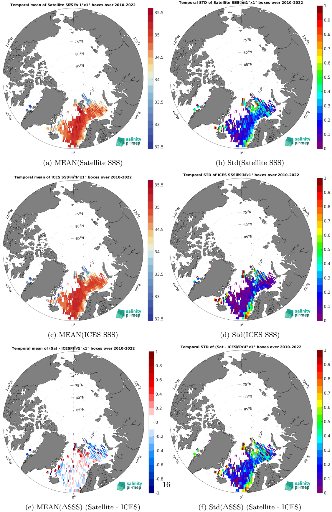
Figure 7: Temporal mean (left) and Std (right) of SSS from CCI SSS L4 Merged-OI v4.41 - 30-day running (ESA) (top), ICES (middle), and of \Delta SSS (Satellite - ICES). Only match-up pairs are used to generate these maps.
