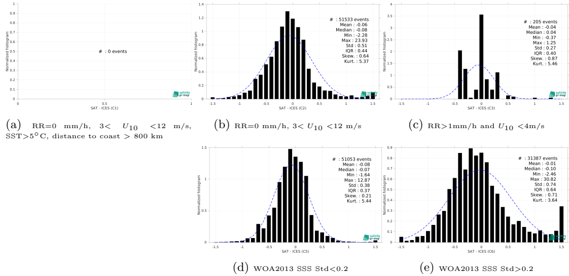
Figure 15: Normalized histogram of \Delta SSS (CCI SSS L4 Merged-OI v4.41 - 30-day running (ESA) - ICES) for 5 different subdatasets corresponding to: RR=0 mm/h, 3 < U_{10} < 12 m/s, SST>5°C, distance to coast > 800 km (a), RR=0 mm/h, 3 < U_{10} < 12 m/s (b), RR>1mm/h and U_{10} < 4 m/s (c), WOA2013 SSS Std<0.2 (d), WOA2013 SSS Std>0.2 (e).
