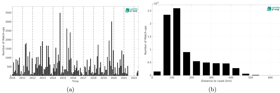
Figure 2: Number of match-ups between ICES and CCI SSS L4 Merged-OI v4.41 - 30-day running (ESA) SSS as a function of time (a) and as function of the distance to coast (b) over the Arctic Ocean Pi-MEP region and for the full satellite product period.
