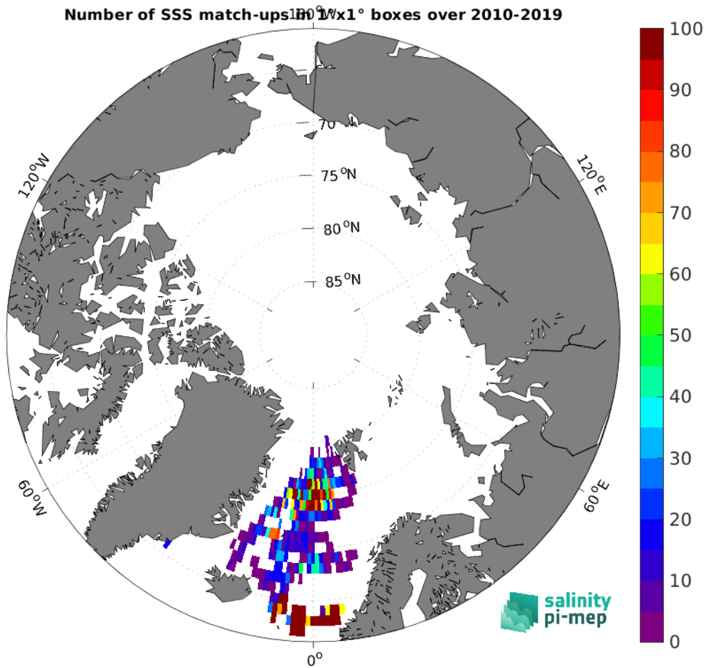
Figure 4: Number of SSS match-ups between Surface drifters SSS and the CCI SSS L4 Merged-OI v4.41 - 30-day running (ESA) SSS product for the Arctic Ocean Pi-MEP region over 1^\circ \times 1^\circ boxes and for the full satellite product period.
