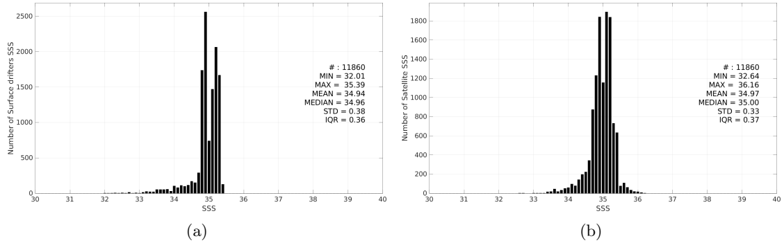
Figure 3: Histograms of SSS from Surface drifters (a) and CCI SSS L4 Merged-OI v4.41 - 30-day running (ESA) (b) considering all match-up pairs per bins of 0.1 over the Arctic Ocean Pi-MEP region and for the full satellite product period.
