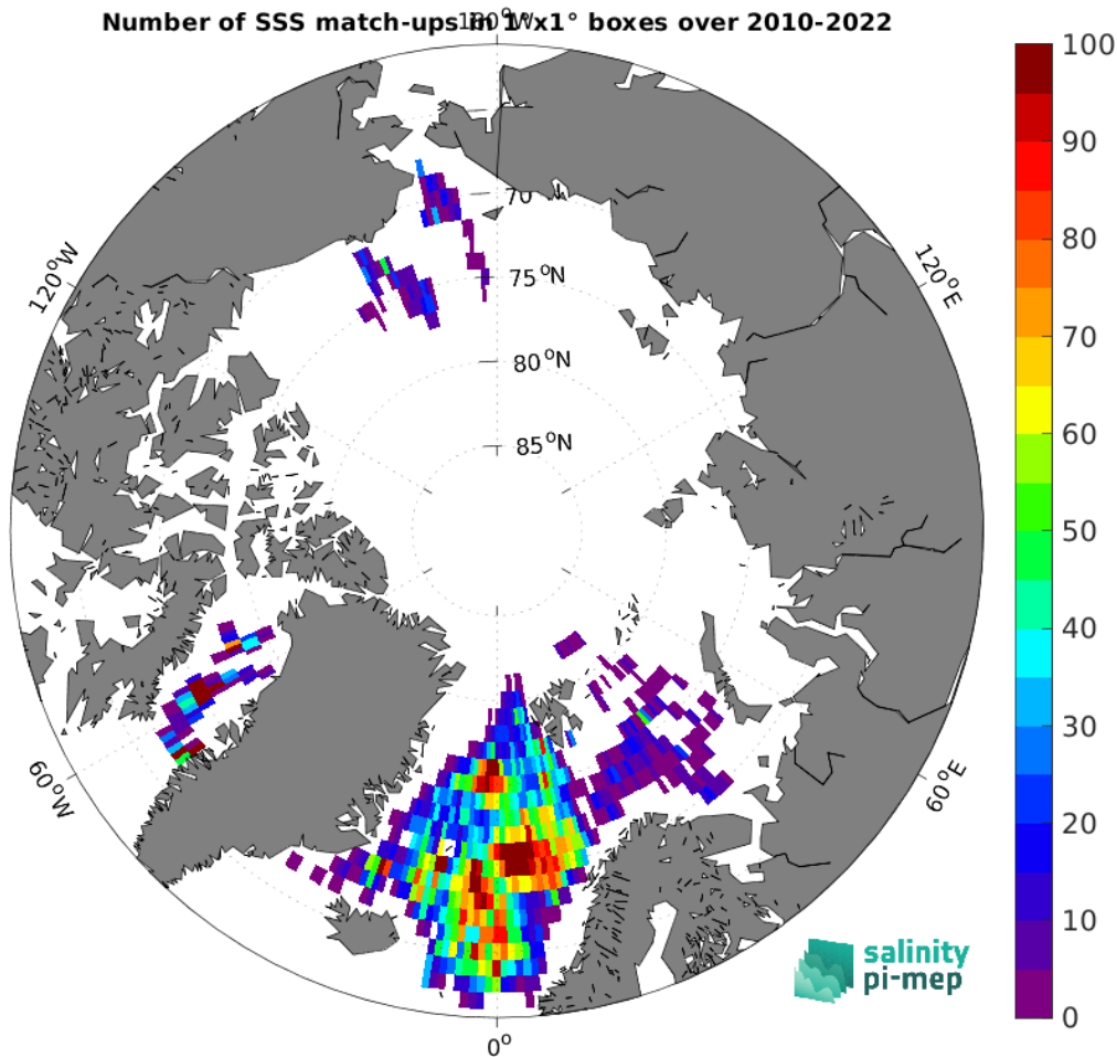
Figure 5: Number of SSS match-ups between Argo SSS and the CCI SSS L4 Merged-OI v4.41 - 30-day running (ESA) SSS product for the Arctic Ocean Pi-MEP region over 1^\circ \times 1^\circ boxes and for the full satellite product period.
