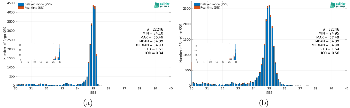
Figure 3: Histograms of SSS from Argo (a) and CCI SSS L4 Merged-OI v4.41 - 30-day running (ESA) (b) considering all match-up pairs per bins of 0.1 over the Arctic Ocean Pi-MEP region and for the full satellite product period.
