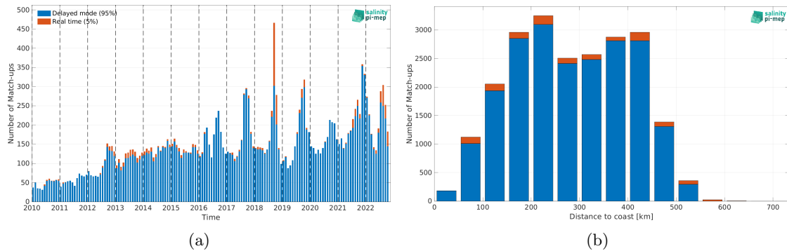
Figure 2: Number of match-ups between Argo and CCI SSS L4 Merged-OI v4.41 - 30-day running (ESA) SSS as a function of time (a) and as function of the distance to coast (b) over the Arctic Ocean Pi-MEP region and for the full satellite product period.
