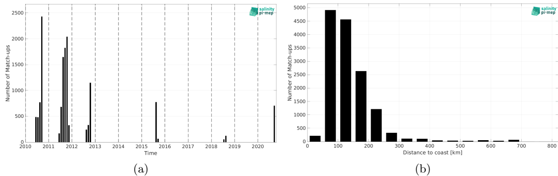
Figure 1: Number of match-ups between TSG (SAMOS) and CCI SSS L4 Merged-OI v4.4 - 7-day running (ESA) SSS as a function of time (a) and as function of the distance to coast (b) over the Arctic Ocean Pi-MEP region and for the full satellite product period.
