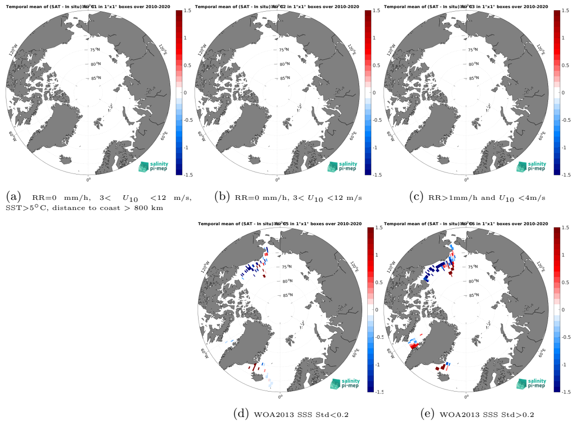
Figure 12: Temporal mean gridded over spatial boxes of size 1^{\circ}\times 1^{\circ} of \Delta\text{SSS} (CCI SSS L4 Merged-OI v4.4 - 7-day running (ESA) - TSG (SAMOS)) for 5 different subdatasets corresponding to: RR=0 mm/h, 3 < U_{10} < 12 m/s, SST > 5^{\circ}\text{C} , distance to coast > 800 km (a), RR=0 mm/h, 3 < U_{10} < 12 m/s (b), RR > 1 mm/h and U_{10} < 4 m/s (c), WOA2013 SSS Std < 0.2 (d), WOA2013 SSS Std > 0.2 (e).
