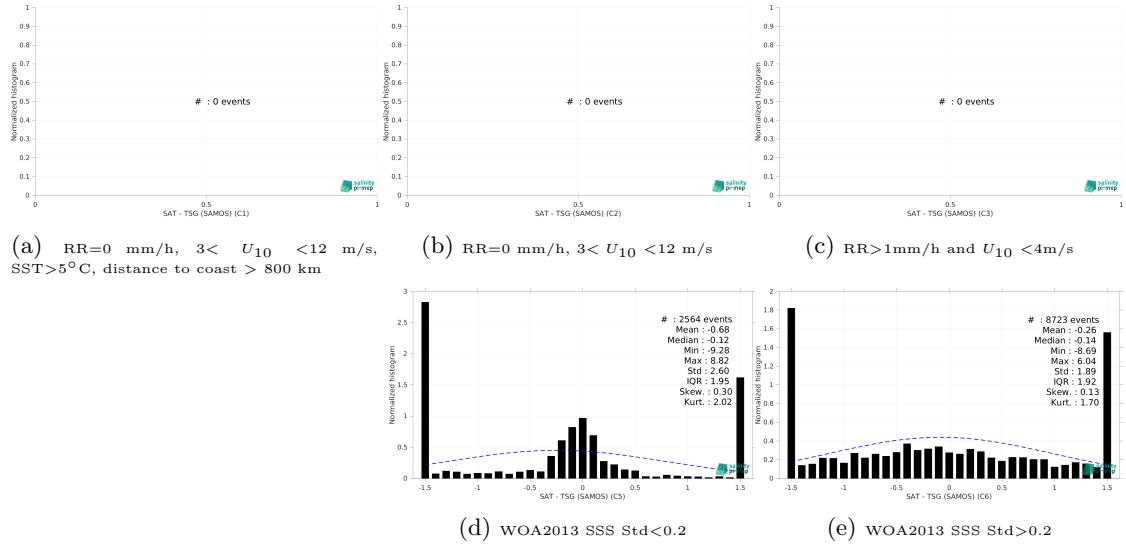
Figure 13: Normalized histogram of \Delta SSS (CCI SSS L4 Merged-OI v4.4 - 7-day running (ESA) - TSG (SAMOS)) for 5 different subdatasets corresponding to: RR=0 mm/h, 3 < U_{10} < 12 m/s, SST > 5°C, distance to coast > 800 km (a), RR=0 mm/h, 3 < U_{10} < 12 m/s (b), RR > 1mm/h and U_{10} < 4 m/s (c), WOA2013 SSS Std < 0.2 (d), WOA2013 SSS Std > 0.2 (e).
