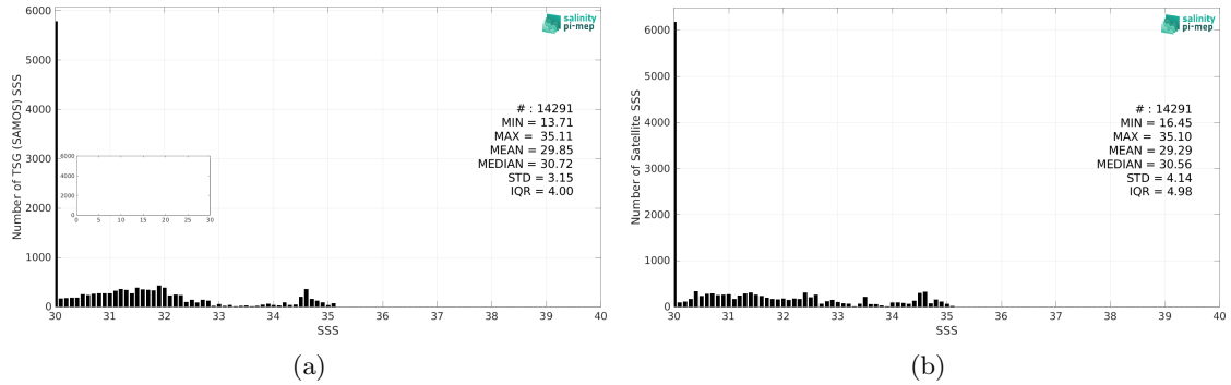
Figure 2: Histograms of SSS from TSG (SAMOS) (a) and CCI SSS L4 Merged-OI v4.4 - 7-day running (ESA) (b) considering all match-up pairs per bins of 0.1 over the Arctic Ocean Pi-MEP region and for the full satellite product period.
