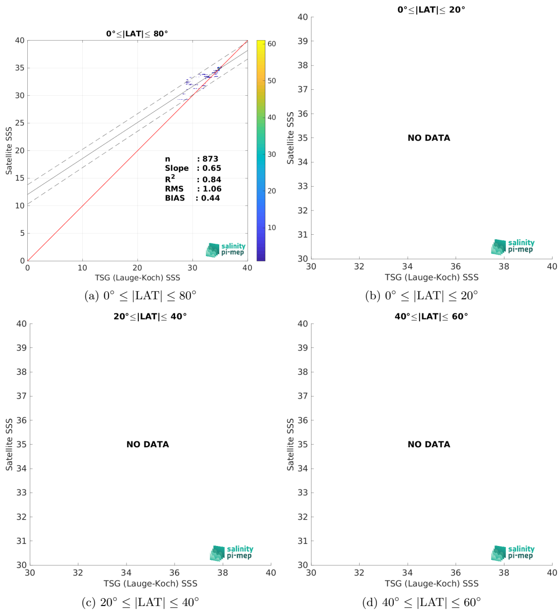
Figure 9: Contour maps of the concentration of CCI SSS L4 Merged-OI v4.4 - 7-day running (ESA) SSS (y-axis) versus TSG (Lauge-Koch) SSS (x-axis) at match-up pairs for different latitude bands. For each plot, the red line shows x=y . The black thin and dashed lines indicate a linear fit through the data cloud and the \pm 95\% confidence levels, respectively. The number match-up pairs n , the slope and R^2 coefficient of the linear fit, the root mean square (RMS) and the mean bias between satellite and in situ data are indicated for each latitude band in each plots.
