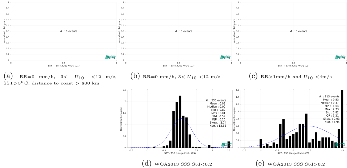
Figure 13: Normalized histogram of \Delta SSS (CCI SSS L4 Merged-OI v4.4 - 7-day running (ESA) - TSG (Lauge-Koch)) for 5 different subdatasets corresponding to: RR=0 mm/h, 3 < U_{10} < 12 m/s, SST > 5°C, distance to coast > 800 km (a), RR=0 mm/h, 3 < U_{10} < 12 m/s (b), RR > 1mm/h and U_{10} < 4 m/s (c), WOA2013 SSS Std < 0.2 (d), WOA2013 SSS Std > 0.2 (e).
