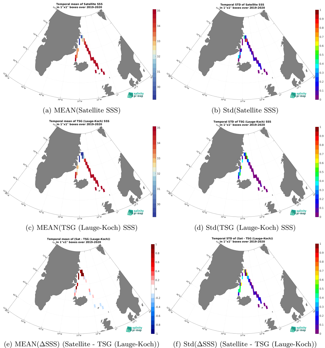
Figure 6: Temporal mean (left) and Std (right) of SSS from CCI SSS L4 Merged-OI v4.4 - 7-day running (ESA) (top), TSG (Lauge-Koch) (middle), and of \Delta SSS (Satellite - TSG (Lauge-Koch)). Only match-up pairs are used to generate these maps.
