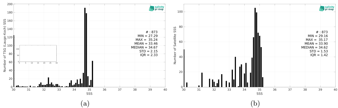
Figure 2: Histograms of SSS from TSG (Lauge-Koch) (a) and CCI SSS L4 Merged-OI v4.4 - 7-day running (ESA) (b) considering all match-up pairs per bins of 0.1 over the Arctic Ocean Pi-MEP region and for the full satellite product period.
