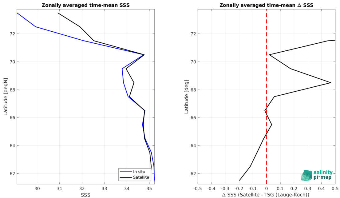
Figure 8: Left panel: Zonal mean SSS from CCI SSS L4 Merged-OI v4.4 - 7-day running (ESA) satellite product (black) and from TSG (Lauge-Koch) (blue). Right panel: Zonal mean of \Delta SSS (Satellite - TSG (Lauge-Koch)) for all the collected Pi-MEP match-up pairs estimated over the full satellite product period.
