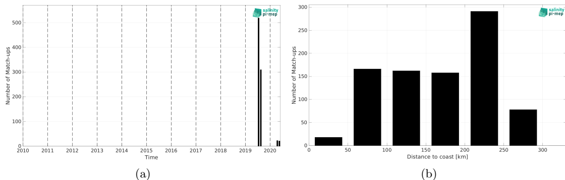
Figure 1: Number of match-ups between TSG (Lauge-Koch) and CCI SSS L4 Merged-OI v4.4 - 7-day running (ESA) SSS as a function of time (a) and as function of the distance to coast (b) over the Arctic Ocean Pi-MEP region and for the full satellite product period.
