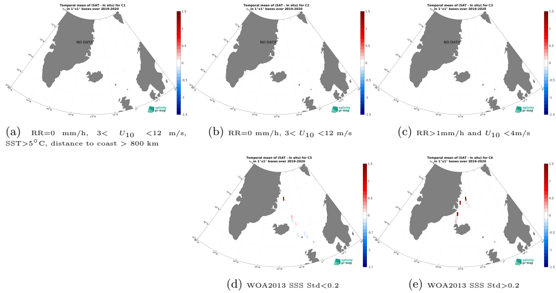
Figure 12: Temporal mean gridded over spatial boxes of size 1^{\circ}\times 1^{\circ} of \Delta\text{SSS} (CCI SSS L4 Merged-OI v4.4 - 7-day running (ESA) - TSG (Lauge-Koch)) for 5 different subdatasets corresponding to:RR=0 mm/h, 3 < U_{10} < 12 m/s, SST >5^{\circ}\text{C} , distance to coast > 800 km (a), RR=0 mm/h, 3 < U_{10} < 12 m/s (b), RR >1 mm/h and U_{10} < 4 m/s (c), WOA2013 SSS Std <0.2 (d), WOA2013 SSS Std >0.2 (e).
