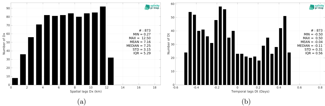
Figure 5: Histograms of the spatial (a) and temporal (b) lags between the location/time of the TSG (Lauge-Koch) measurement and the date of the corresponding CCI SSS L4 Merged-OI v4.4 - 7-day running (ESA) SSS pixel.
