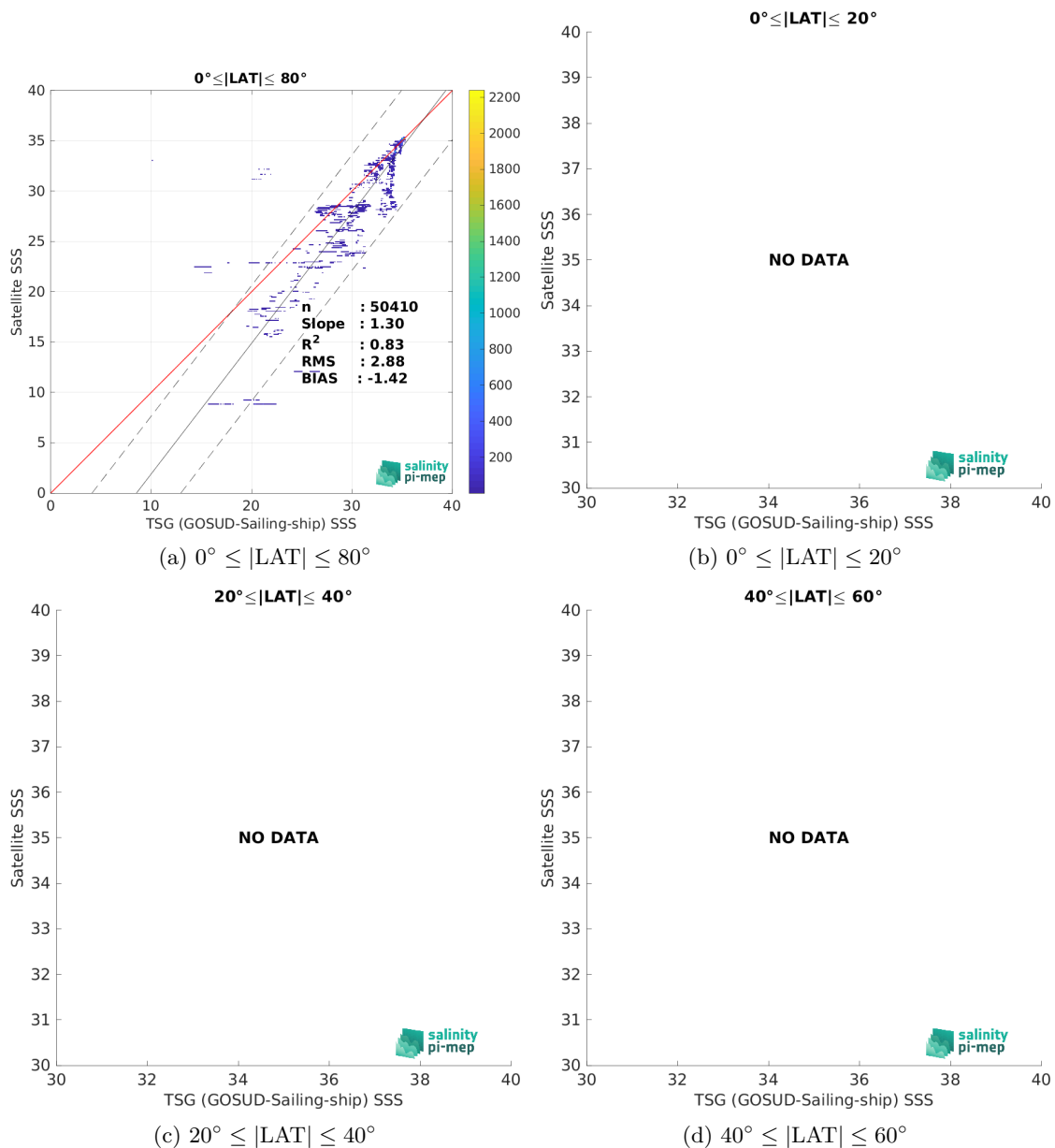
Figure 9: Contour maps of the concentration of CCI SSS L4 Merged-OI v4.4 - 7-day running (ESA) SSS (y-axis) versus TSG (GOSUD-Sailing-ship) SSS (x-axis) at match-up pairs for different latitude bands. For each plot, the red line shows x=y . The black thin and dashed lines indicate a linear fit through the data cloud and the \pm 95\% confidence levels, respectively. The number match-up pairs n , the slope and R^2 coefficient of the linear fit, the root mean square (RMS) and the mean bias between satellite and in situ data are indicated for each latitude band in each plots.
