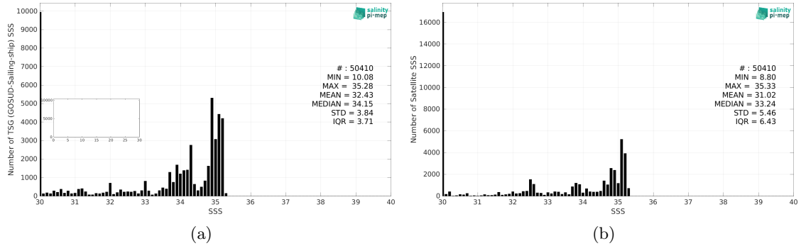
Figure 2: Histograms of SSS from TSG (GOSUD-Sailing-ship) (a) and CCI SSS L4 Merged-OI v4.4 - 7-day running (ESA) (b) considering all match-up pairs per bins of 0.1 over the Arctic Ocean Pi-MEP region and for the full satellite product period.
