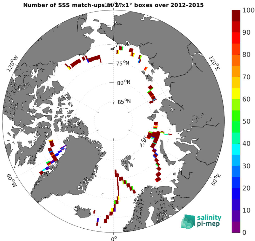
Figure 4: Number of SSS match-ups between TSG (GOSUD-Sailing-ship) SSS and the CCI SSS L4 Merged-OI v4.4 - 7-day running (ESA) SSS product for the Arctic Ocean Pi-MEP region over 1^\circ \times 1^\circ boxes and for the full satellite product period.
