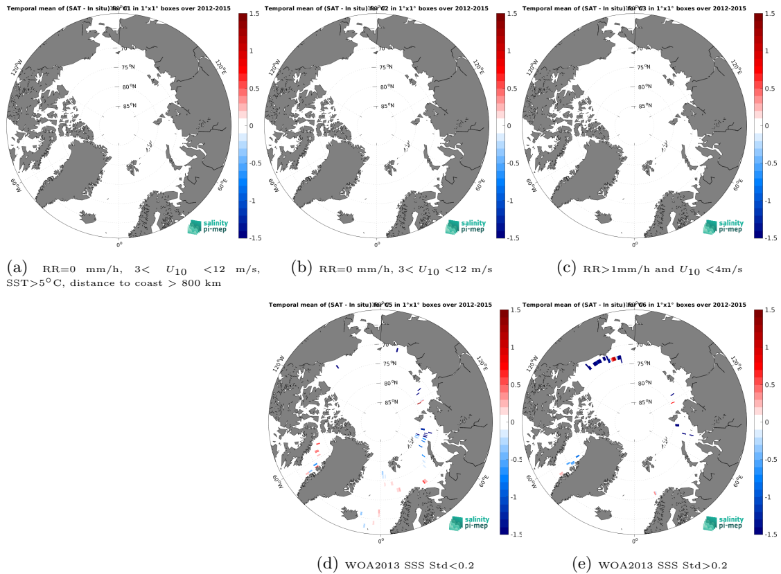
Figure 12: Temporal mean gridded over spatial boxes of size 1^\circ \times 1^\circ of \Delta SSS (CCI SSS L4 Merged-OI v4.4 - 7-day running (ESA) - TSG (GOSUD-Sailing-ship)) for 5 different subdatasets corresponding to: RR=0 mm/h, 3 < U_{10} < 12 m/s, SST > 5°C, distance to coast > 800 km (a), RR=0 mm/h, 3 < U_{10} < 12 m/s (b), RR > 1mm/h and U_{10} < 4 m/s (c), WOA2013 SSS Std < 0.2 (d), WOA2013 SSS Std > 0.2 (e).
