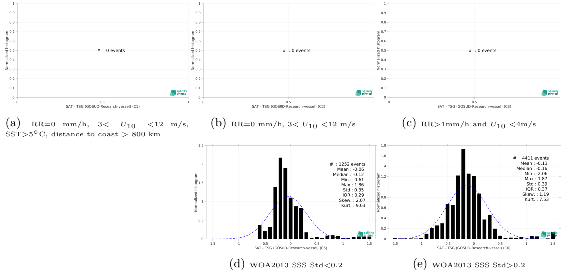
Figure 13: Normalized histogram of \Delta SSS (CCI SSS L4 Merged-OI v4.4 - 7-day running (ESA) - TSG (GOSUD-Research-vessel)) for 5 different subdatasets corresponding to: RR=0 mm/h, 3 < U_{10} < 12 m/s, SST > 5°C, distance to coast > 800 km (a), RR=0 mm/h, 3 < U_{10} < 12 m/s (b), RR > 1mm/h and U_{10} < 4 m/s (c), WOA2013 SSS Std < 0.2 (d), WOA2013 SSS Std > 0.2 (e).
