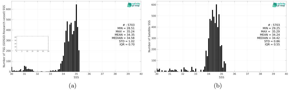
Figure 2: Histograms of SSS from TSG (GOSUD-Research-vessel) (a) and CCI SSS L4 Merged-OI v4.4 - 7-day running (ESA) (b) considering all match-up pairs per bins of 0.1 over the Arctic Ocean Pi-MEP region and for the full satellite product period.
