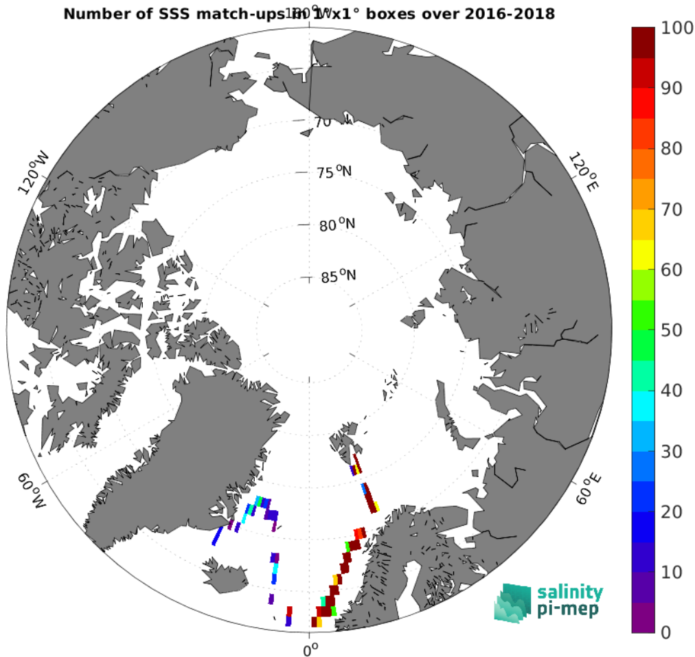
Figure 4: Number of SSS match-ups between TSG (GOSUD-Research-vessel) SSS and the CCI SSS L4 Merged-OI v4.4 - 7-day running (ESA) SSS product for the Arctic Ocean Pi-MEP region over 1^\circ \times 1^\circ boxes and for the full satellite product period.
