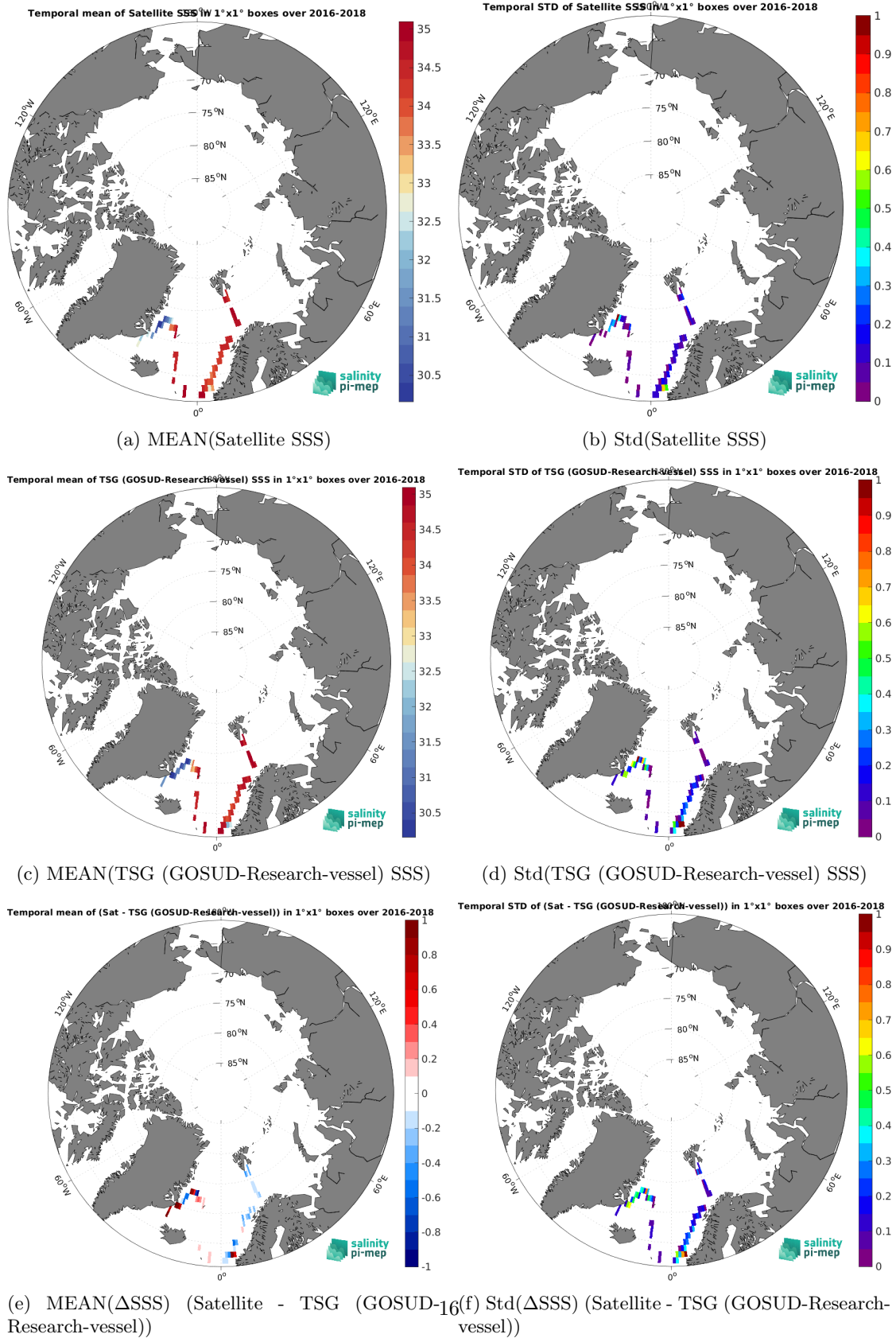
Figure 6: Temporal mean (left) and Std (right) of SSS from CCI SSS L4 Merged-OI v4.4 - 7-day running (ESA) (top), TSG (GOSUD-Research-vessel) (middle), and of \Delta SSS (Satellite - TSG (GOSUD-Research-vessel)). Only match-up pairs are used to generate these maps.
