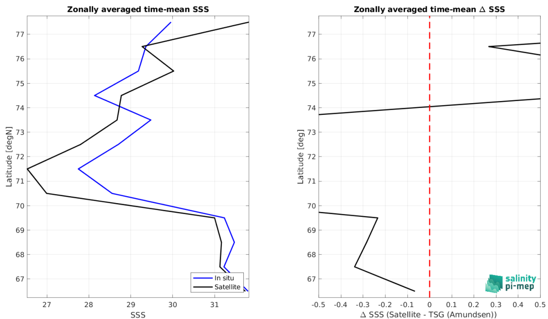
Figure 8: Left panel: Zonal mean SSS from CCI SSS L4 Merged-OI v4.4 - 7-day running (ESA) satellite product (black) and from TSG (Amundsen) (blue). Right panel: Zonal mean of \Delta SSS (Satellite - TSG (Amundsen)) for all the collected Pi-MEP match-up pairs estimated over the full satellite product period.
