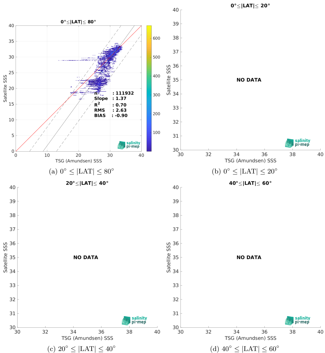
Figure 9: Contour maps of the concentration of CCI SSS L4 Merged-OI v4.4 - 7-day running (ESA) SSS (y-axis) versus TSG (Amundsen) SSS (x-axis) at match-up pairs for different latitude bands. For each plot, the red line shows x=y . The black thin and dashed lines indicate a linear fit through the data cloud and the \pm 95\% confidence levels, respectively. The number match-up pairs n , the slope and R^2 coefficient of the linear fit, the root mean square (RMS) and the mean bias between satellite and in situ data are indicated for each latitude band in each plots.
