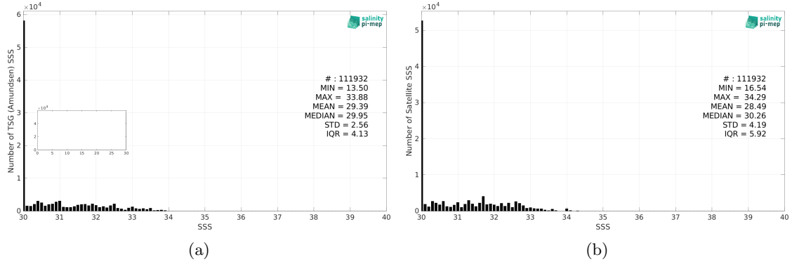
Figure 2: Histograms of SSS from TSG (Amundsen) (a) and CCI SSS L4 Merged-OI v4.4 - 7-day running (ESA) (b) considering all match-up pairs per bins of 0.1 over the Arctic Ocean Pi-MEP region and for the full satellite product period.
