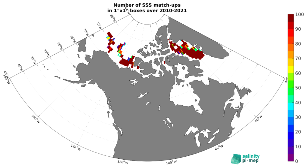
Figure 4: Number of SSS match-ups between TSG (Amundsen) SSS and the CCI SSS L4 Merged-OI v4.4 - 7-day running (ESA) SSS product for the Arctic Ocean Pi-MEP region over 1°x1° boxes and for the full satellite product period.
