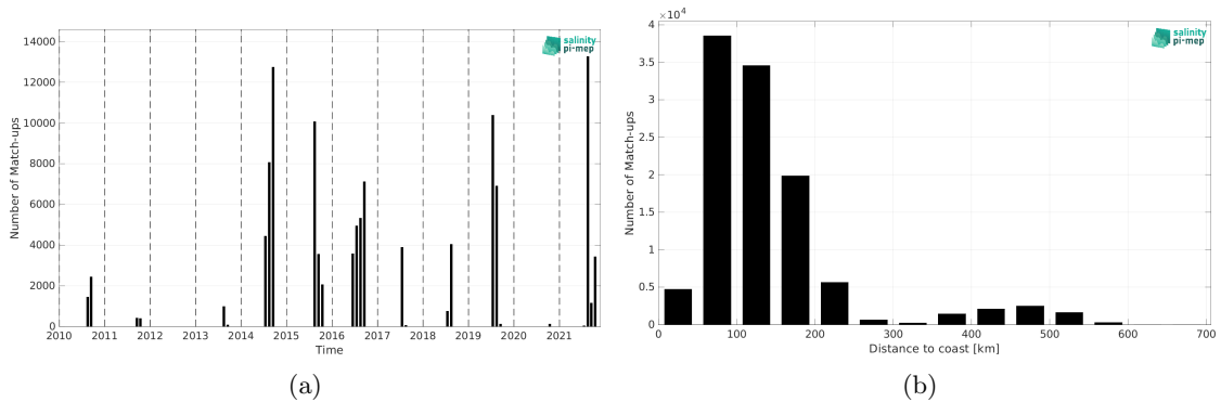
Figure 1: Number of match-ups between TSG (Amundsen) and CCI SSS L4 Merged-OI v4.4 - 7-day running (ESA) SSS as a function of time (a) and as function of the distance to coast (b) over the Arctic Ocean Pi-MEP region and for the full satellite product period.
