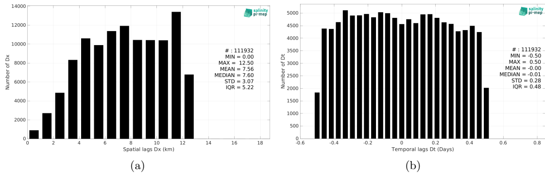
Figure 5: Histograms of the spatial (a) and temporal (b) lags between the location/time of the TSG (Amundsen) measurement and the date of the corresponding CCI SSS L4 Merged-OI v4.4 - 7-day running (ESA) SSS pixel.
