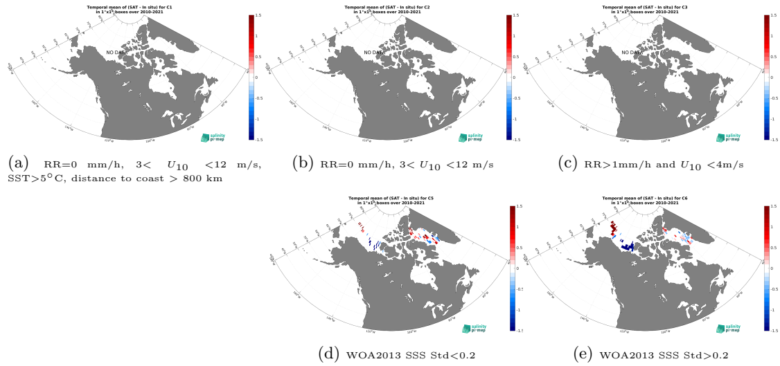
Figure 12: Temporal mean gridded over spatial boxes of size 1^{\circ}\times 1^{\circ} of \Delta\text{SSS} (CCI SSS L4 Merged-OI v4.4 - 7-day running (ESA) - TSG (Amundsen)) for 5 different subdatasets corresponding to:RR=0 mm/h, 3 < U_{10} < 12 m/s, SST > 5^{\circ}\text{C} , distance to coast > 800 km (a), RR=0 mm/h, 3 < U_{10} < 12 m/s (b), RR > 1 mm/h and U_{10} < 4 m/s (c), WOA2013 SSS Std < 0.2 (d), WOA2013 SSS Std > 0.2 (e).
