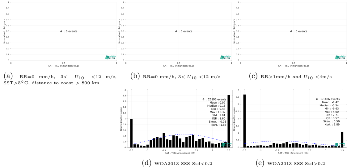
Figure 13: Normalized histogram of \Delta SSS (CCI SSS L4 Merged-OI v4.4 - 7-day running (ESA) - TSG (Amundsen)) for 5 different subdatasets corresponding to: RR=0 mm/h, 3 < U_{10} < 12 m/s, SST>5°C, distance to coast > 800 km (a), RR=0 mm/h, 3 < U_{10} < 12 m/s (b), RR>1mm/h and U_{10} < 4 m/s (c), WOA2013 SSS Std<0.2 (d), WOA2013 SSS Std>0.2 (e).
