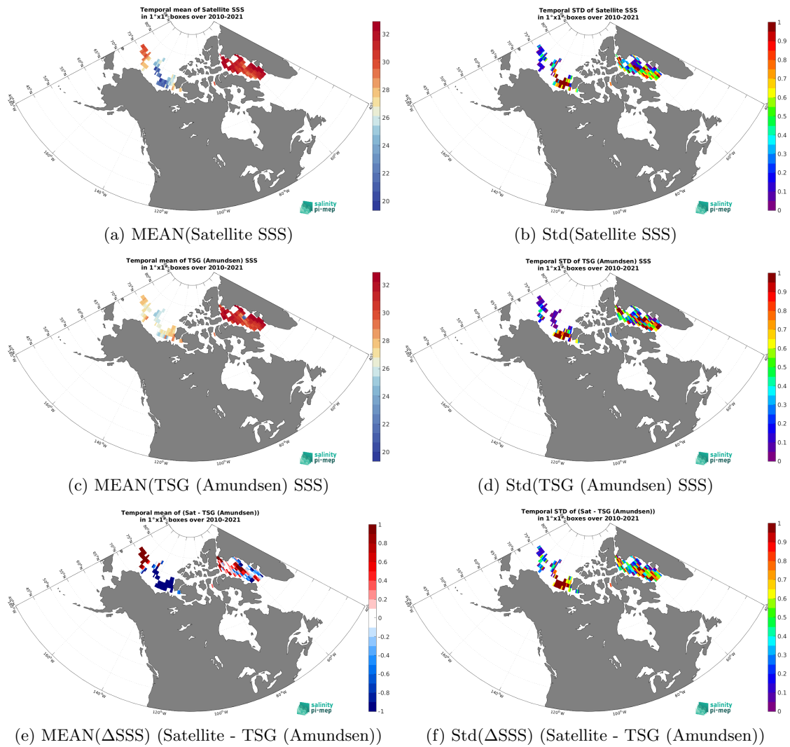
Figure 6: Temporal mean (left) and Std (right) of SSS from CCI SSS L4 Merged-OI v4.4 - 7-day running (ESA) (top), TSG (Amundsen) (middle), and of \Delta SSS (Satellite - TSG (Amundsen)). Only match-up pairs are used to generate these maps.
