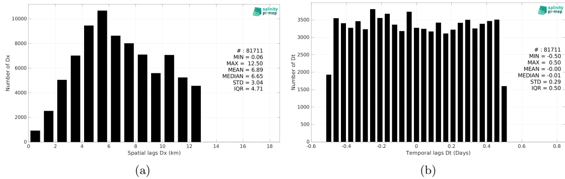
Figure 5: Histograms of the spatial (a) and temporal (b) lags between the location/time of the ICES measurement and the date of the corresponding CCI SSS L4 Merged-OI v4.4 - 7-day running (ESA) SSS pixel.
