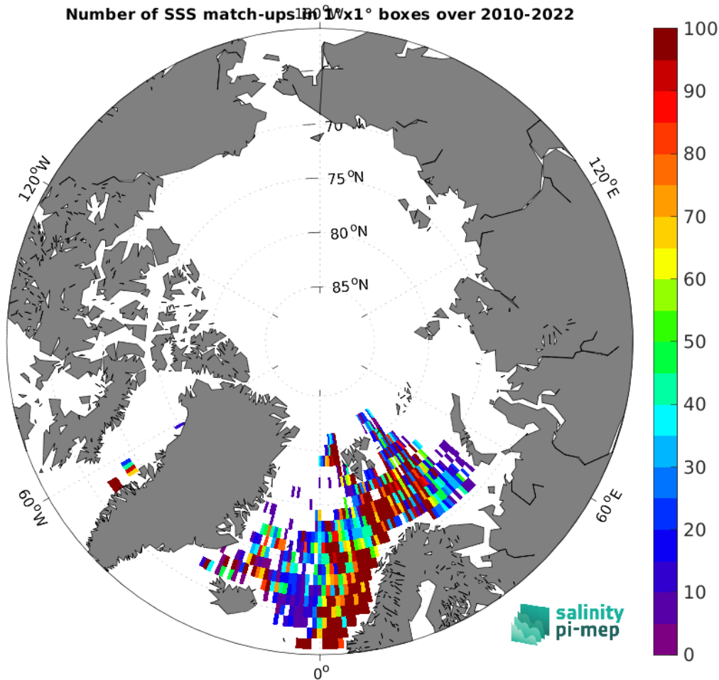
Figure 4: Number of SSS match-ups between ICES SSS and the CCI SSS L4 Merged-OI v4.4 - 7-day running (ESA) SSS product for the Arctic Ocean Pi-MEP region over 1^\circ \times 1^\circ boxes and for the full satellite product period.
