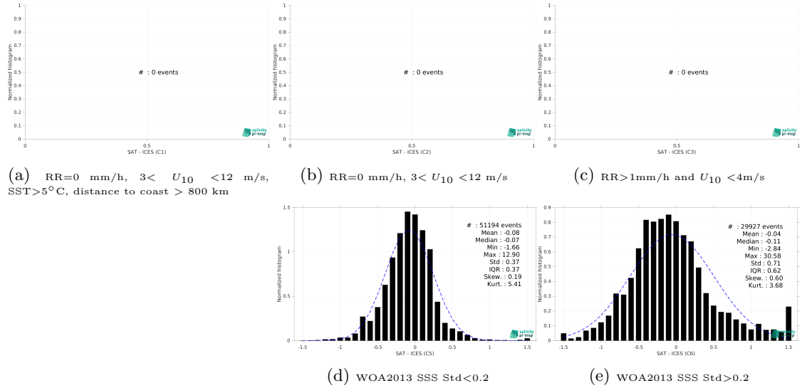
Figure 13: Normalized histogram of \Delta SSS (CCI SSS L4 Merged-OI v4.4 - 7-day running (ESA) - ICES) for 5 different subdatasets corresponding to: RR=0 mm/h, 3 < U_{10} < 12 m/s, SST >5^{\circ} C, distance to coast > 800 km (a), RR=0 mm/h, 3 < U_{10} < 12 m/s (b), RR >1 mm/h and U_{10} < 4 m/s (c), WOA2013 SSS Std <0.2 (d), WOA2013 SSS Std >0.2 (e).
