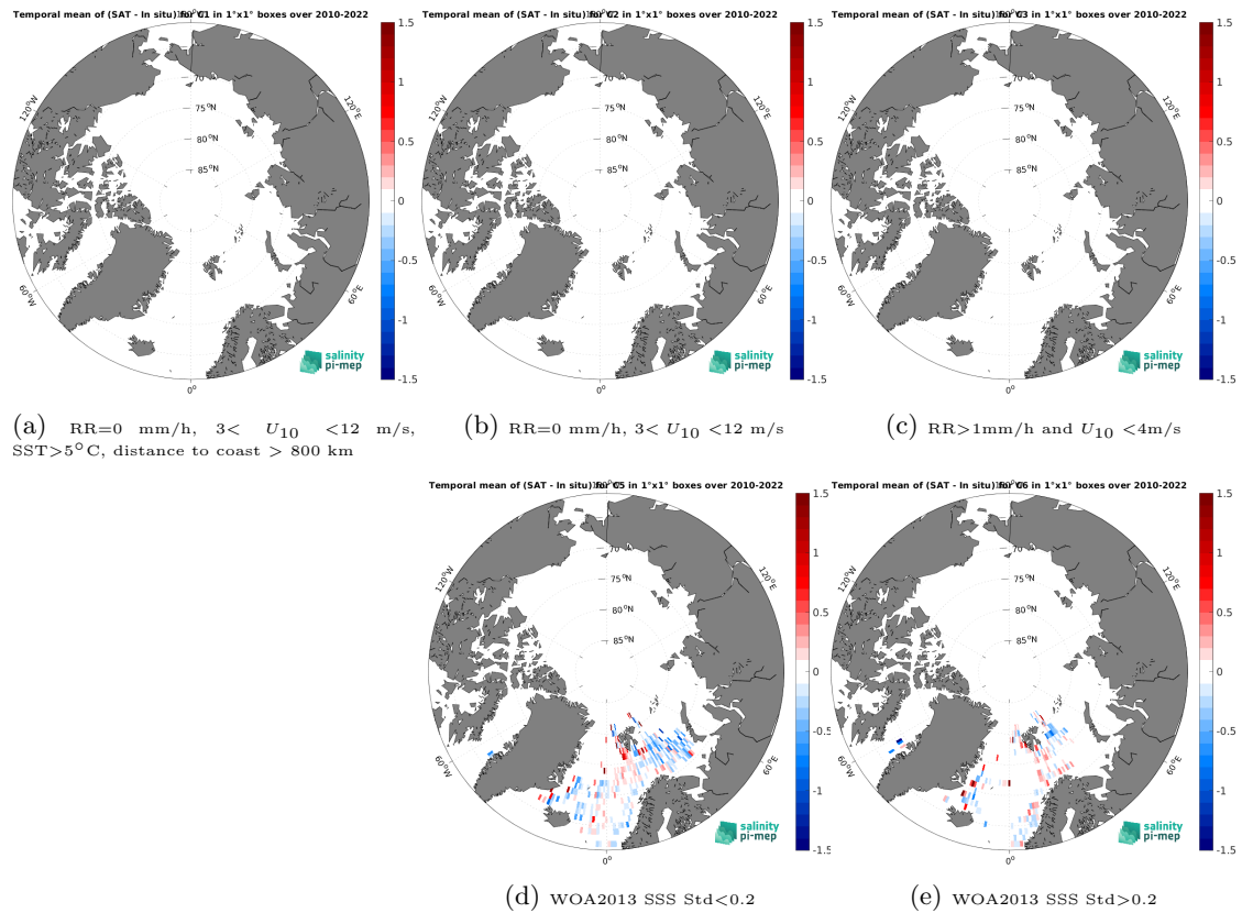
Figure 12: Temporal mean gridded over spatial boxes of size 1^{\circ}\times 1^{\circ} of \Delta\text{SSS} (CCI SSS L4 Merged-OI v4.4 - 7-day running (ESA) - ICES) for 5 different subdatasets corresponding to:RR=0 mm/h, 3 < U_{10} < 12 m/s, SST > 5^{\circ}\text{C} , distance to coast > 800 km (a), RR=0 mm/h, 3 < U_{10} < 12 m/s (b), RR > 1 mm/h and U_{10} < 4 m/s (c), WOA2013 SSS Std < 0.2 (d), WOA2013 SSS Std > 0.2 (e).
