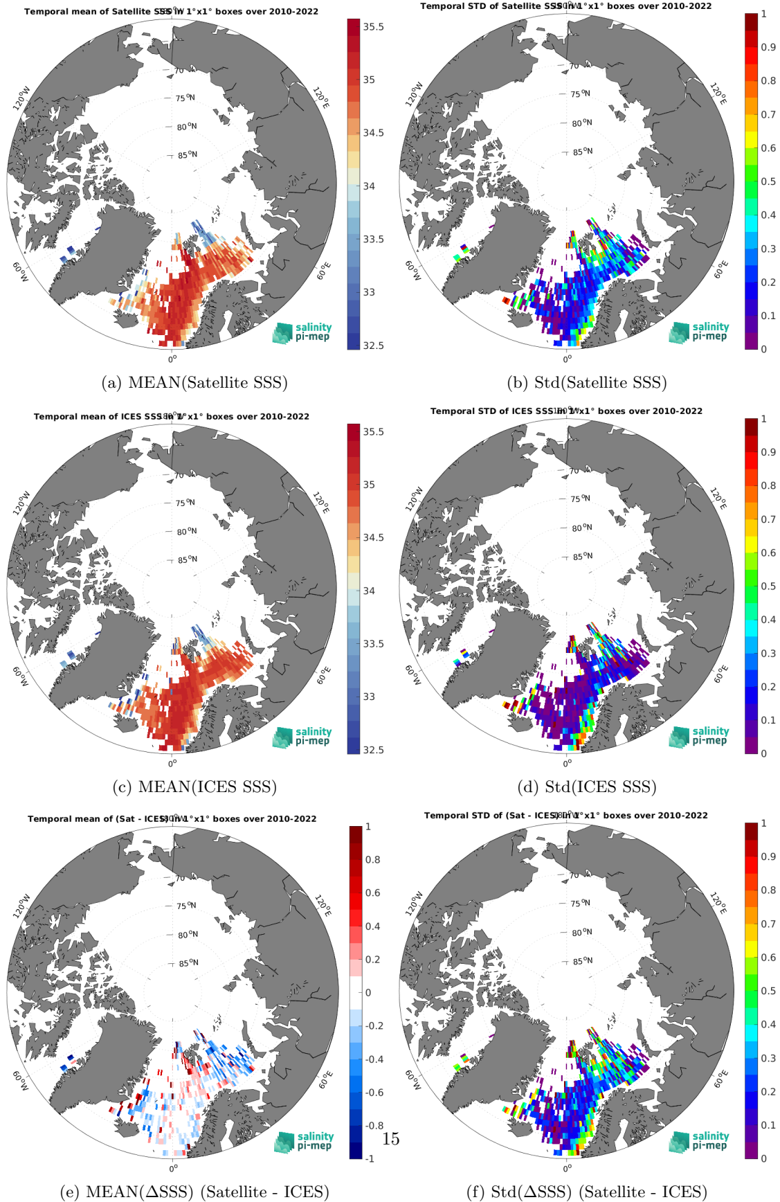
Figure 6: Temporal mean (left) and Std (right) of SSS from CCI SSS L4 Merged-OI v4.4 - 7-day running (ESA) (top), ICES (middle), and of \Delta SSS (Satellite - ICES). Only match-up pairs are used to generate these maps.
