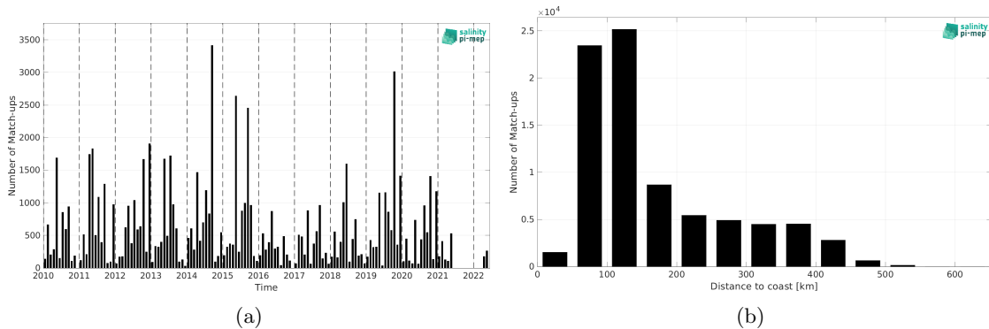
Figure 1: Number of match-ups between ICES and CCI SSS L4 Merged-OI v4.4 - 7-day running (ESA) SSS as a function of time (a) and as function of the distance to coast (b) over the Arctic Ocean Pi-MEP region and for the full satellite product period.
