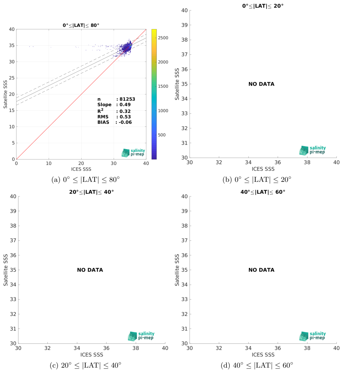
Figure 9: Contour maps of the concentration of CCI SSS L4 Merged-OI v4.4 - 7-day running (ESA) SSS (y-axis) versus ICES SSS (x-axis) at match-up pairs for different latitude bands. For each plot, the red line shows x=y . The black thin and dashed lines indicate a linear fit through the data cloud and the \pm 95\% confidence levels, respectively. The number match-up pairs n , the slope and R^2 coefficient of the linear fit, the root mean square (RMS) and the mean bias between satellite and in situ data are indicated for each latitude band in each plots.
