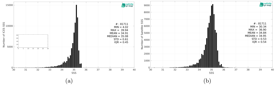
Figure 2: Histograms of SSS from ICES (a) and CCI SSS L4 Merged-OI v4.4 - 7-day running (ESA) (b) considering all match-up pairs per bins of 0.1 over the Arctic Ocean Pi-MEP region and for the full satellite product period.
