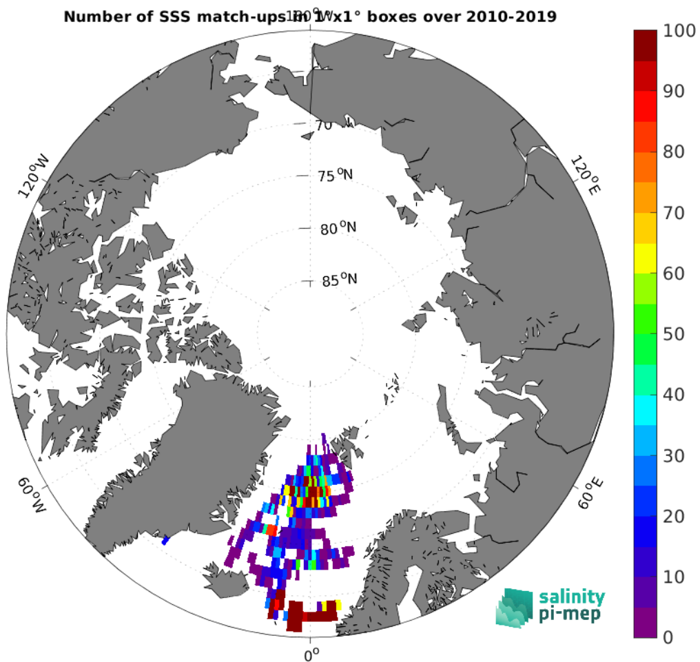
Figure 3: Number of SSS match-ups between Surface drifters SSS and the CCI SSS L4 Merged-OI v4.4 - 7-day running (ESA) SSS product for the Arctic Ocean Pi-MEP region over 1^\circ \times 1^\circ boxes and for the full satellite product period.
