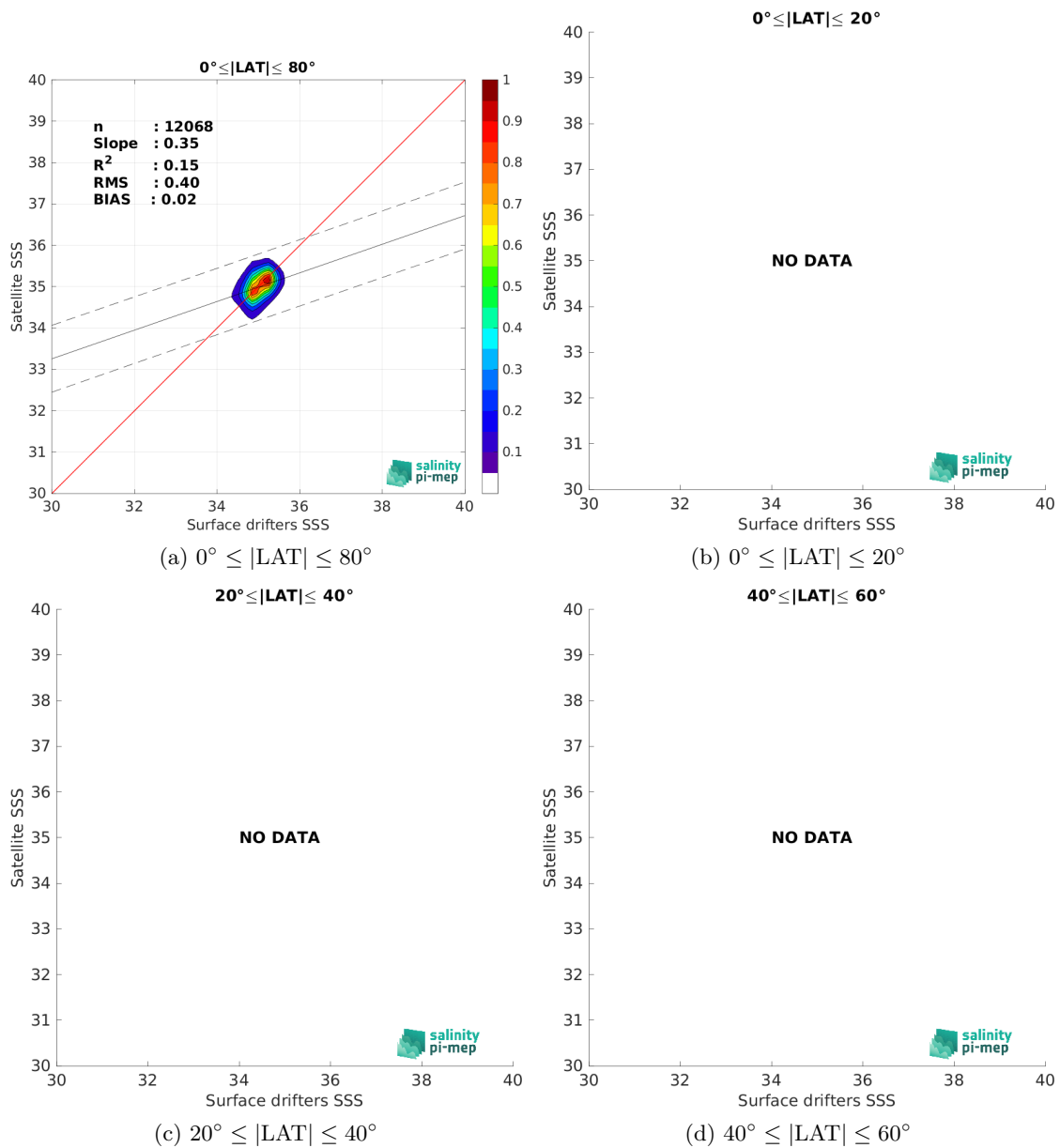
Figure 8: Contour maps of the concentration of CCI SSS L4 Merged-OI v4.4 - 7-day running (ESA) SSS (y-axis) versus Surface drifters SSS (x-axis) at match-up pairs for different latitude bands. For each plot, the red line shows x=y . The black thin and dashed lines indicate a linear fit through the data cloud and the \pm 95\% confidence levels, respectively. The number match-up pairs n , the slope and R^2 coefficient of the linear fit, the root mean square (RMS) and the mean bias between satellite and in situ data are indicated for each latitude band in each plots.
