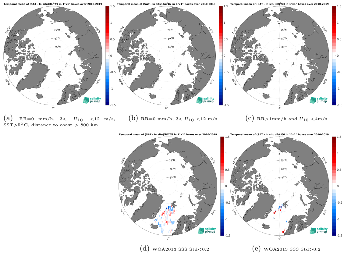
Figure 11: Temporal mean gridded over spatial boxes of size 1^{\circ}\times 1^{\circ} of \Delta\text{SSS} (CCI SSS L4 Merged-OI v4.4 - 7-day running (ESA) - Surface drifters) for 5 different subdatasets corresponding to:RR=0 mm/h, 3 < U_{10} < 12 m/s, SST >5^{\circ}\text{C} , distance to coast > 800 km (a), RR=0 mm/h, 3 < U_{10} < 12 m/s (b), RR >1 mm/h and U_{10} < 4 m/s (c), WOA2013 SSS Std <0.2 (d), WOA2013 SSS Std >0.2 (e).
