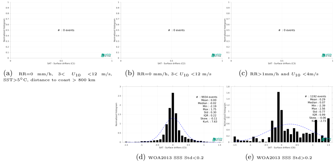
Figure 12: Normalized histogram of \Delta SSS (CCI SSS L4 Merged-OI v4.4 - 7-day running (ESA) - Surface drifters) for 5 different subdatasets corresponding to: RR=0 mm/h, 3 < U_{10} < 12 m/s, SST>5°C, distance to coast > 800 km (a), RR=0 mm/h, 3 < U_{10} < 12 m/s (b), RR>1mm/h and U_{10} < 4 m/s (c), WOA2013 SSS Std<0.2 (d), WOA2013 SSS Std>0.2 (e).
