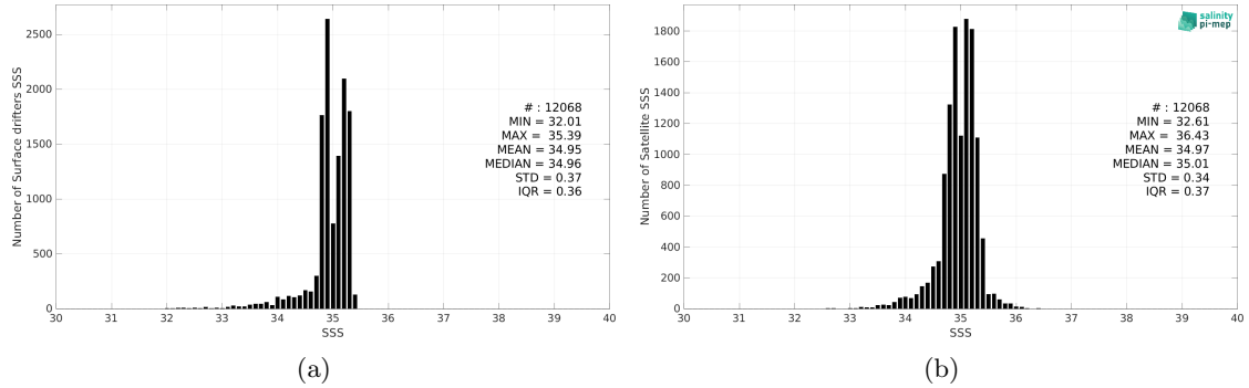
Figure 2: Histograms of SSS from Surface drifters (a) and CCI SSS L4 Merged-OI v4.4 - 7-day running (ESA) (b) considering all match-up pairs per bins of 0.1 over the Arctic Ocean Pi-MEP region and for the full satellite product period.
