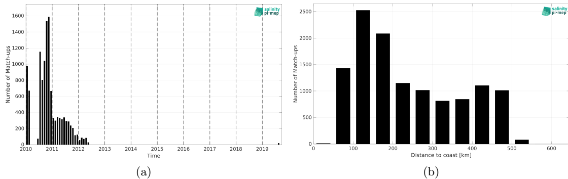
Figure 1: Number of match-ups between Surface drifters and CCI SSS L4 Merged-OI v4.4 - 7-day running (ESA) SSS as a function of time (a) and as function of the distance to coast (b) over the Arctic Ocean Pi-MEP region and for the full satellite product period.
