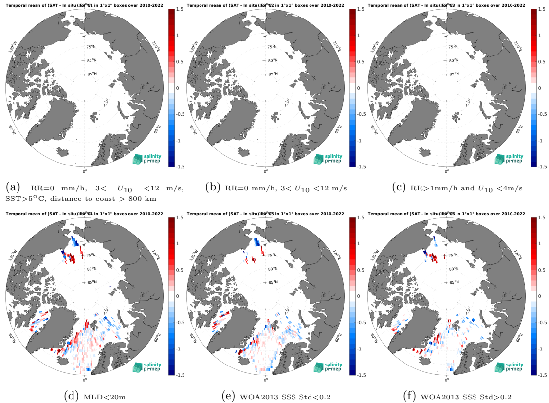
Figure 12: Temporal mean gridded over spatial boxes of size 1^{\circ}\times 1^{\circ} of \Delta\text{SSS} (CCI SSS L4 Merged-OI v4.4 - 7-day running (ESA) - Argo) for 6 different subdatasets corresponding to:RR=0 mm/h, 3 < U_{10} < 12 m/s, SST >5^{\circ}\text{C} , distance to coast > 800 km (a), RR=0 mm/h, 3 < U_{10} < 12 m/s (b), RR >1 mm/h and U_{10} < 4 m/s (c),MLD <20 m (d),WOA2013 SSS Std <0.2 (e),WOA2013 SSS Std >0.2 (f).
