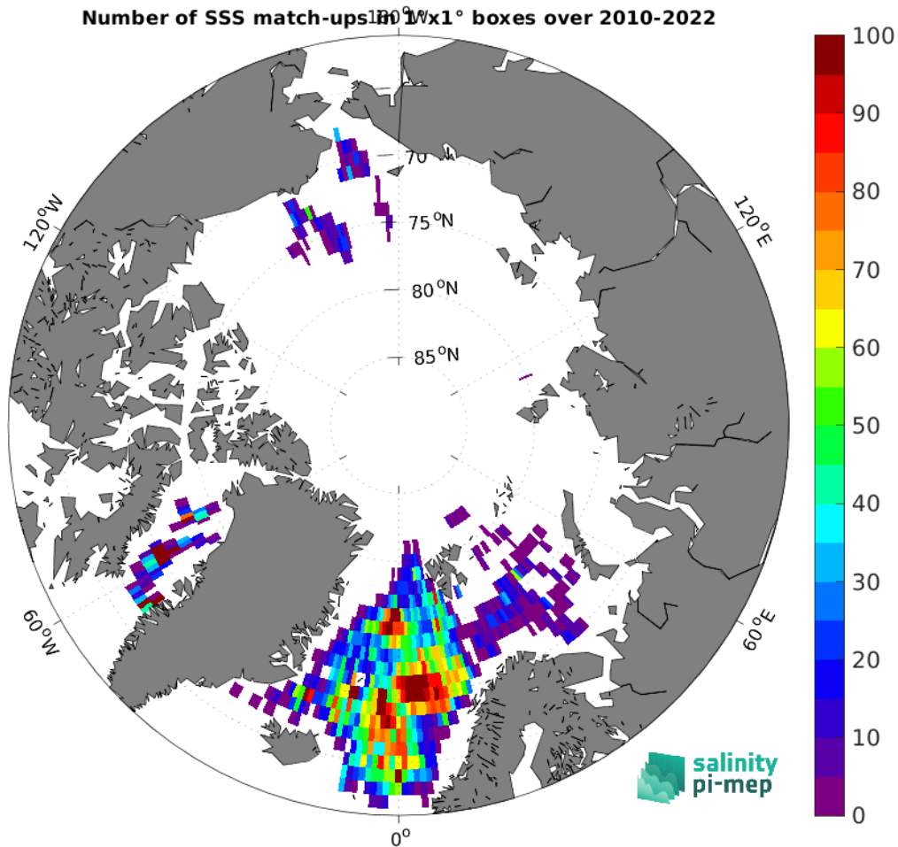
Figure 4: Number of SSS match-ups between Argo SSS and the CCI SSS L4 Merged-OI v4.4 - 7-day running (ESA) SSS product for the Arctic Ocean Pi-MEP region over 1^\circ \times 1^\circ boxes and for the full satellite product period.
