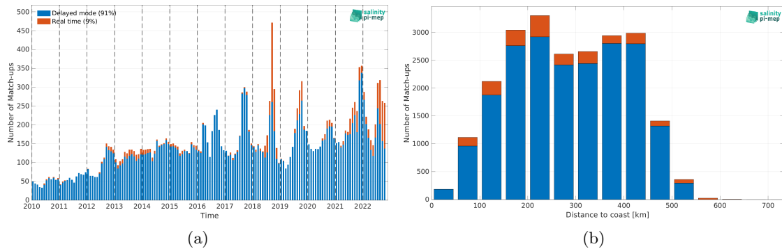
Figure 1: Number of match-ups between Argo and CCI SSS L4 Merged-OI v4.4 - 7-day running (ESA) SSS as a function of time (a) and as function of the distance to coast (b) over the Arctic Ocean Pi-MEP region and for the full satellite product period.
