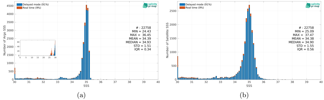
Figure 2: Histograms of SSS from Argo (a) and CCI SSS L4 Merged-OI v4.4 - 7-day running (ESA) (b) considering all match-up pairs per bins of 0.1 over the Arctic Ocean Pi-MEP region and for the full satellite product period.
