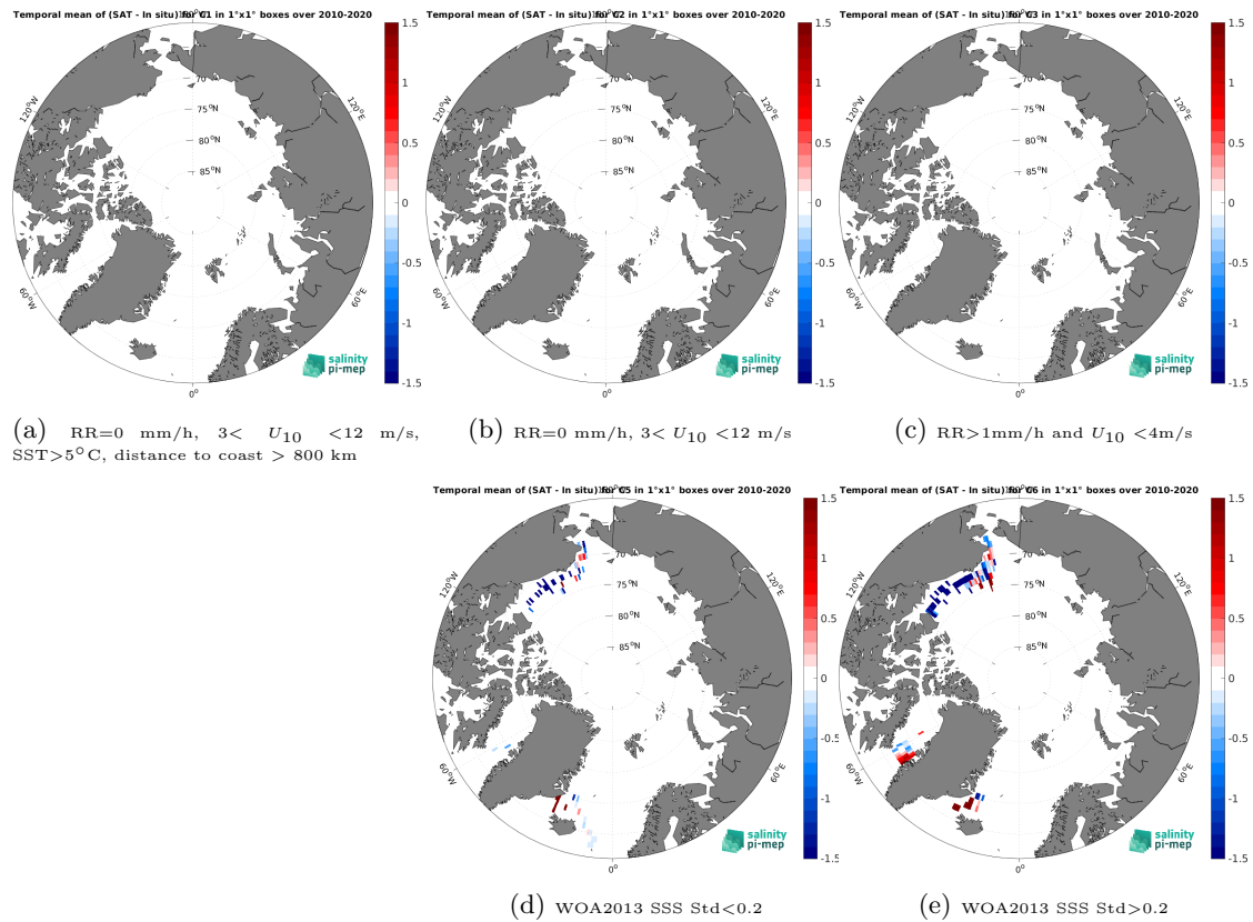
Figure 12: Temporal mean gridded over spatial boxes of size 1^{\circ}\times 1^{\circ} of \Delta\text{SSS} (CCI SSS L4 Merged-OI v4.4 - 30-day running (ESA) - TSG (SAMOS)) for 5 different subdatasets corresponding to:RR=0 mm/h, 3 < U_{10} < 12 m/s, SST >5^{\circ}\text{C} , distance to coast > 800 km (a), RR=0 mm/h, 3 < U_{10} < 12 m/s (b), RR >1 mm/h and U_{10} < 4 m/s (c), WOA2013 SSS Std <0.2 (d), WOA2013 SSS Std >0.2 (e).
