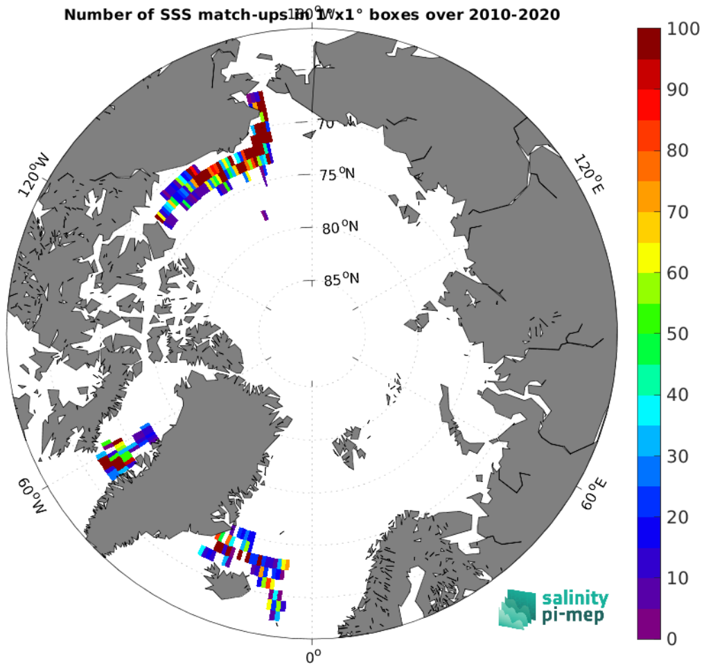
Figure 4: Number of SSS match-ups between TSG (SAMOS) SSS and the CCI SSS L4 Merged-OI v4.4 - 30-day running (ESA) SSS product for the Arctic Ocean Pi-MEP region over 1^\circ \times 1^\circ boxes and for the full satellite product period.
