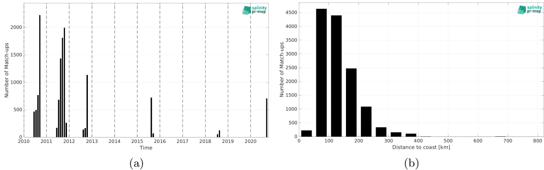
Figure 1: Number of match-ups between TSG (SAMOS) and CCI SSS L4 Merged-OI v4.4 - 30-day running (ESA) SSS as a function of time (a) and as function of the distance to coast (b) over the Arctic Ocean Pi-MEP region and for the full satellite product period.
