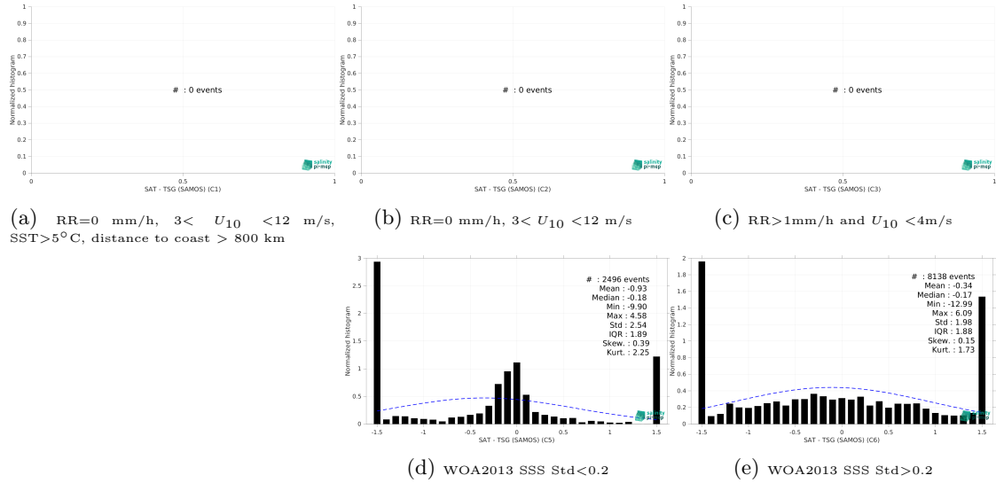
Figure 13: Normalized histogram of \Delta SSS (CCI SSS L4 Merged-OI v4.4 - 30-day running (ESA) - TSG (SAMOS)) for 5 different subdatasets corresponding to: RR=0 mm/h, 3 < U_{10} < 12 m/s, SST >5^{\circ} C, distance to coast > 800 km (a), RR=0 mm/h, 3 < U_{10} < 12 m/s (b), RR >1 mm/h and U_{10} < 4 m/s (c), WOA2013 SSS Std <0.2 (d), WOA2013 SSS Std >0.2 (e).
