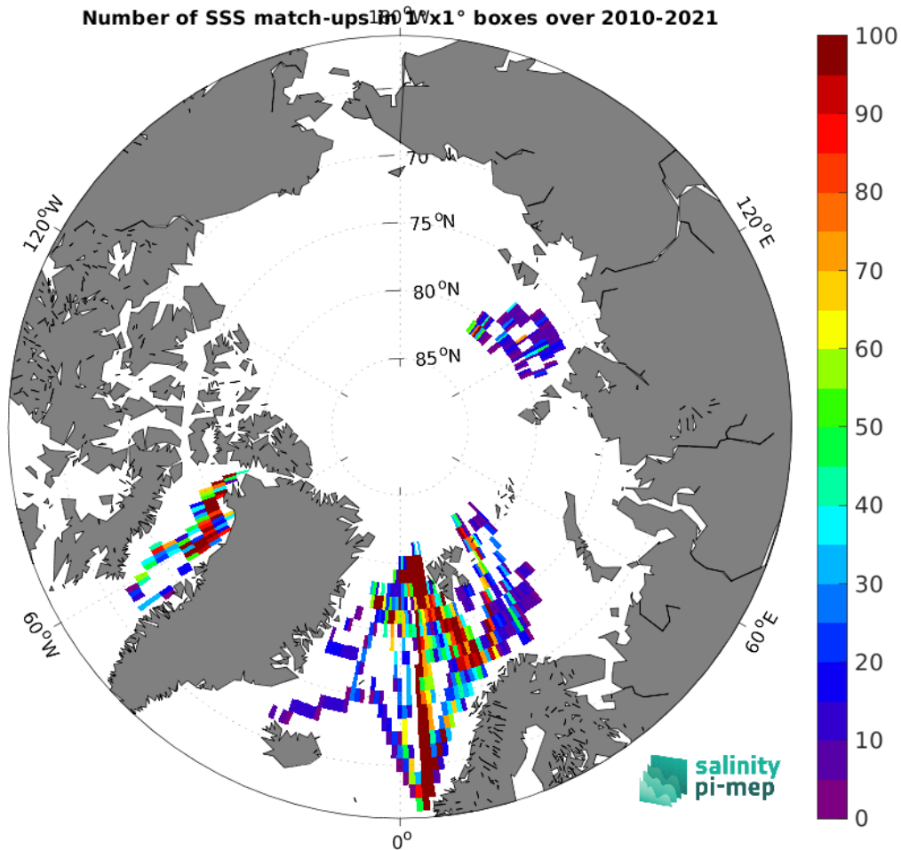
Figure 4: Number of SSS match-ups between TSG (Polarstern) SSS and the CCI SSS L4 Merged-OI v4.4 - 30-day running (ESA) SSS product for the Arctic Ocean Pi-MEP region over 1^\circ \times 1^\circ boxes and for the full satellite product period.
