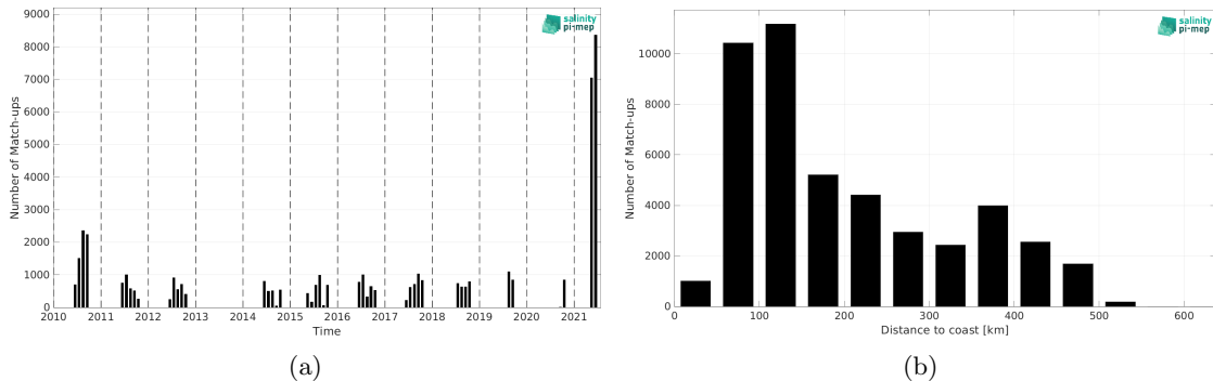
Figure 1: Number of match-ups between TSG (Polarstern) and CCI SSS L4 Merged-OI v4.4 - 30-day running (ESA) SSS as a function of time (a) and as function of the distance to coast (b) over the Arctic Ocean Pi-MEP region and for the full satellite product period.
