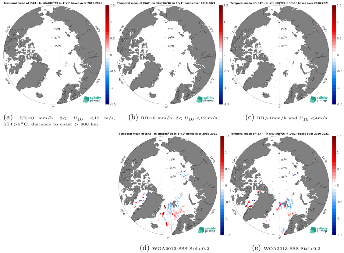
Figure 12: Temporal mean gridded over spatial boxes of size 1^{\circ}\times 1^{\circ} of \Delta\text{SSS} (CCI SSS L4 Merged-OI v4.4 - 30-day running (ESA) - TSG (Polarstern)) for 5 different subdatasets corresponding to:RR=0 mm/h, 3 < U_{10} < 12 m/s, SST >5^{\circ}\text{C} , distance to coast > 800 km (a), RR=0 mm/h, 3 < U_{10} < 12 m/s (b), RR >1 mm/h and U_{10} < 4 m/s (c), WOA2013 SSS Std <0.2 (d), WOA2013 SSS Std >0.2 (e).
