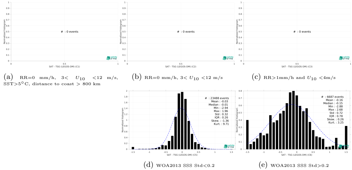
Figure 13: Normalized histogram of \Delta SSS (CCI SSS L4 Merged-OI v4.4 - 30-day running (ESA) - TSG (LEGOS-DM)) for 5 different subdatasets corresponding to: RR=0 mm/h, 3 < U_{10} < 12 m/s, SST > 5°C, distance to coast > 800 km (a), RR=0 mm/h, 3 < U_{10} < 12 m/s (b), RR > 1mm/h and U_{10} < 4 m/s (c), WOA2013 SSS Std < 0.2 (d), WOA2013 SSS Std > 0.2 (e).
