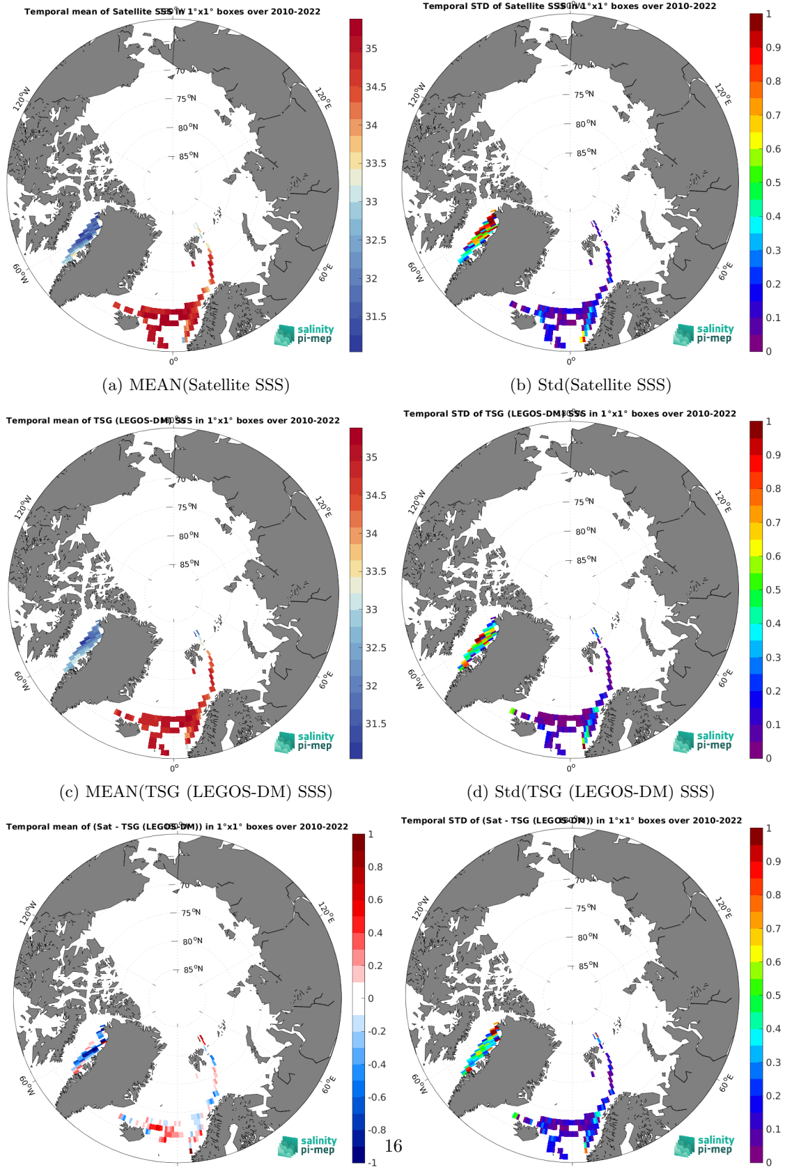
(e) MEAN( \Delta SSS) (Satellite - TSG (LEGOS-DM)) (f) Std( \Delta SSS) (Satellite - TSG (LEGOS-DM)) Figure 6: Temporal mean (left) and Std (right) of SSS from CCI SSS L4 Merged-OI v4.4 - 30-day running (ESA) (top), TSG (LEGOS-DM) (middle), and of \Delta SSS (Satellite - TSG (LEGOS-DM)). Only match-up pairs are used to generate these maps.
