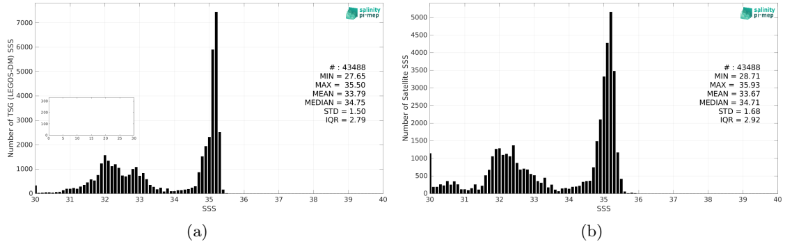
Figure 2: Histograms of SSS from TSG (LEGOS-DM) (a) and CCI SSS L4 Merged-OI v4.4 - 30-day running (ESA) (b) considering all match-up pairs per bins of 0.1 over the Arctic Ocean Pi-MEP region and for the full satellite product period.
