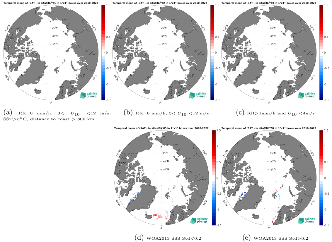
Figure 12: Temporal mean gridded over spatial boxes of size 1^{\circ}\times 1^{\circ} of \Delta\text{SSS} (CCI SSS L4 Merged-OI v4.4 - 30-day running (ESA) - TSG (LEGOS-DM)) for 5 different subdatasets corresponding to:RR=0 mm/h, 3 < U_{10} < 12 m/s, SST >5^{\circ}\text{C} , distance to coast > 800 km (a), RR=0 mm/h, 3 < U_{10} < 12 m/s (b), RR >1 mm/h and U_{10} < 4 m/s (c), WOA2013 SSS Std <0.2 (d), WOA2013 SSS Std >0.2 (e).
