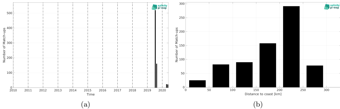
Figure 1: Number of match-ups between TSG (Lauge-Koch) and CCI SSS L4 Merged-OI v4.4 - 30-day running (ESA) SSS as a function of time (a) and as function of the distance to coast (b) over the Arctic Ocean Pi-MEP region and for the full satellite product period.
