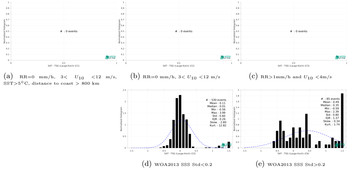
Figure 13: Normalized histogram of \Delta SSS (CCI SSS L4 Merged-OI v4.4 - 30-day running (ESA) - TSG (Lauge-Koch)) for 5 different subdatasets corresponding to: RR=0 mm/h, 3 < U_{10} < 12 m/s, SST>5°C, distance to coast > 800 km (a), RR=0 mm/h, 3 < U_{10} < 12 m/s (b), RR>1mm/h and U_{10} < 4 m/s (c), WOA2013 SSS Std<0.2 (d), WOA2013 SSS Std>0.2 (e).
