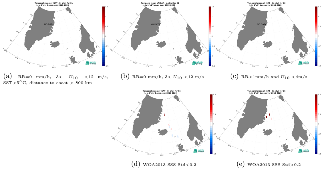
Figure 12: Temporal mean gridded over spatial boxes of size 1^{\circ}\times 1^{\circ} of \Delta\text{SSS} (CCI SSS L4 Merged-OI v4.4 - 30-day running (ESA) - TSG (Lauge-Koch)) for 5 different subdatasets corresponding to:RR=0 mm/h, 3 < U_{10} < 12 m/s, SST > 5^{\circ}\text{C} , distance to coast > 800 km (a), RR=0 mm/h, 3 < U_{10} < 12 m/s (b), RR > 1 mm/h and U_{10} < 4 m/s (c), WOA2013 SSS Std < 0.2 (d), WOA2013 SSS Std > 0.2 (e).
