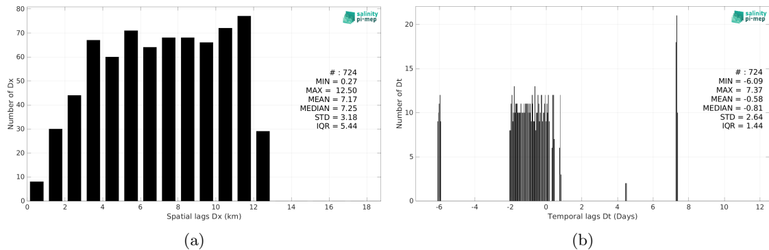
Figure 5: Histograms of the spatial (a) and temporal (b) lags between the location/time of the TSG (Lauge-Koch) measurement and the date of the corresponding CCI SSS L4 Merged-OI v4.4 - 30-day running (ESA) SSS pixel.
