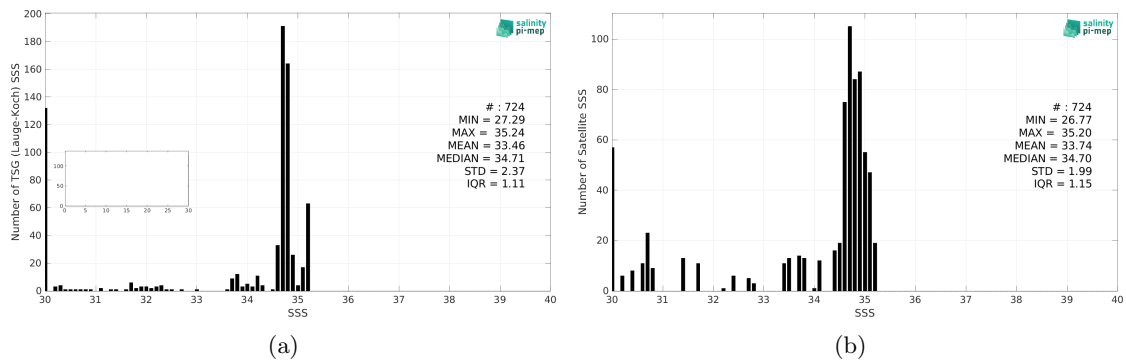
Figure 2: Histograms of SSS from TSG (Lauge-Koch) (a) and CCI SSS L4 Merged-OI v4.4 - 30-day running (ESA) (b) considering all match-up pairs per bins of 0.1 over the Arctic Ocean Pi-MEP region and for the full satellite product period.
