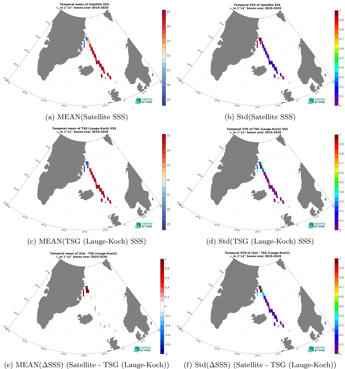
Figure 6: Temporal mean (left) and Std (right) of SSS from CCI SSS L4 Merged-OI v4.4 - 30-day running (ESA) (top), TSG (Lauge-Koch) (middle), and of \Delta SSS (Satellite - TSG (Lauge-Koch)). Only match-up pairs are used to generate these maps.
