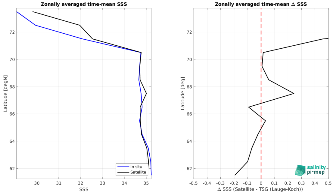
Figure 8: Left panel: Zonal mean SSS from CCI SSS L4 Merged-OI v4.4 - 30-day running (ESA) satellite product (black) and from TSG (Lauge-Koch) (blue). Right panel: Zonal mean of \Delta SSS (Satellite - TSG (Lauge-Koch)) for all the collected Pi-MEP match-up pairs estimated over the full satellite product period.
