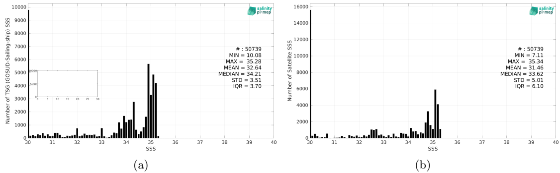
Figure 2: Histograms of SSS from TSG (GOSUD-Sailing-ship) (a) and CCI SSS L4 Merged-OI v4.4 - 30-day running (ESA) (b) considering all match-up pairs per bins of 0.1 over the Arctic Ocean Pi-MEP region and for the full satellite product period.
