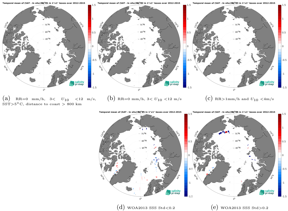
Figure 12: Temporal mean gridded over spatial boxes of size 1^\circ \times 1^\circ of \Delta SSS (CCI SSS L4 Merged-OI v4.4 - 30-day running (ESA) - TSG (GOSUD-Sailing-ship)) for 5 different subdatasets corresponding to: RR=0 mm/h, 3 < U_{10} < 12 m/s, SST > 5^\circ\text{C} , distance to coast > 800 km (a), RR=0 mm/h, 3 < U_{10} < 12 m/s (b), RR > 1 mm/h and U_{10} < 4 m/s (c), WOA2013 SSS Std < 0.2 (d), WOA2013 SSS Std > 0.2 (e).
