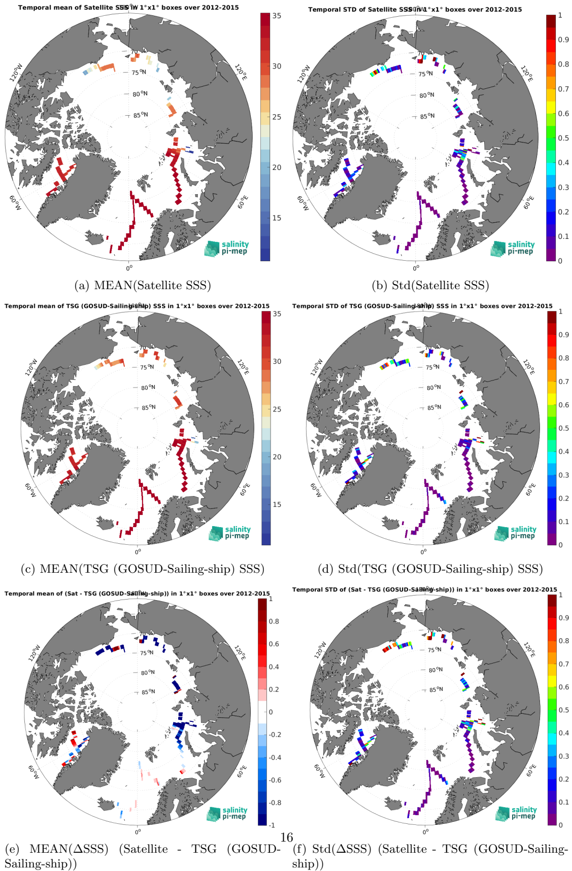
Figure 6: Temporal mean (left) and Std (right) of SSS from CCI SSS L4 Merged-OI v4.4 - 30-day running (ESA) (top), TSG (GOSUD-Sailing-ship) (middle), and of \Delta SSS (Satellite - TSG (GOSUD-Sailing-ship)). Only match-up pairs are used to generate these maps.
