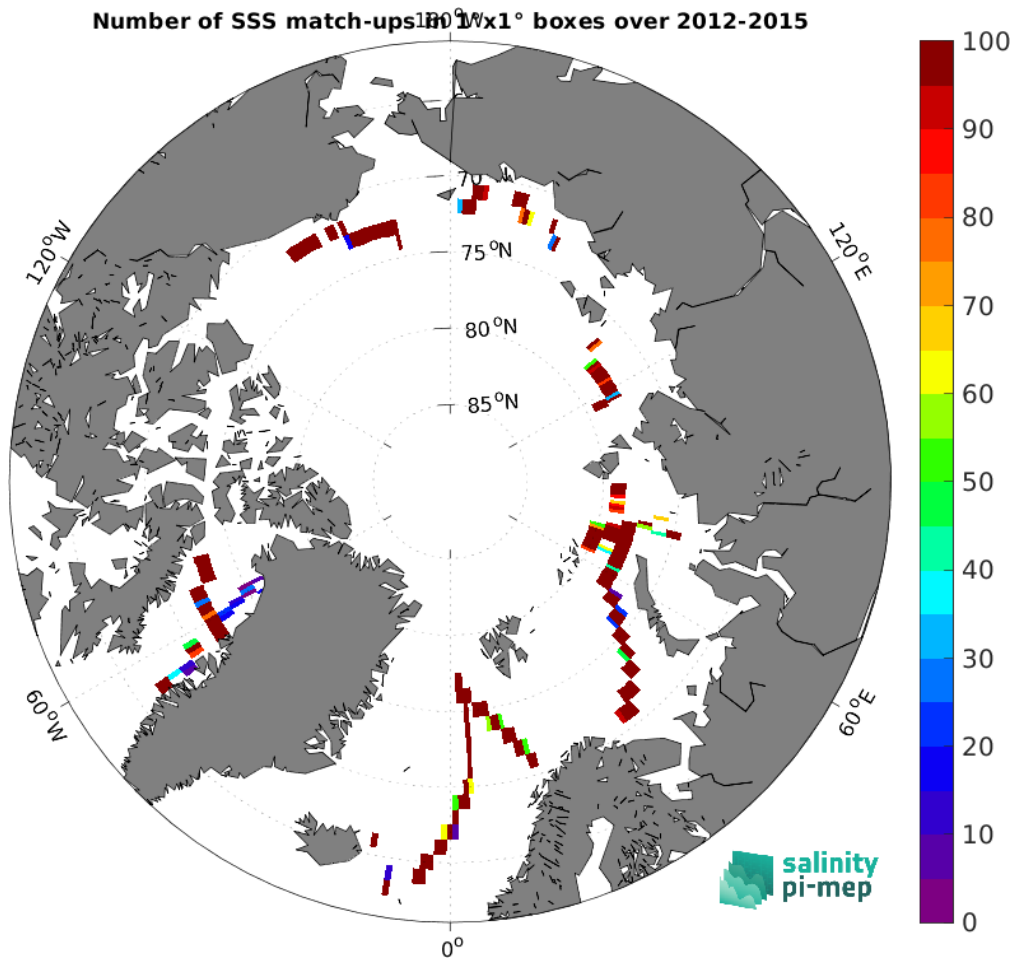
Figure 4: Number of SSS match-ups between TSG (GOSUD-Sailing-ship) SSS and the CCI SSS L4 Merged-OI v4.4 - 30-day running (ESA) SSS product for the Arctic Ocean Pi-MEP region over 1^\circ \times 1^\circ boxes and for the full satellite product period.
