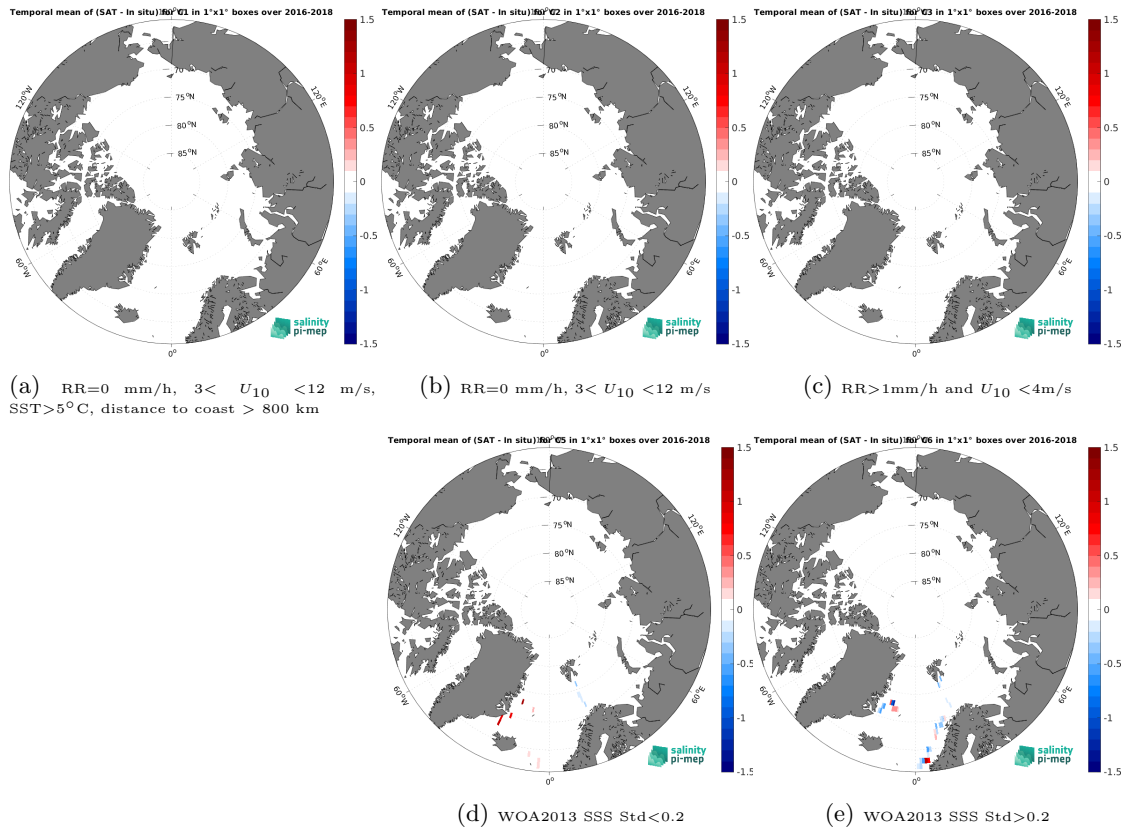
Figure 12: Temporal mean gridded over spatial boxes of size 1^\circ \times 1^\circ of \Delta SSS (CCI SSS L4 Merged-OI v4.4 - 30-day running (ESA) - TSG (GOSUD-Research-vessel)) for 5 different subdatasets corresponding to: RR=0 mm/h, 3 < U_{10} < 12 m/s, SST > 5^\circ\text{C} , distance to coast > 800 km (a), RR=0 mm/h, 3 < U_{10} < 12 m/s (b), RR > 1 mm/h and U_{10} < 4 m/s (c), WOA2013 SSS Std < 0.2 (d), WOA2013 SSS Std > 0.2 (e).
