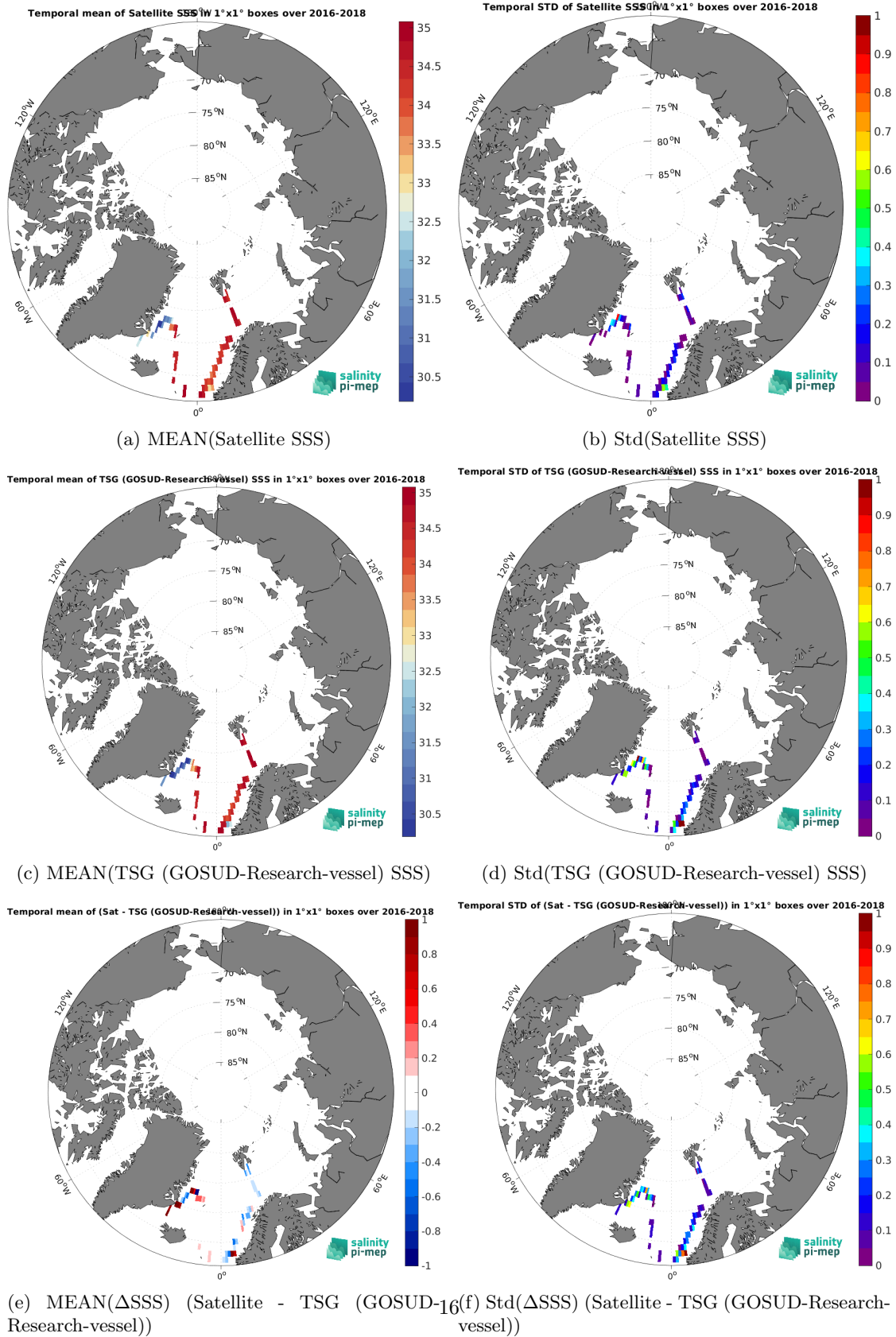
Figure 6: Temporal mean (left) and Std (right) of SSS from CCI SSS L4 Merged-OI v4.4 - 30-day running (ESA) (top), TSG (GOSUD-Research-vessel) (middle), and of \Delta SSS (Satellite - TSG (GOSUD-Research-vessel)). Only match-up pairs are used to generate these maps.
