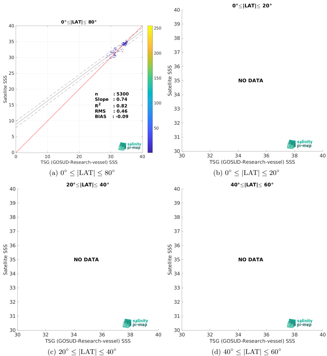
Figure 9: Contour maps of the concentration of CCI SSS L4 Merged-OI v4.4 - 30-day running (ESA) SSS (y-axis) versus TSG (GOSUD-Research-vessel) SSS (x-axis) at match-up pairs for different latitude bands. For each plot, the red line shows x=y . The black thin and dashed lines indicate a linear fit through the data cloud and the \pm 95\% confidence levels, respectively. The number match-up pairs n , the slope and R^2 coefficient of the linear fit, the root mean square (RMS) and the mean bias between satellite and in situ data are indicated for each latitude band in each plots.
