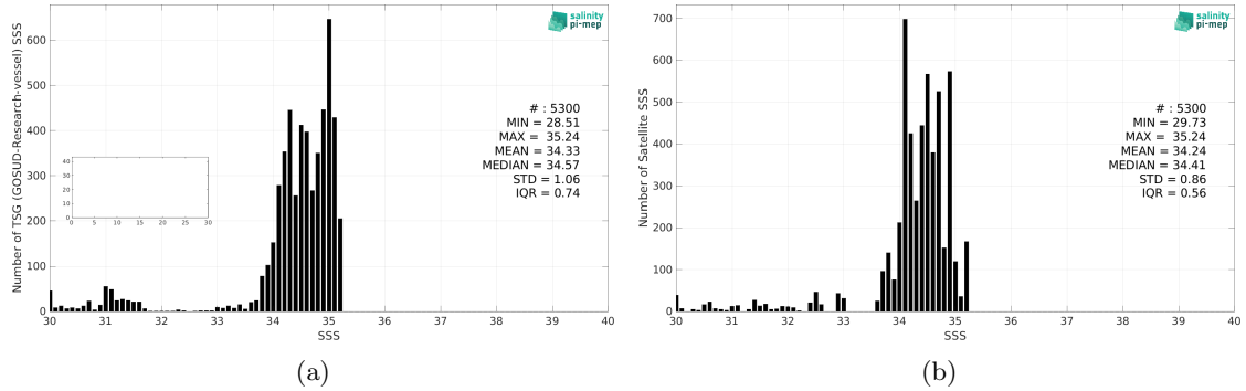
Figure 2: Histograms of SSS from TSG (GOSUD-Research-vessel) (a) and CCI SSS L4 Merged-OI v4.4 - 30-day running (ESA) (b) considering all match-up pairs per bins of 0.1 over the Arctic Ocean Pi-MEP region and for the full satellite product period.
