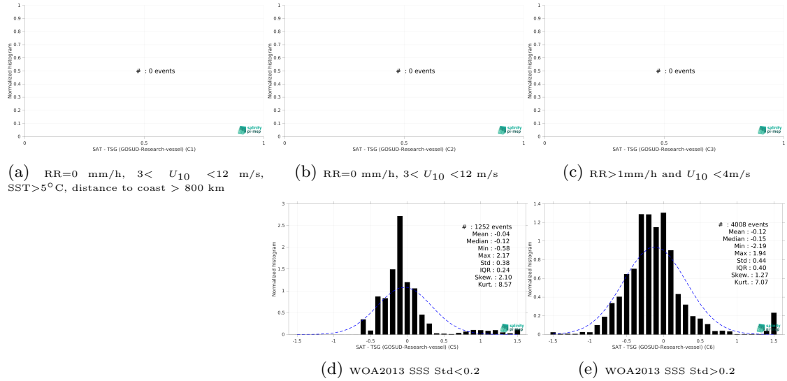
Figure 13: Normalized histogram of \Delta SSS (CCI SSS L4 Merged-OI v4.4 - 30-day running (ESA) - TSG (GOSUD-Research-vessel)) for 5 different subdatasets corresponding to: RR=0 mm/h, 3 < U_{10} < 12 m/s, SST > 5°C, distance to coast > 800 km (a), RR=0 mm/h, 3 < U_{10} < 12 m/s (b), RR > 1mm/h and U_{10} < 4 m/s (c), WOA2013 SSS Std < 0.2 (d), WOA2013 SSS Std > 0.2 (e).
