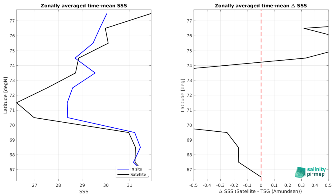
Figure 8: Left panel: Zonal mean SSS from CCI SSS L4 Merged-OI v4.4 - 30-day running (ESA) satellite product (black) and from TSG (Amundsen) (blue). Right panel: Zonal mean of \Delta SSS (Satellite - TSG (Amundsen)) for all the collected Pi-MEP match-up pairs estimated over the full satellite product period.
