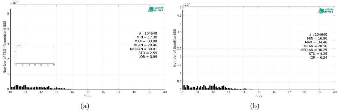
Figure 2: Histograms of SSS from TSG (Amundsen) (a) and CCI SSS L4 Merged-OI v4.4 - 30-day running (ESA) (b) considering all match-up pairs per bins of 0.1 over the Arctic Ocean Pi-MEP region and for the full satellite product period.
