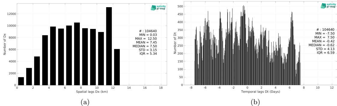
Figure 5: Histograms of the spatial (a) and temporal (b) lags between the location/time of the TSG (Amundsen) measurement and the date of the corresponding CCI SSS L4 Merged-OI v4.4 - 30-day running (ESA) SSS pixel.
