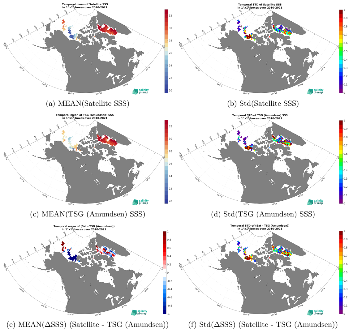
Figure 6: Temporal mean (left) and Std (right) of SSS from CCI SSS L4 Merged-OI v4.4 - 30-day running (ESA) (top), TSG (Amundsen) (middle), and of \Delta SSS (Satellite - TSG (Amundsen)). Only match-up pairs are used to generate these maps.
