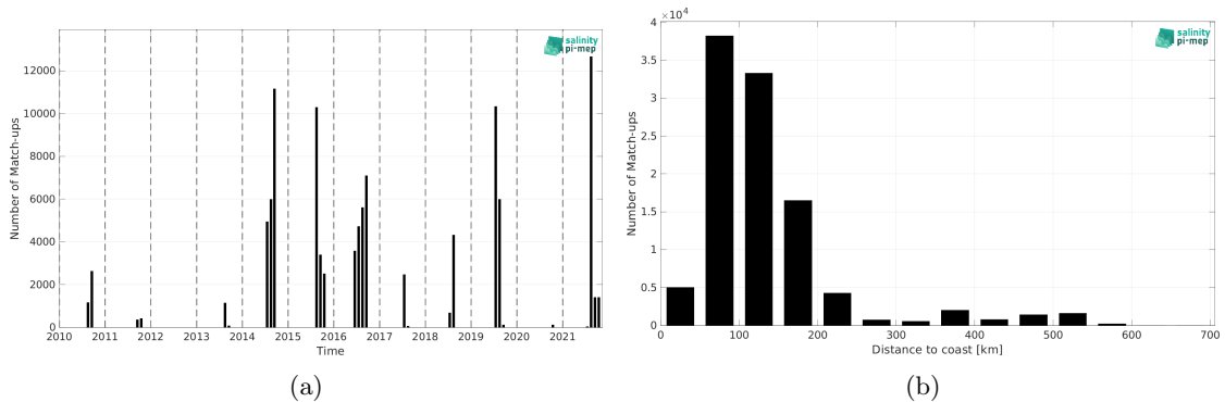
Figure 1: Number of match-ups between TSG (Amundsen) and CCI SSS L4 Merged-OI v4.4 - 30-day running (ESA) SSS as a function of time (a) and as function of the distance to coast (b) over the Arctic Ocean Pi-MEP region and for the full satellite product period.
