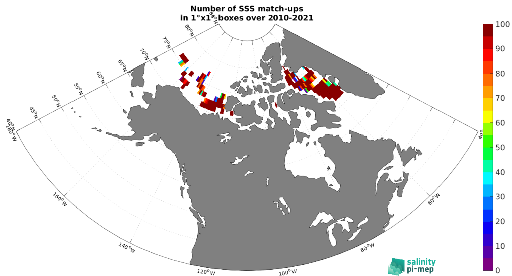
Figure 4: Number of SSS match-ups between TSG (Amundsen) SSS and the CCI SSS L4 Merged-OI v4.4 - 30-day running (ESA) SSS product for the Arctic Ocean Pi-MEP region over 1°x1° boxes and for the full satellite product period.
