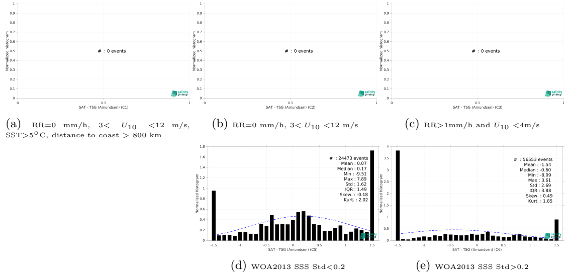
Figure 13: Normalized histogram of \Delta SSS (CCI SSS L4 Merged-OI v4.4 - 30-day running (ESA) - TSG (Amundsen)) for 5 different subdatasets corresponding to: RR=0 mm/h, 3 < U_{10} < 12 m/s, SST > 5°C, distance to coast > 800 km (a), RR=0 mm/h, 3 < U_{10} < 12 m/s (b), RR > 1mm/h and U_{10} < 4 m/s (c), WOA2013 SSS Std < 0.2 (d), WOA2013 SSS Std > 0.2 (e).
