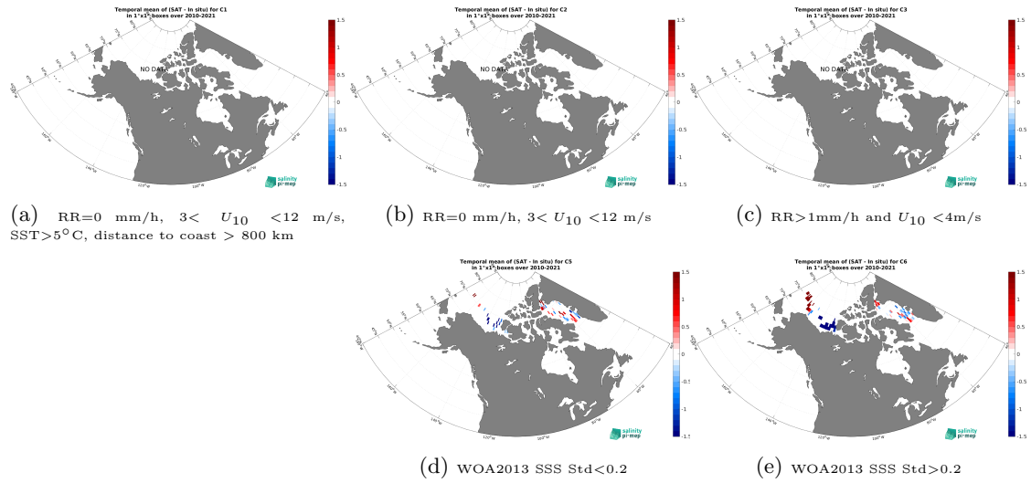
Figure 12: Temporal mean gridded over spatial boxes of size 1^{\circ}\times 1^{\circ} of \Delta\text{SSS} (CCI SSS L4 Merged-OI v4.4 - 30-day running (ESA) - TSG (Amundsen)) for 5 different subdatasets corresponding to:RR=0 mm/h, 3 < U_{10} < 12 m/s, SST > 5^{\circ}\text{C} , distance to coast > 800 km (a), RR=0 mm/h, 3 < U_{10} < 12 m/s (b), RR > 1 mm/h and U_{10} < 4 m/s (c), WOA2013 SSS Std < 0.2 (d), WOA2013 SSS Std > 0.2 (e).
