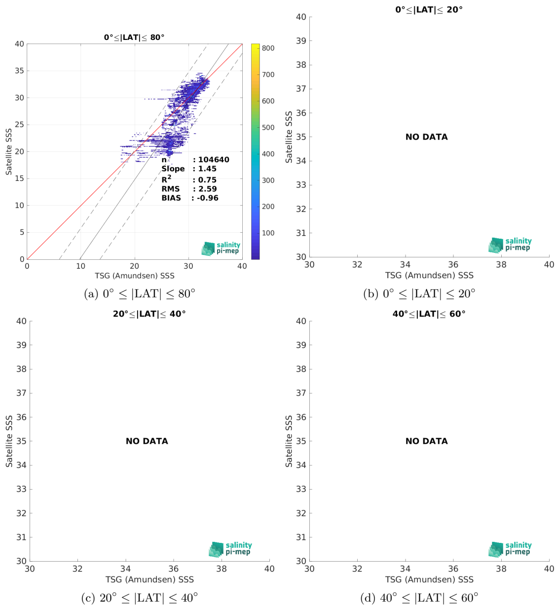
Figure 9: Contour maps of the concentration of CCI SSS L4 Merged-OI v4.4 - 30-day running (ESA) SSS (y-axis) versus TSG (Amundsen) SSS (x-axis) at match-up pairs for different latitude bands. For each plot, the red line shows x=y . The black thin and dashed lines indicate a linear fit through the data cloud and the \pm 95\% confidence levels, respectively. The number match-up pairs n , the slope and R^2 coefficient of the linear fit, the root mean square (RMS) and the mean bias between satellite and in situ data are indicated for each latitude band in each plots.
