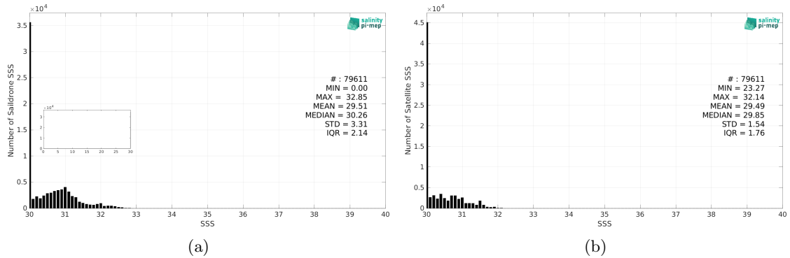
Figure 2: Histograms of SSS from Sairdrone (a) and CCI SSS L4 Merged-OI v4.4 - 30-day running (ESA) (b) considering all match-up pairs per bins of 0.1 over the Arctic Ocean Pi-MEP region and for the full satellite product period.
