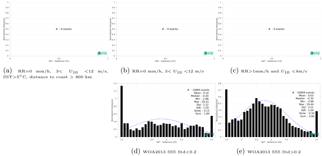
Figure 13: Normalized histogram of \Delta SSS (CCI SSS L4 Merged-OI v4.4 - 30-day running (ESA) - Saldrone) for 5 different subdatasets corresponding to: RR=0 mm/h, 3 < U_{10} < 12 m/s, SST>5°C, distance to coast > 800 km (a), RR=0 mm/h, 3 < U_{10} < 12 m/s (b), RR>1mm/h and U_{10} < 4 m/s (c), WOA2013 SSS Std<0.2 (d), WOA2013 SSS Std>0.2 (e).
