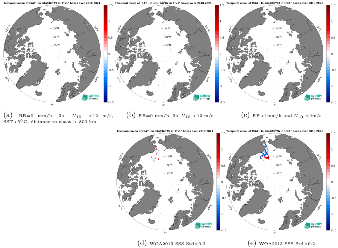
Figure 12: Temporal mean gridded over spatial boxes of size 1^{\circ}\times 1^{\circ} of \Delta\text{SSS} (CCI SSS L4 Merged-OI v4.4 - 30-day running (ESA) - Saildrone) for 5 different subdatasets corresponding to: RR=0 mm/h, 3 < U_{10} < 12 m/s, SST > 5^{\circ}\text{C} , distance to coast > 800 km (a), RR=0 mm/h, 3 < U_{10} < 12 m/s (b), RR > 1 mm/h and U_{10} < 4 m/s (c), WOA2013 SSS Std < 0.2 (d), WOA2013 SSS Std > 0.2 (e).
