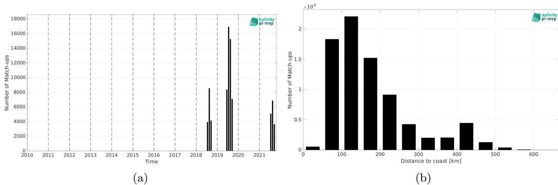
Figure 1: Number of match-ups between Saildrone and CCI SSS L4 Merged-OI v4.4 - 30-day running (ESA) SSS as a function of time (a) and as function of the distance to coast (b) over the Arctic Ocean Pi-MEP region and for the full satellite product period.
