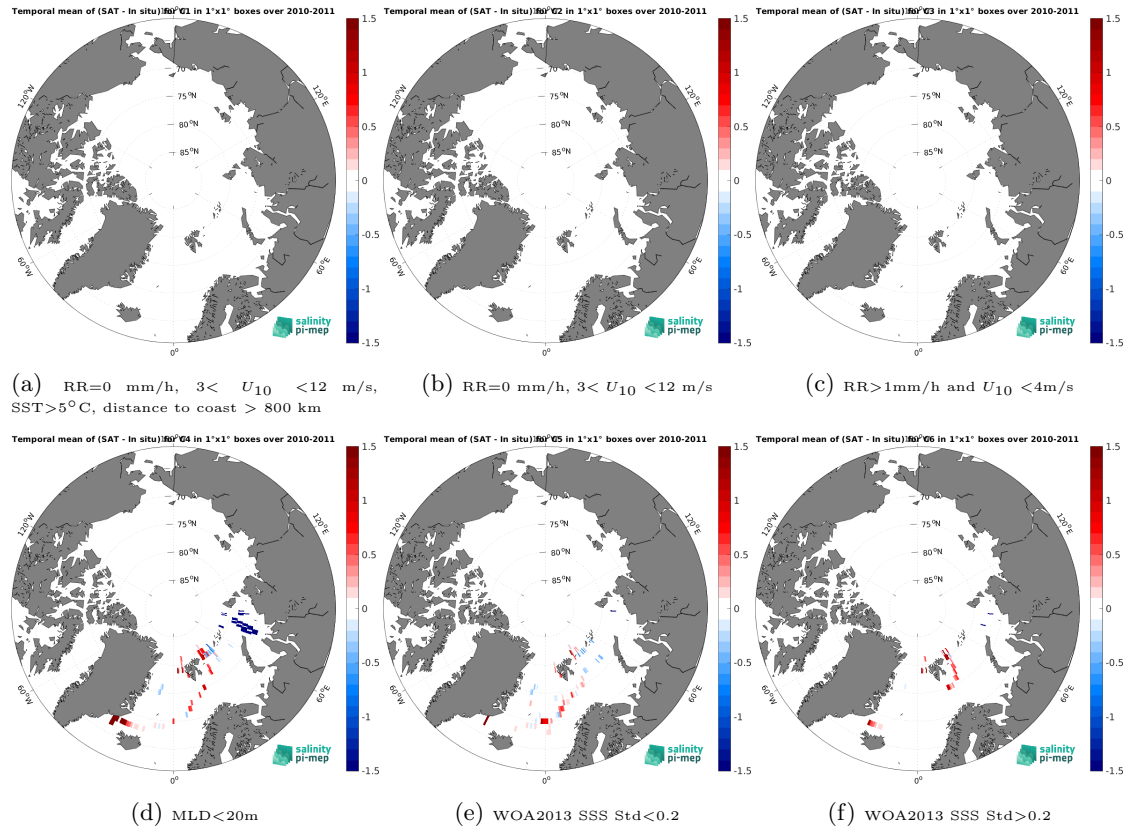
Figure 12: Temporal mean gridded over spatial boxes of size 1^{\circ}\times 1^{\circ} of \Delta\text{SSS} (CCI SSS L4 Merged-OI v4.4 - 30-day running (ESA) - Marine mammals) for 6 different subdatasets corresponding to: RR=0 mm/h, 3 < U_{10} < 12 m/s, SST > 5^{\circ}\text{C} , distance to coast > 800 km (a), RR=0 mm/h, 3 < U_{10} < 12 m/s (b), RR > 1 mm/h and U_{10} < 4 m/s (c), MLD < 20 m (d), WOA2013 SSS Std < 0.2 (e), WOA2013 SSS Std > 0.2 (f).
