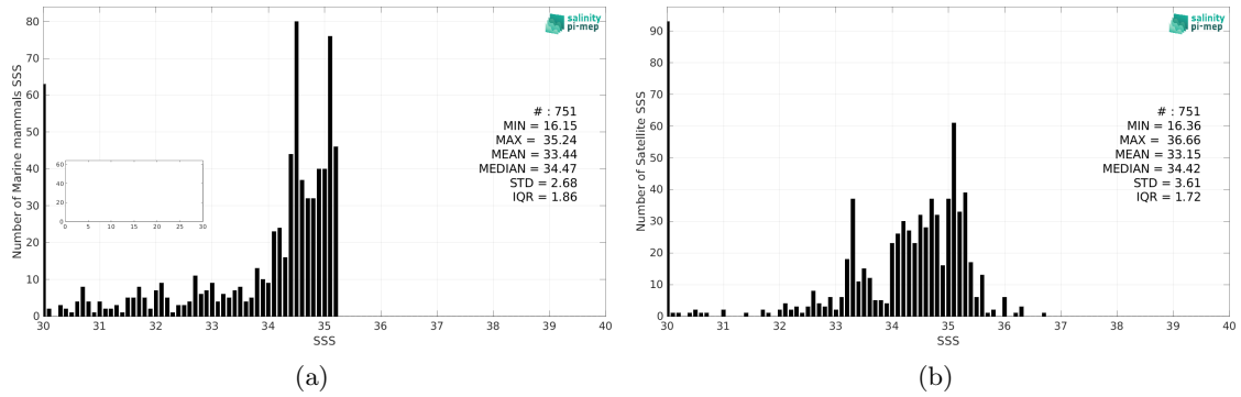
Figure 2: Histograms of SSS from Marine mammals (a) and CCI SSS L4 Merged-OI v4.4 - 30-day running (ESA) (b) considering all match-up pairs per bins of 0.1 over the Arctic Ocean Pi-MEP region and for the full satellite product period.
