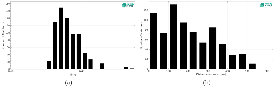
Figure 1: Number of match-ups between Marine mammals and CCI SSS L4 Merged-OI v4.4 - 30-day running (ESA) SSS as a function of time (a) and as function of the distance to coast (b) over the Arctic Ocean Pi-MEP region and for the full satellite product period.
