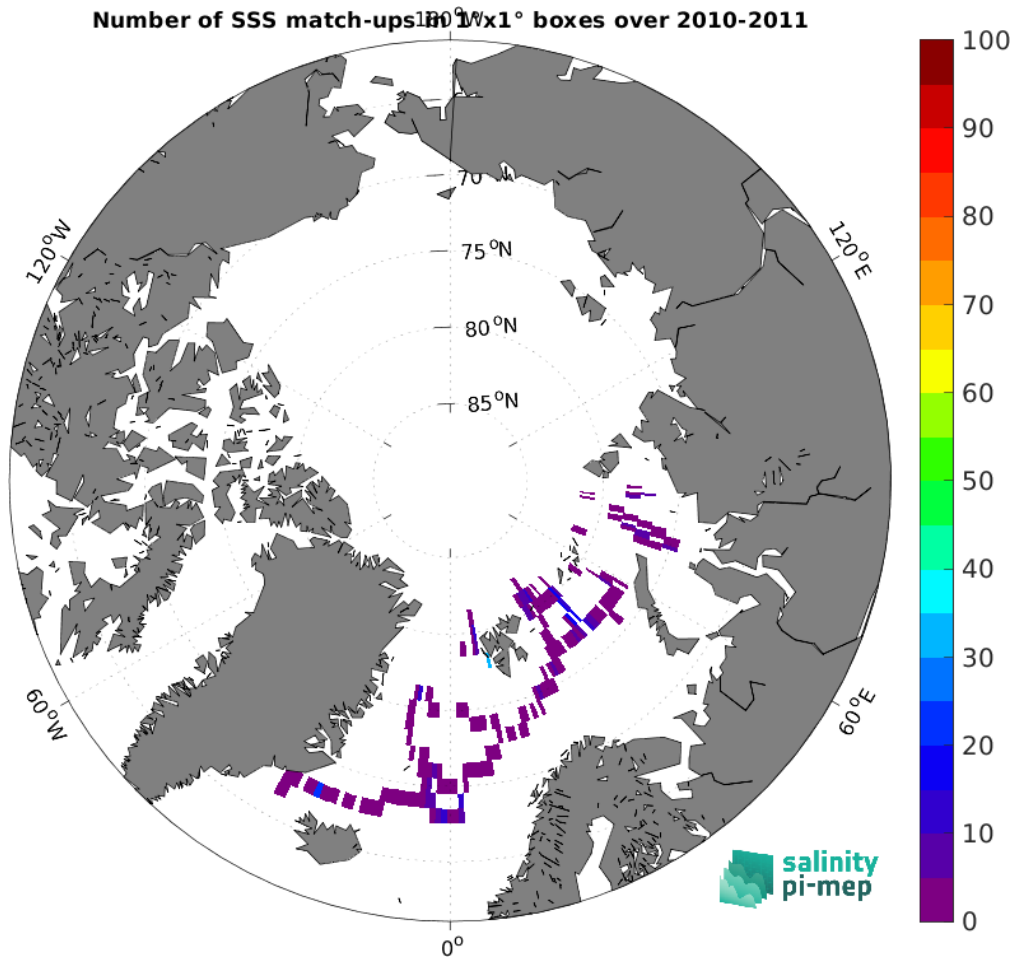
Figure 4: Number of SSS match-ups between Marine mammals SSS and the CCI SSS L4 Merged-OI v4.4 - 30-day running (ESA) SSS product for the Arctic Ocean Pi-MEP region over 1^\circ \times 1^\circ boxes and for the full satellite product period.
