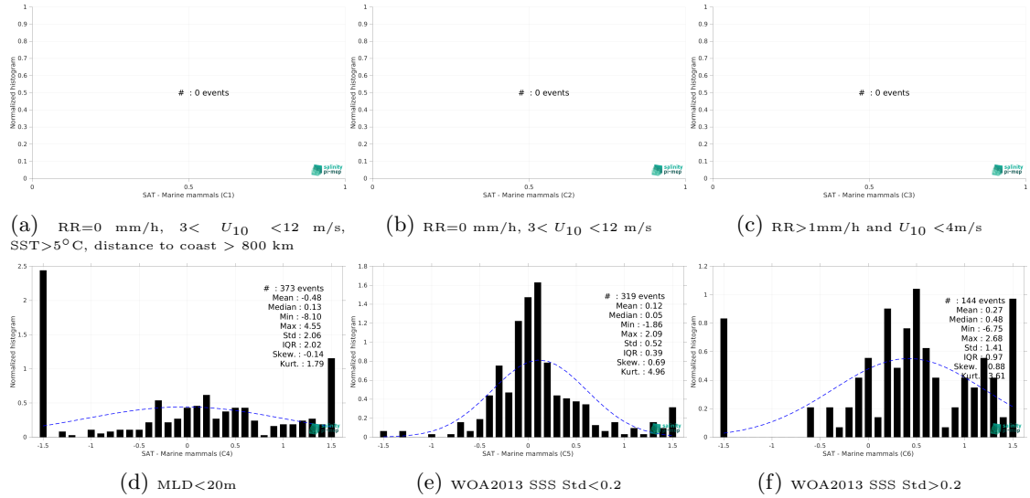
Figure 13: Normalized histogram of \Delta SSS (CCI SSS L4 Merged-OI v4.4 - 30-day running (ESA) - Marine mammals) for 6 different subdatasets corresponding to: RR=0 mm/h, 3 < U_{10} < 12 m/s, SST > 5°C, distance to coast > 800 km (a), RR=0 mm/h, 3 < U_{10} < 12 m/s (b), RR > 1mm/h and U_{10} < 4 m/s (c), MLD < 20m (d), WOA2013 SSS Std < 0.2 (e), WOA2013 SSS Std > 0.2 (f).
