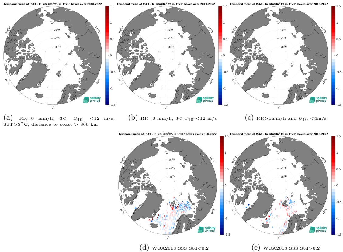
Figure 12: Temporal mean gridded over spatial boxes of size 1^{\circ}\times 1^{\circ} of \Delta\text{SSS} (CCI SSS L4 Merged-OI v4.4 - 30-day running (ESA) - ICES) for 5 different subdatasets corresponding to:RR=0 mm/h, 3 < U_{10} < 12 m/s, SST >5^{\circ}\text{C} , distance to coast > 800 km (a), RR=0 mm/h, 3 < U_{10} < 12 m/s (b), RR >1 mm/h and U_{10} < 4 m/s (c), WOA2013 SSS Std <0.2 (d), WOA2013 SSS Std >0.2 (e).
