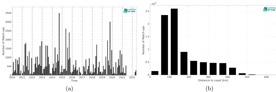
Figure 1: Number of match-ups between ICES and CCI SSS L4 Merged-OI v4.4 - 30-day running (ESA) SSS as a function of time (a) and as function of the distance to coast (b) over the Arctic Ocean Pi-MEP region and for the full satellite product period.
