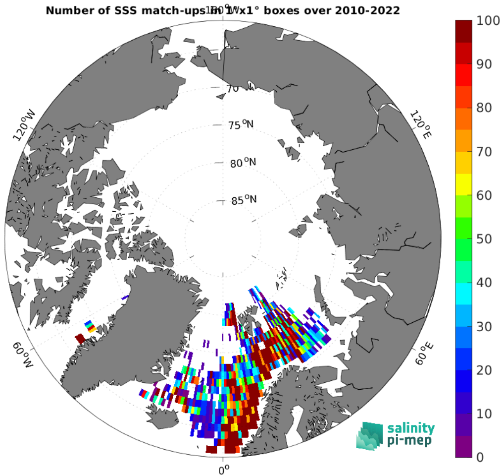
Figure 4: Number of SSS match-ups between ICES SSS and the CCI SSS L4 Merged-OI v4.4 - 30-day running (ESA) SSS product for the Arctic Ocean Pi-MEP region over 1^\circ \times 1^\circ boxes and for the full satellite product period.
