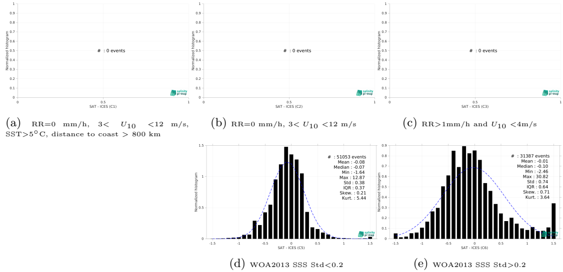
Figure 13: Normalized histogram of \Delta SSS (CCI SSS L4 Merged-OI v4.4 - 30-day running (ESA) - ICES) for 5 different subdatasets corresponding to: RR=0 mm/h, 3 < U_{10} < 12 m/s, SST>5°C, distance to coast > 800 km (a), RR=0 mm/h, 3 < U_{10} < 12 m/s (b), RR>1mm/h and U_{10} < 4 m/s (c), WOA2013 SSS Std<0.2 (d), WOA2013 SSS Std>0.2 (e).
