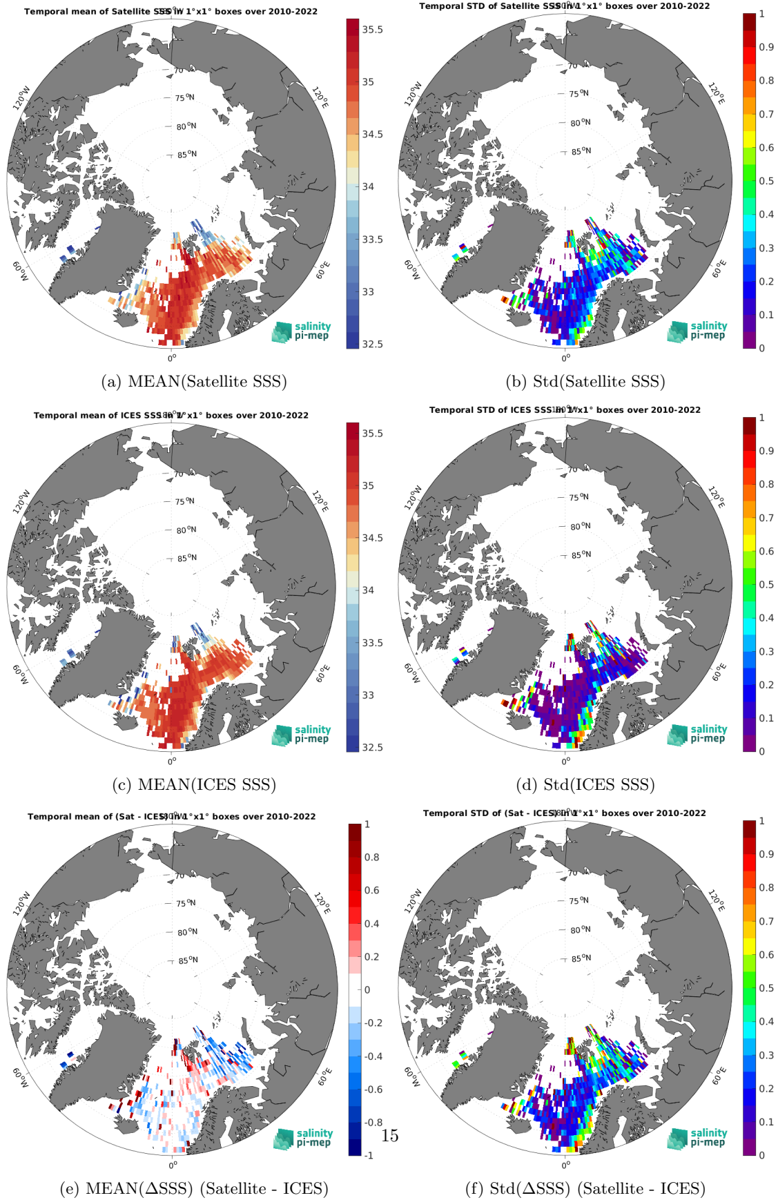
Figure 6: Temporal mean (left) and Std (right) of SSS from CCI SSS L4 Merged-OI v4.4 - 30-day running (ESA) (top), ICES (middle), and of \Delta SSS (Satellite - ICES). Only match-up pairs are used to generate these maps.
