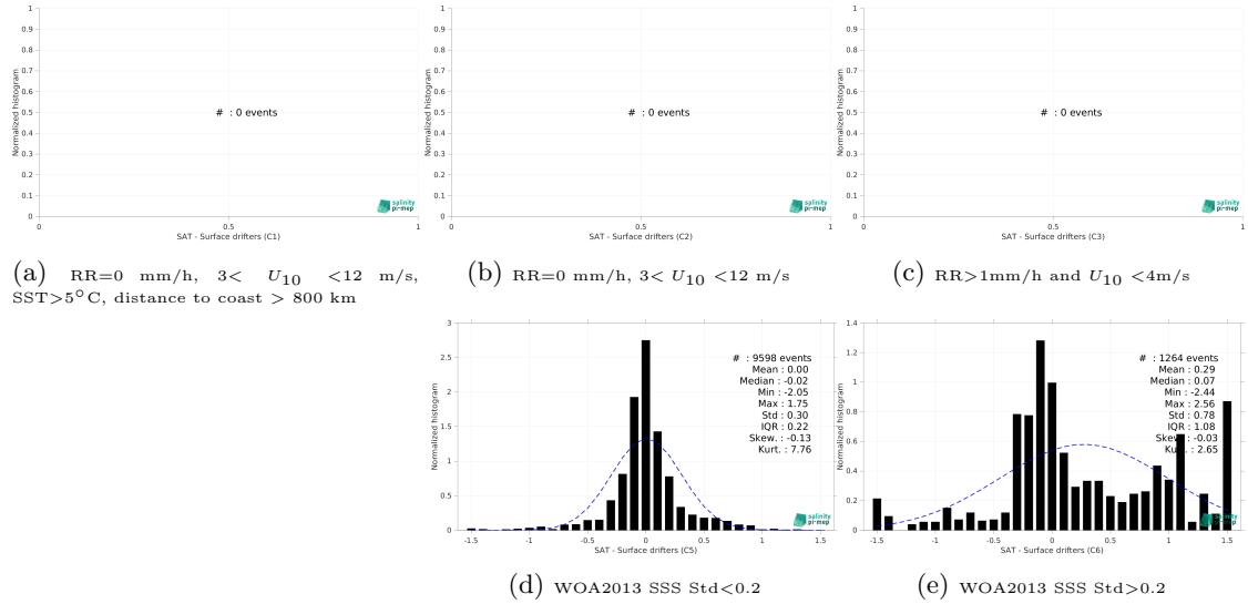
Figure 12: Normalized histogram of \Delta SSS (CCI SSS L4 Merged-OI v4.4 - 30-day running (ESA) - Surface drifters) for 5 different subdatasets corresponding to: RR=0 mm/h, 3 < U_{10} < 12 m/s, SST > 5°C, distance to coast > 800 km (a), RR=0 mm/h, 3 < U_{10} < 12 m/s (b), RR > 1mm/h and U_{10} < 4 m/s (c), WOA2013 SSS Std < 0.2 (d), WOA2013 SSS Std > 0.2 (e).
