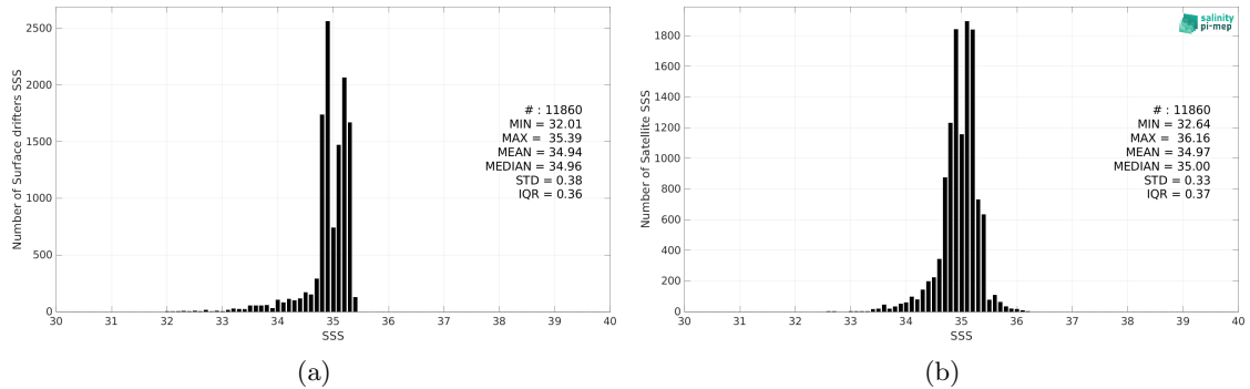
Figure 2: Histograms of SSS from Surface drifters (a) and CCI SSS L4 Merged-OI v4.4 - 30-day running (ESA) (b) considering all match-up pairs per bins of 0.1 over the Arctic Ocean Pi-MEP region and for the full satellite product period.
