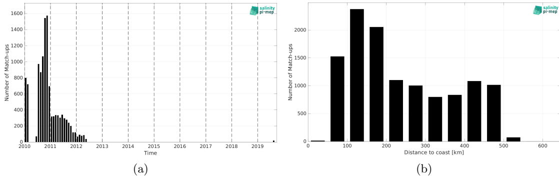
Figure 1: Number of match-ups between Surface drifters and CCI SSS L4 Merged-OI v4.4 - 30-day running (ESA) SSS as a function of time (a) and as function of the distance to coast (b) over the Arctic Ocean Pi-MEP region and for the full satellite product period.
