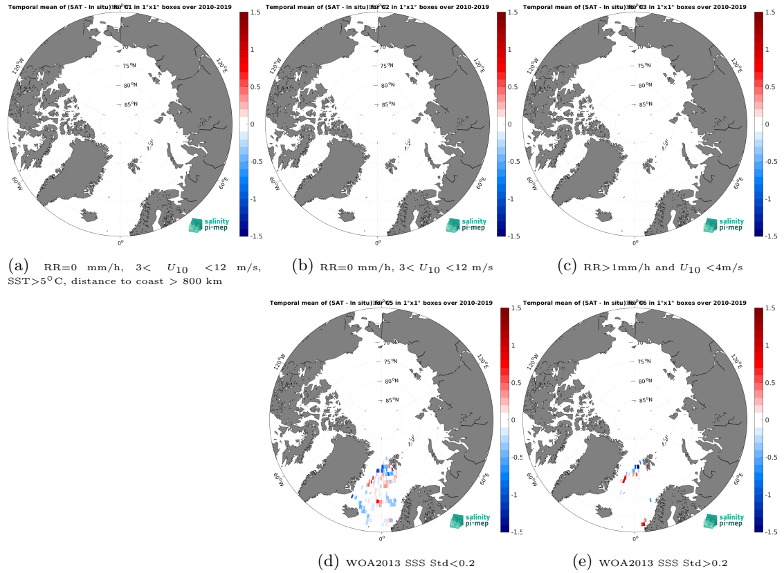
Figure 11: Temporal mean gridded over spatial boxes of size 1^{\circ}\times 1^{\circ} of \Delta\text{SSS} (CCI SSS L4 Merged-OI v4.4 - 30-day running (ESA) - Surface drifters) for 5 different subdatasets corresponding to: RR=0 mm/h, 3 < U_{10} < 12 m/s, SST > 5^{\circ}\text{C} , distance to coast > 800 km (a), RR=0 mm/h, 3 < U_{10} < 12 m/s (b), RR > 1 mm/h and U_{10} < 4 m/s (c), WOA2013 SSS Std < 0.2 (d), WOA2013 SSS Std > 0.2 (e).
