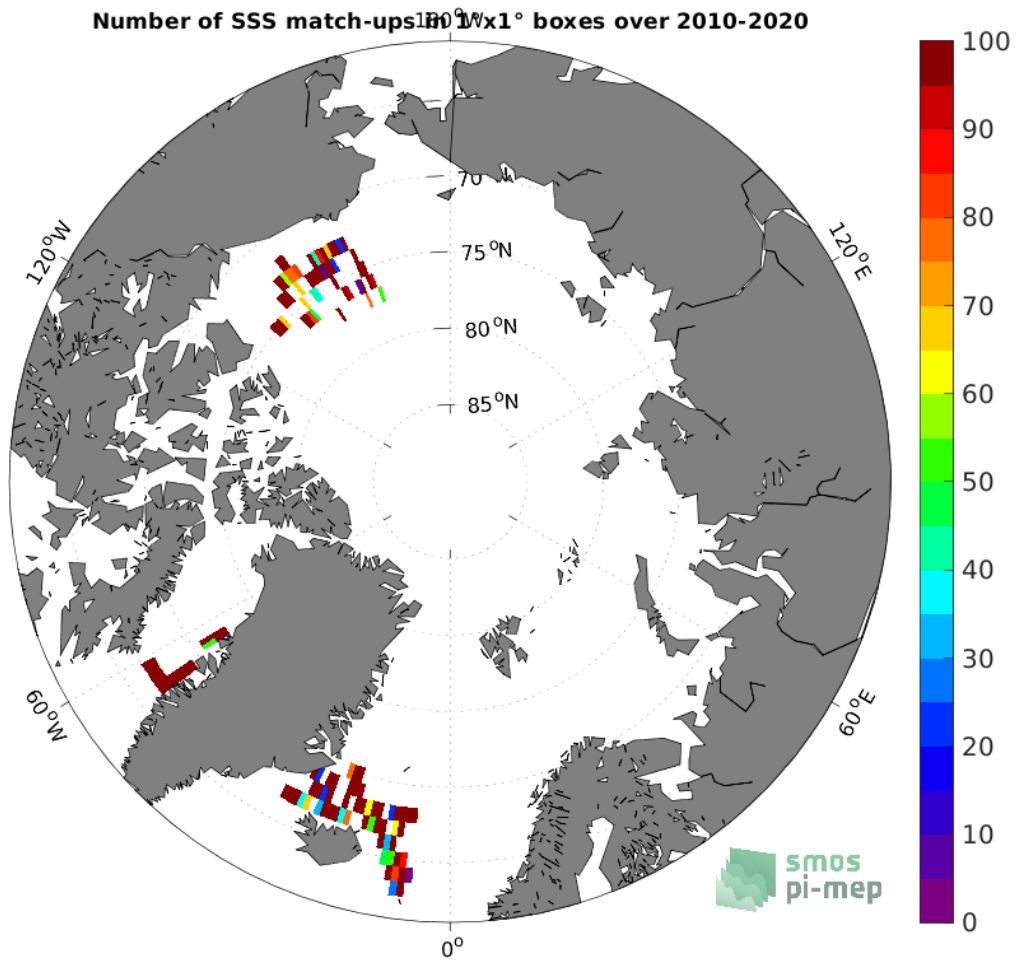
Figure 4: Number of SSS match-ups between TSG (SAMOS) SSS and the CCI SSS L4 Merged-OI v3.2 - 7-day running (ESA) SSS product for the Arctic Ocean Pi-MEP region over 1^\circ \times 1^\circ boxes and for the full satellite product period.
