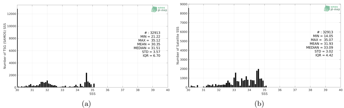
Figure 2: Histograms of SSS from TSG (SAMOS) (a) and CCI SSS L4 Merged-OI v3.2 - 7-day running (ESA) (b) considering all match-up pairs per bins of 0.1 over the Arctic Ocean Pi-MEP region and for the full satellite product period.
