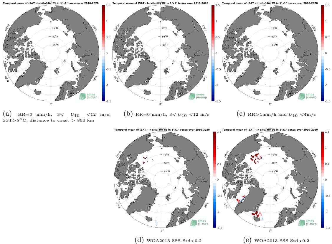
Figure 12: Temporal mean gridded over spatial boxes of size 1^{\circ}\times 1^{\circ} of \Delta\text{SSS} (CCI SSS L4 Merged-OI v3.2 - 7-day running (ESA) - TSG (SAMOS)) for 5 different subdatasets corresponding to:RR=0 mm/h, 3 < U_{10} < 12 m/s, SST >5^{\circ}\text{C} , distance to coast > 800 km (a), RR=0 mm/h, 3 < U_{10} < 12 m/s (b), RR >1 mm/h and U_{10} < 4 m/s (c), WOA2013 SSS Std <0.2 (d), WOA2013 SSS Std >0.2 (e).
