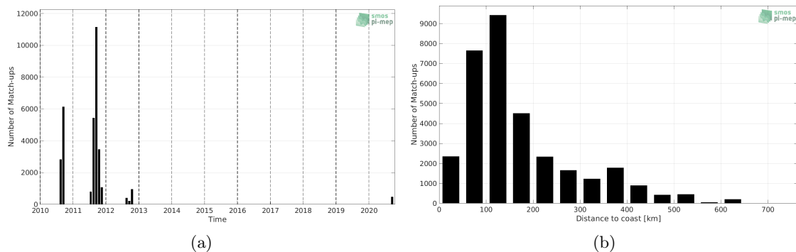
Figure 1: Number of match-ups between TSG (SAMOS) and CCI SSS L4 Merged-OI v3.2 - 7-day running (ESA) SSS as a function of time (a) and as function of the distance to coast (b) over the Arctic Ocean Pi-MEP region and for the full satellite product period.
