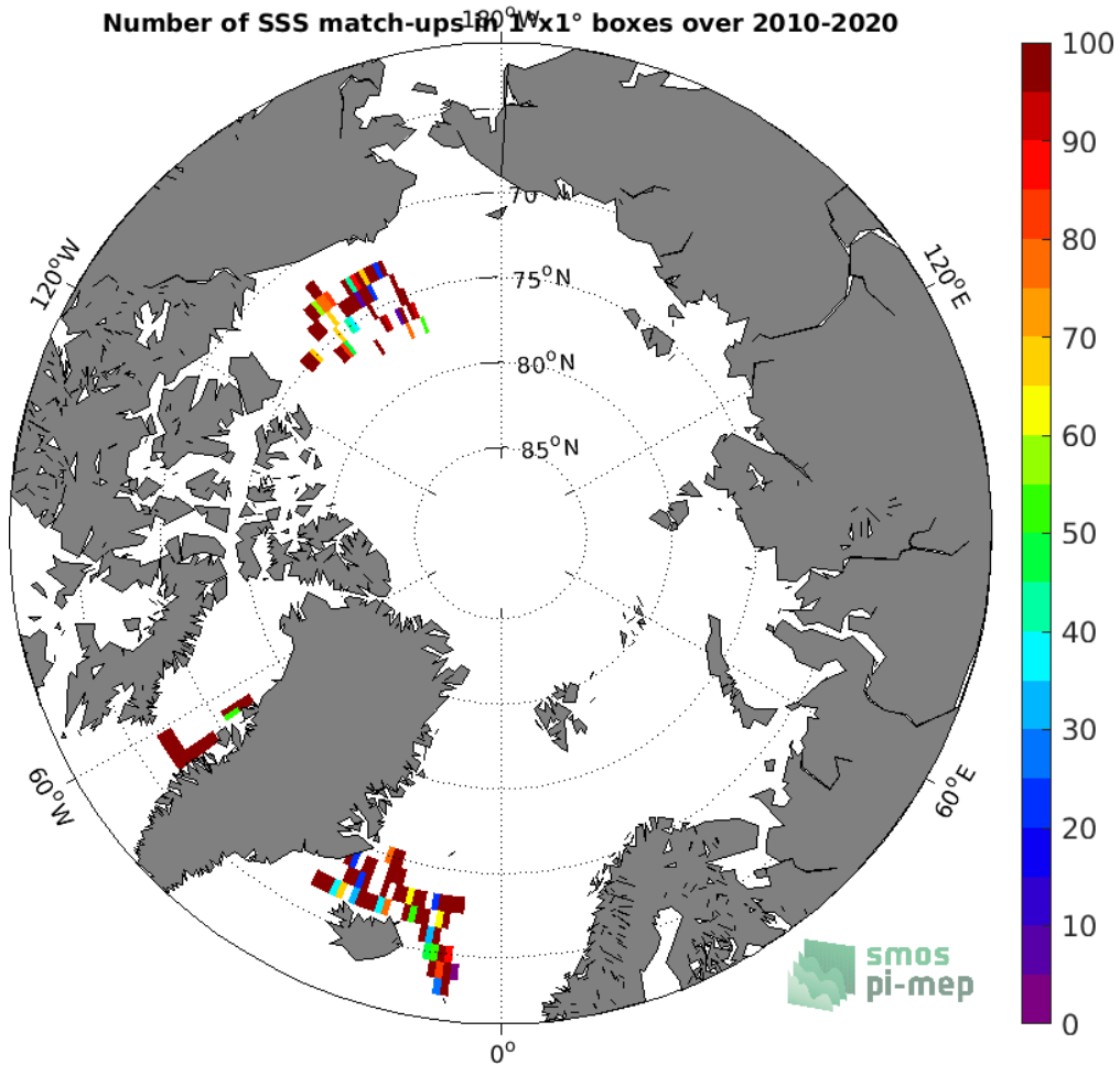
Figure 4: Number of SSS match-ups between TSG (SAMOS) SSS and the CCI SSS L4 Merged-OI v3.2 - 7-day running (ESA) SSS product for the Arctic Ocean Pi-MEP region over 1°x1° boxes and for the full satellite product period.
