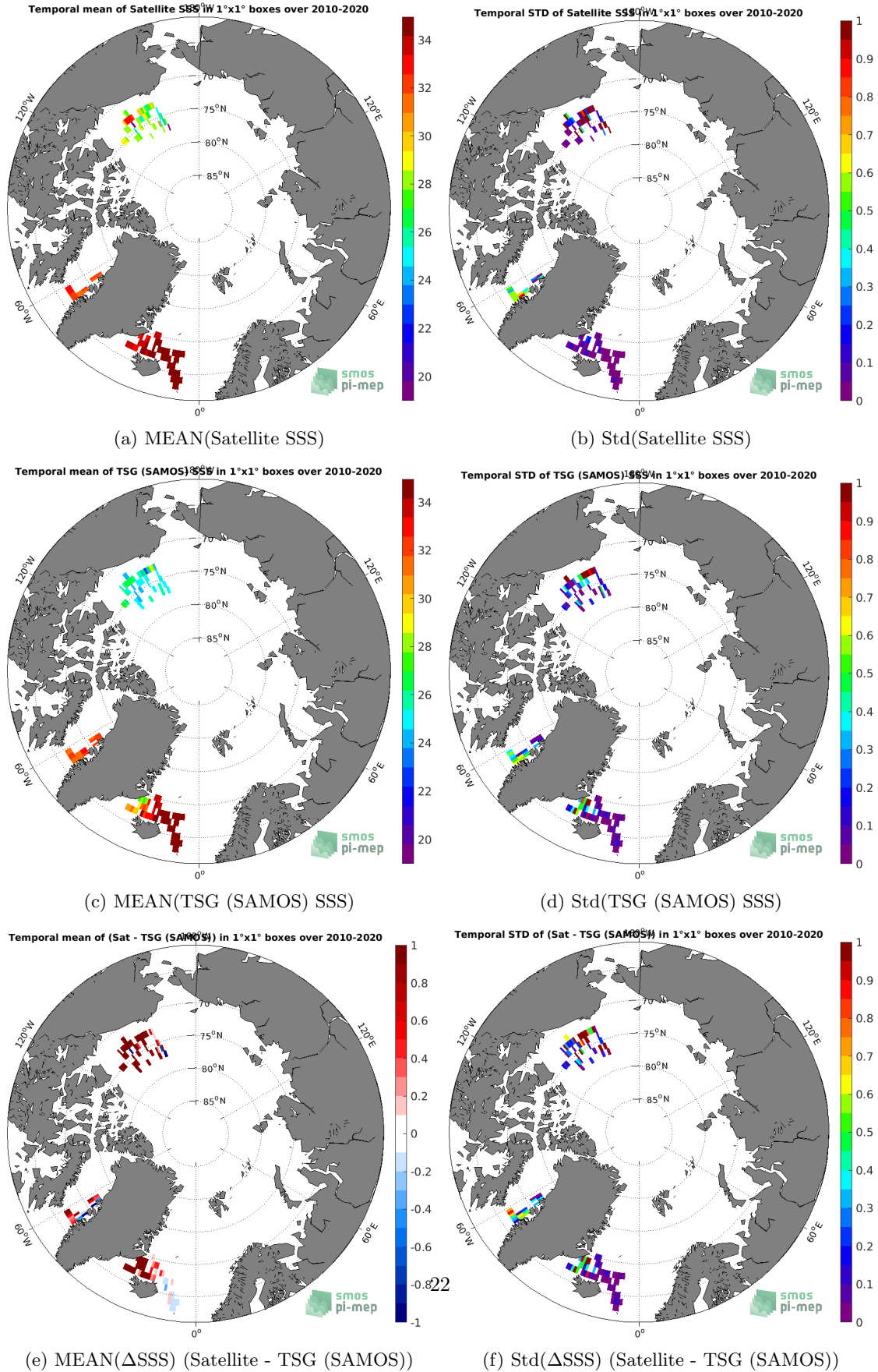
Figure 6: Temporal mean (left) and Std (right) of SSS from CCI SSS L4 Merged-OI v3.2 - 7-day running (ESA) (top), TSG (SAMOS) (middle), and of \Delta SSS (Satellite - TSG (SAMOS)). Only match-up pairs are used to generate these maps.
