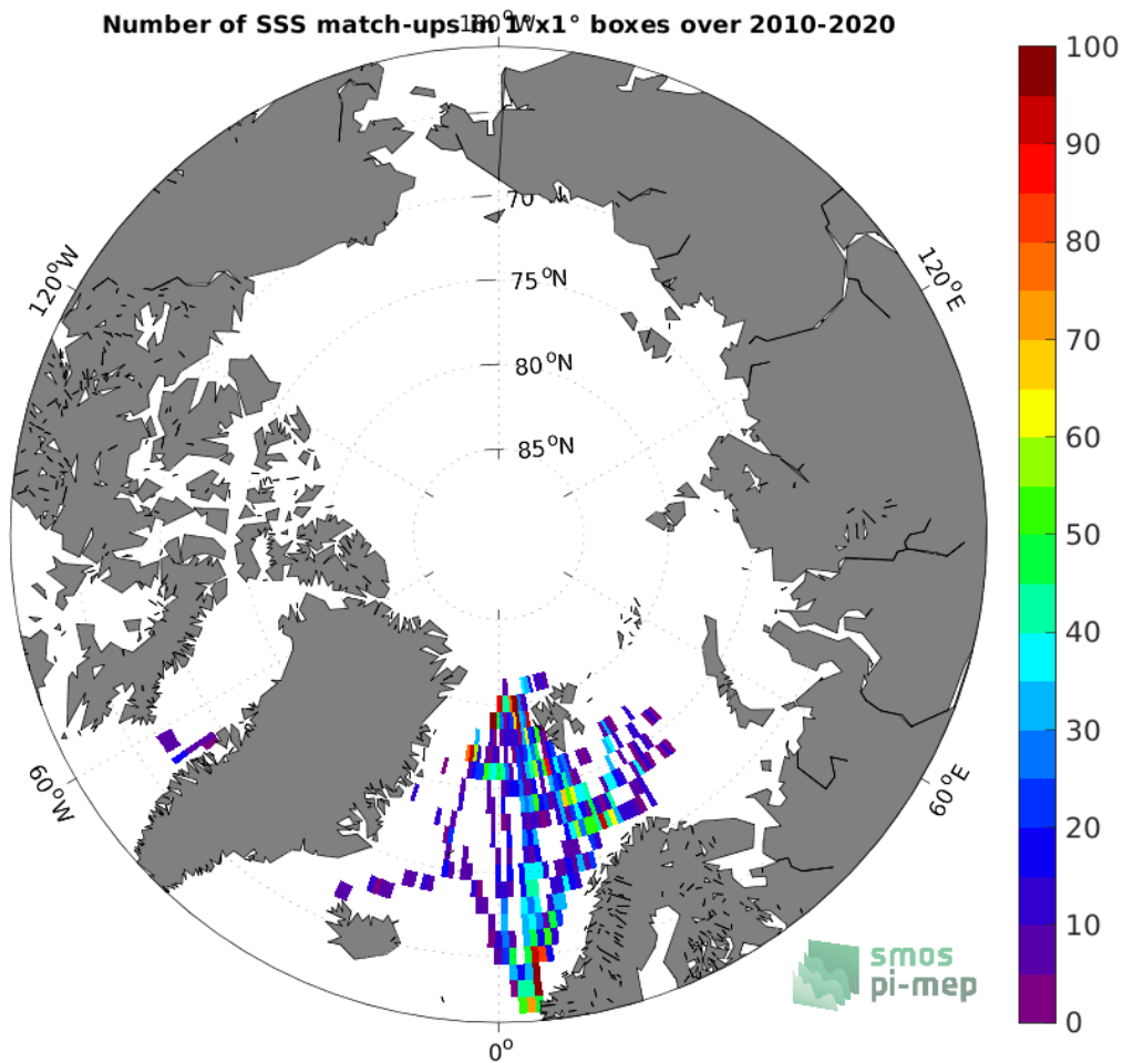
Figure 4: Number of SSS match-ups between TSG (Polarstern) SSS and the CCI SSS L4 Merged-OI v3.2 - 7-day running (ESA) SSS product for the Arctic Ocean Pi-MEP region over 1^\circ \times 1^\circ boxes and for the full satellite product period.
