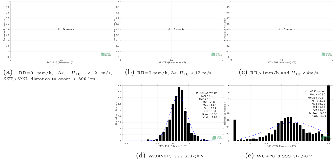
Figure 13: Normalized histogram of \Delta SSS (CCI SSS L4 Merged-OI v3.2 - 7-day running (ESA) - TSG (Polarstern)) for 5 different subdatasets corresponding to: RR=0 mm/h, 3 < U_{10} < 12 m/s, SST>5°C, distance to coast > 800 km (a), RR=0 mm/h, 3 < U_{10} < 12 m/s (b), RR>1mm/h and U_{10} < 4 m/s (c), WOA2013 SSS Std<0.2 (d), WOA2013 SSS Std>0.2 (e).
