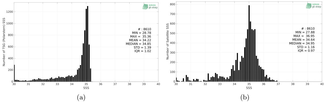
Figure 2: Histograms of SSS from TSG (Polarstern) (a) and CCI SSS L4 Merged-OI v3.2 - 7-day running (ESA) (b) considering all match-up pairs per bins of 0.1 over the Arctic Ocean Pi-MEP region and for the full satellite product period.
