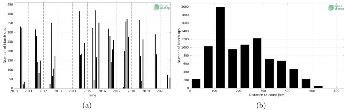
Figure 1: Number of match-ups between TSG (Polarstern) and CCI SSS L4 Merged-OI v3.2 - 7-day running (ESA) SSS as a function of time (a) and as function of the distance to coast (b) over the Arctic Ocean Pi-MEP region and for the full satellite product period.
