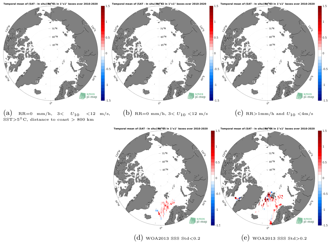
Figure 12: Temporal mean gridded over spatial boxes of size 1^{\circ}\times 1^{\circ} of \Delta\text{SSS} (CCI SSS L4 Merged-OI v3.2 - 7-day running (ESA) - TSG (Polarstern)) for 5 different subdatasets corresponding to:RR=0 mm/h, 3 < U_{10} < 12 m/s, SST >5^{\circ}\text{C} , distance to coast > 800 km (a), RR=0 mm/h, 3 < U_{10} < 12 m/s (b), RR >1 mm/h and U_{10} < 4 m/s (c), WOA2013 SSS Std <0.2 (d), WOA2013 SSS Std >0.2 (e).
