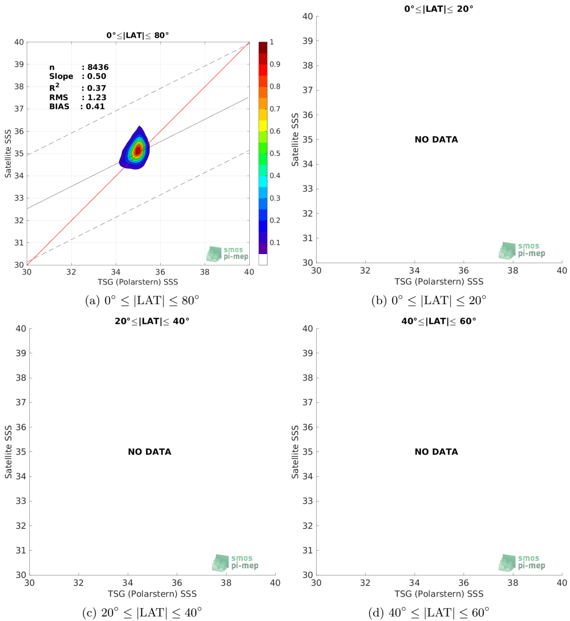
Figure 9: Contour maps of the concentration of CCI SSS L4 Merged-OI v3.2 - 7-day running (ESA) SSS (y-axis) versus TSG (Polarstern) SSS (x-axis) at match-up pairs for different latitude bands. For each plot, the red line shows x=y . The black thin and dashed lines indicate a linear fit through the data cloud and the \pm 95\% confidence levels, respectively. The number match-up pairs n , the slope and R^2 coefficient of the linear fit, the root mean square (RMS) and the mean bias between satellite and in situ data are indicated for each latitude band in each plots.
