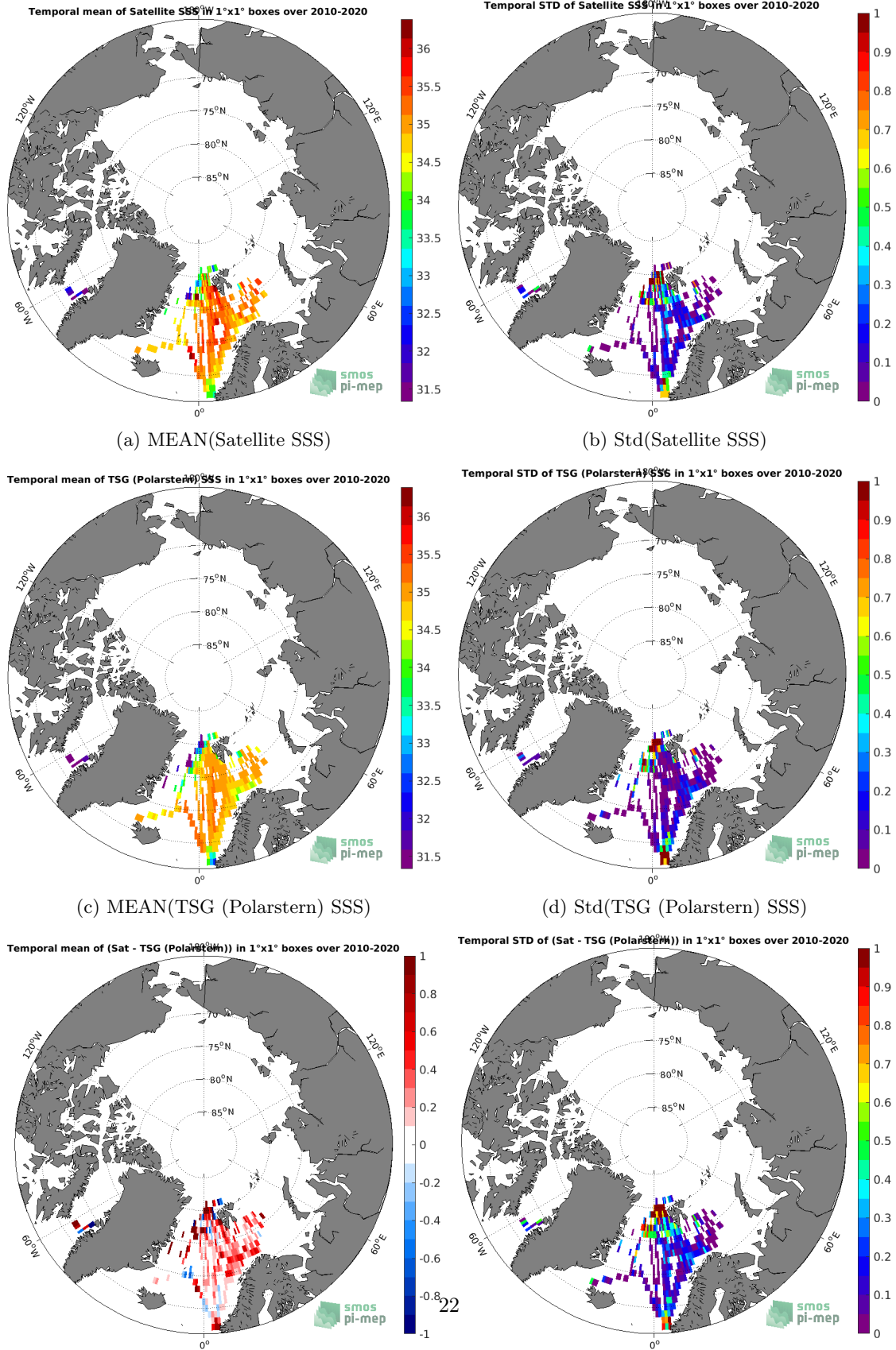
Figure 6: Temporal mean (left) and Std (right) of SSS from CCI SSS L4 Merged-OI v3.2 - 7-day running (ESA) (top), TSG (Polarstern) (middle), and of \Delta SSS (Satellite - TSG (Polarstern)). Only match-up pairs are used to generate these maps.
