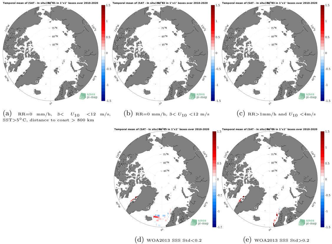
Figure 12: Temporal mean gridded over spatial boxes of size 1^{\circ}\times 1^{\circ} of \Delta\text{SSS} (CCI SSS L4 Merged-OI v3.2 - 7-day running (ESA) - TSG (LEGOS-DM)) for 5 different subdatasets corresponding to: RR=0 mm/h, 3 < U_{10} < 12 m/s, SST > 5^{\circ}\text{C} , distance to coast > 800 km (a), RR=0 mm/h, 3 < U_{10} < 12 m/s (b), RR > 1 mm/h and U_{10} < 4 m/s (c), WOA2013 SSS Std < 0.2 (d), WOA2013 SSS Std > 0.2 (e).
