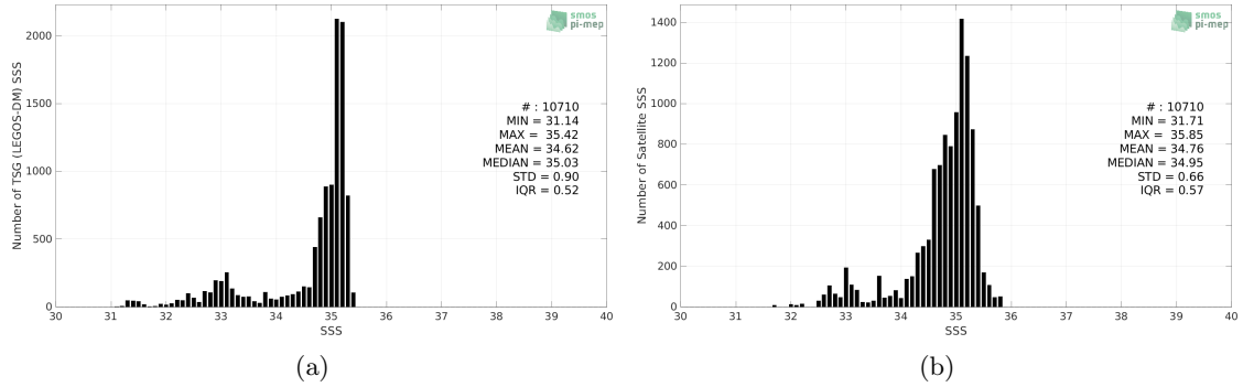
Figure 2: Histograms of SSS from TSG (LEGOS-DM) (a) and CCI SSS L4 Merged-OI v3.2 - 7-day running (ESA) (b) considering all match-up pairs per bins of 0.1 over the Arctic Ocean Pi-MEP region and for the full satellite product period.
