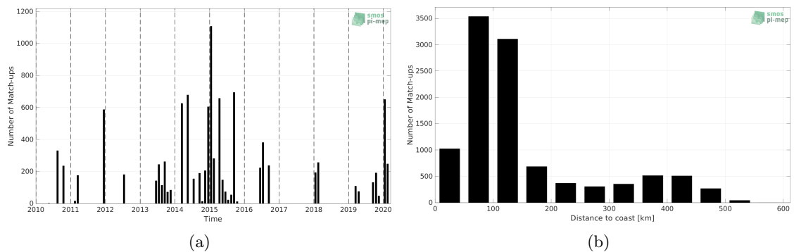
Figure 1: Number of match-ups between TSG (LEGOS-DM) and CCI SSS L4 Merged-OI v3.2 - 7-day running (ESA) SSS as a function of time (a) and as function of the distance to coast (b) over the Arctic Ocean Pi-MEP region and for the full satellite product period.
