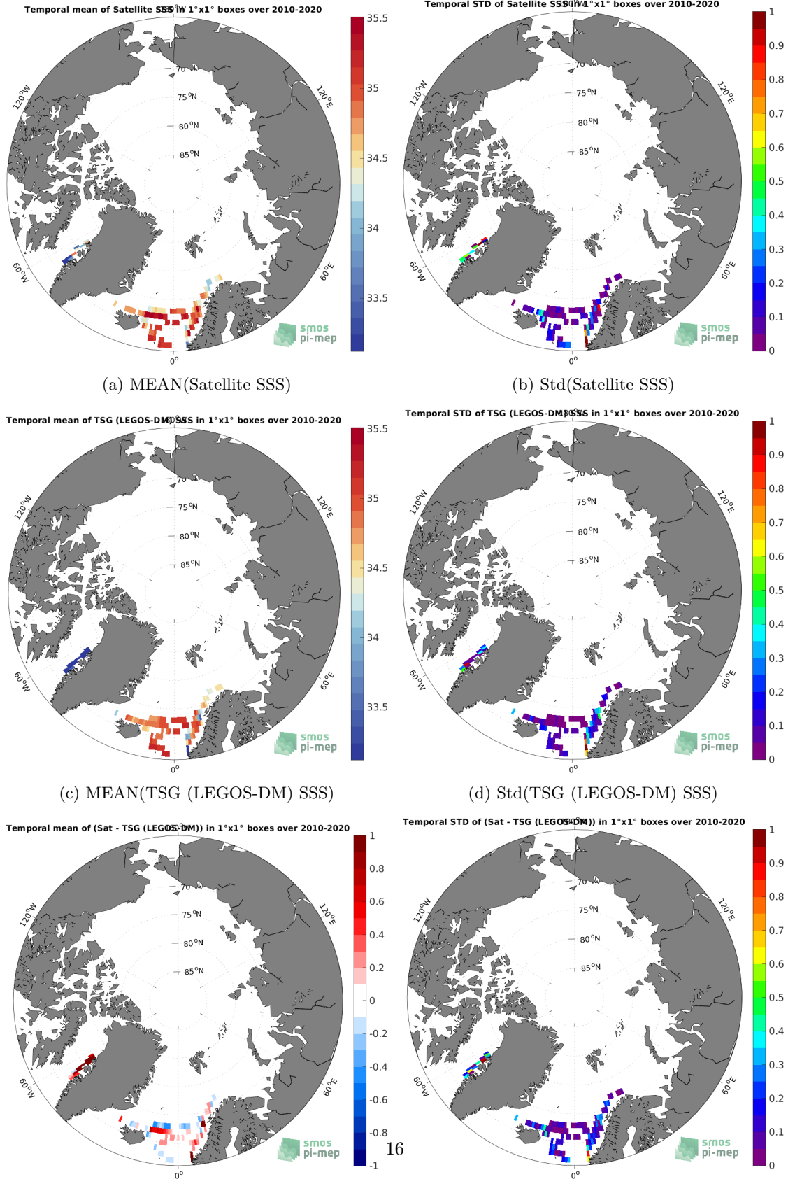
(e) MEAN( \Delta SSS) (Satellite - TSG (LEGOS-DM)) (f) Std( \Delta SSS) (Satellite - TSG (LEGOS-DM)) Figure 6: Temporal mean (left) and Std (right) of SSS from CCI SSS L4 Merged-OI v3.2 - 7-day running (ESA) (top), TSG (LEGOS-DM) (middle), and of \Delta SSS (Satellite - TSG (LEGOS-DM)). Only match-up pairs are used to generate these maps.
