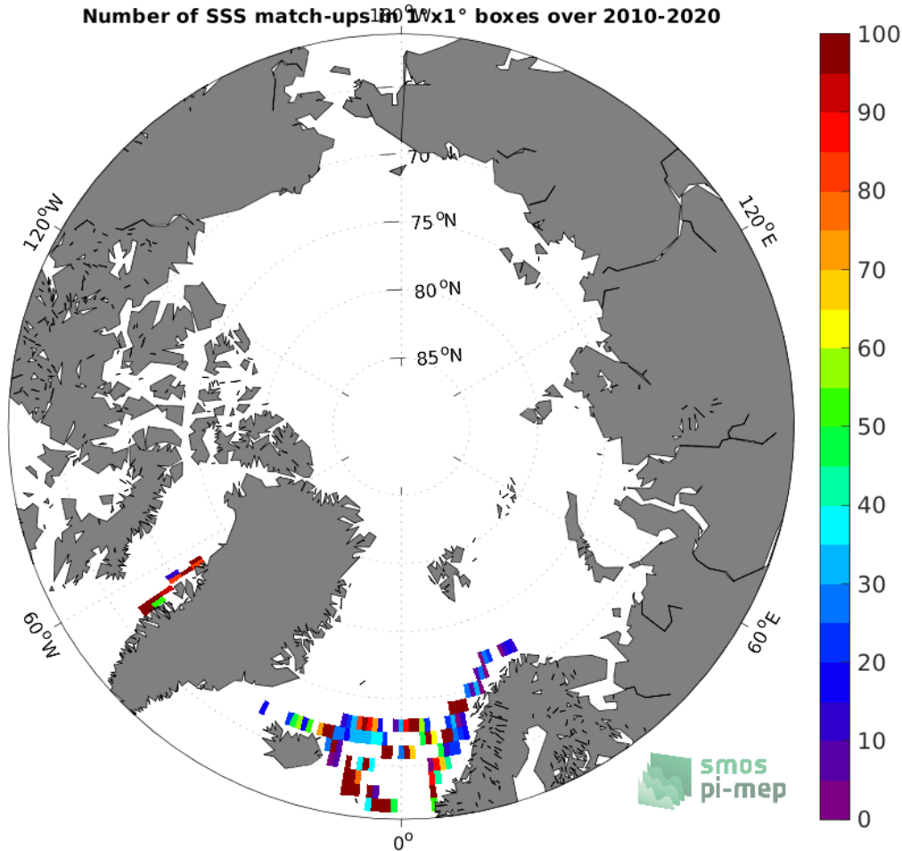
Figure 4: Number of SSS match-ups between TSG (LEGOS-DM) SSS and the CCI SSS L4 Merged-OI v3.2 - 7-day running (ESA) SSS product for the Arctic Ocean Pi-MEP region over 1^\circ \times 1^\circ boxes and for the full satellite product period.
