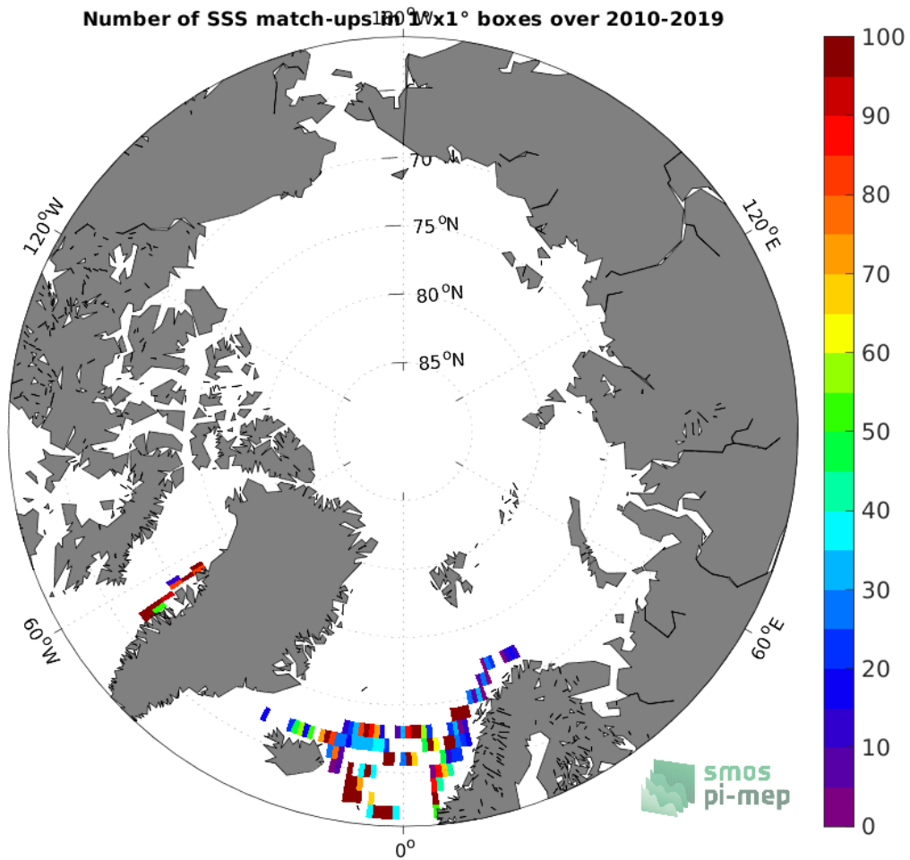
Figure 4: Number of SSS match-ups between TSG (LEGOS-DM) SSS and the CCI SSS L4 Merged-OI v3.2 - 7-day running (ESA) SSS product for the Arctic Ocean Pi-MEP region over 1^{\circ} \times 1^{\circ} boxes and for the full satellite product period.
