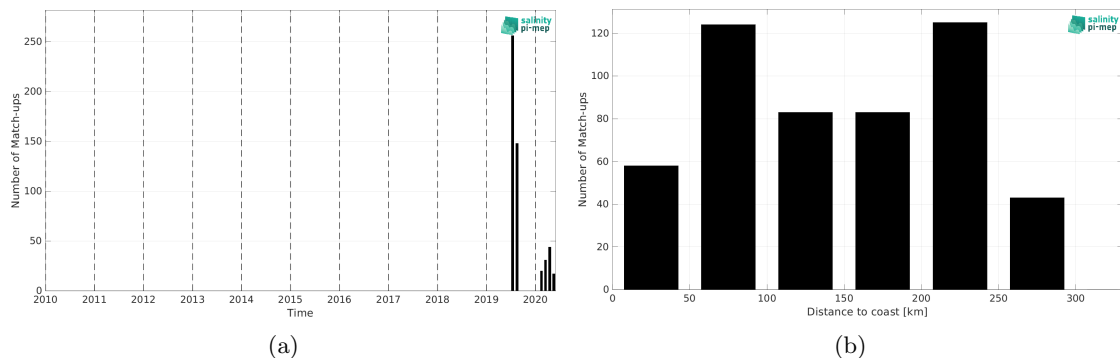
Figure 1: Number of match-ups between TSG (Lauge-Koch) and CCI SSS L4 Merged-OI v3.2 - 7-day running (ESA) SSS as a function of time (a) and as function of the distance to coast (b) over the Arctic Ocean Pi-MEP region and for the full satellite product period.
