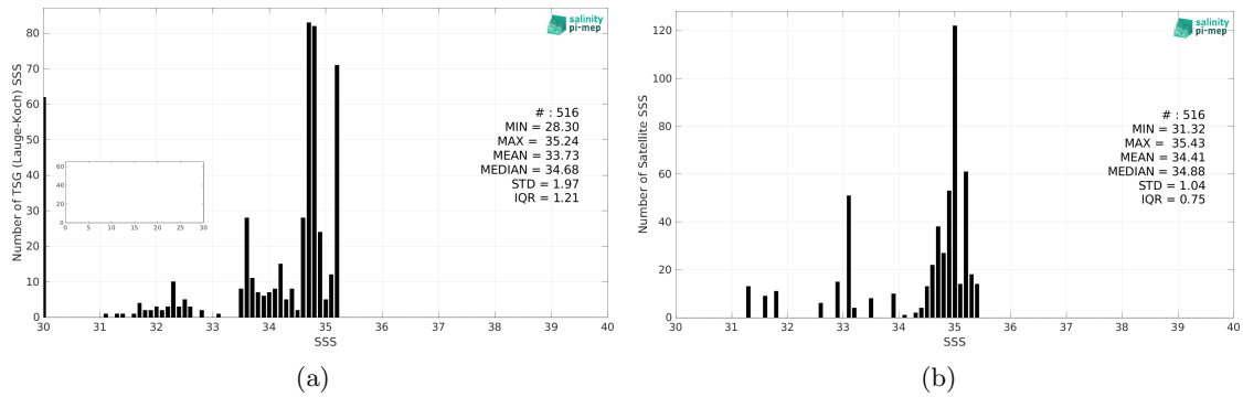
Figure 2: Histograms of SSS from TSG (Lauge-Koch) (a) and CCI SSS L4 Merged-OI v3.2 - 7-day running (ESA) (b) considering all match-up pairs per bins of 0.1 over the Arctic Ocean Pi-MEP region and for the full satellite product period.
