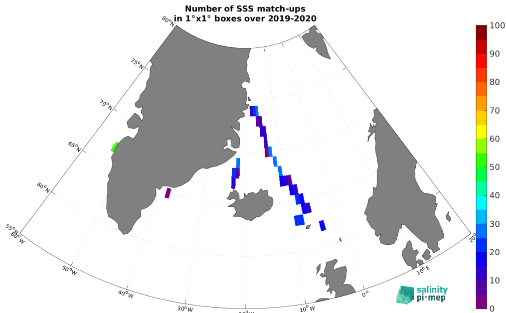
Figure 4: Number of SSS match-ups between TSG (Lauge-Koch) SSS and the CCI SSS L4 Merged-OI v3.2 - 7-day running (ESA) SSS product for the Arctic Ocean Pi-MEP region over 1^\circ \times 1^\circ boxes and for the full satellite product period.
