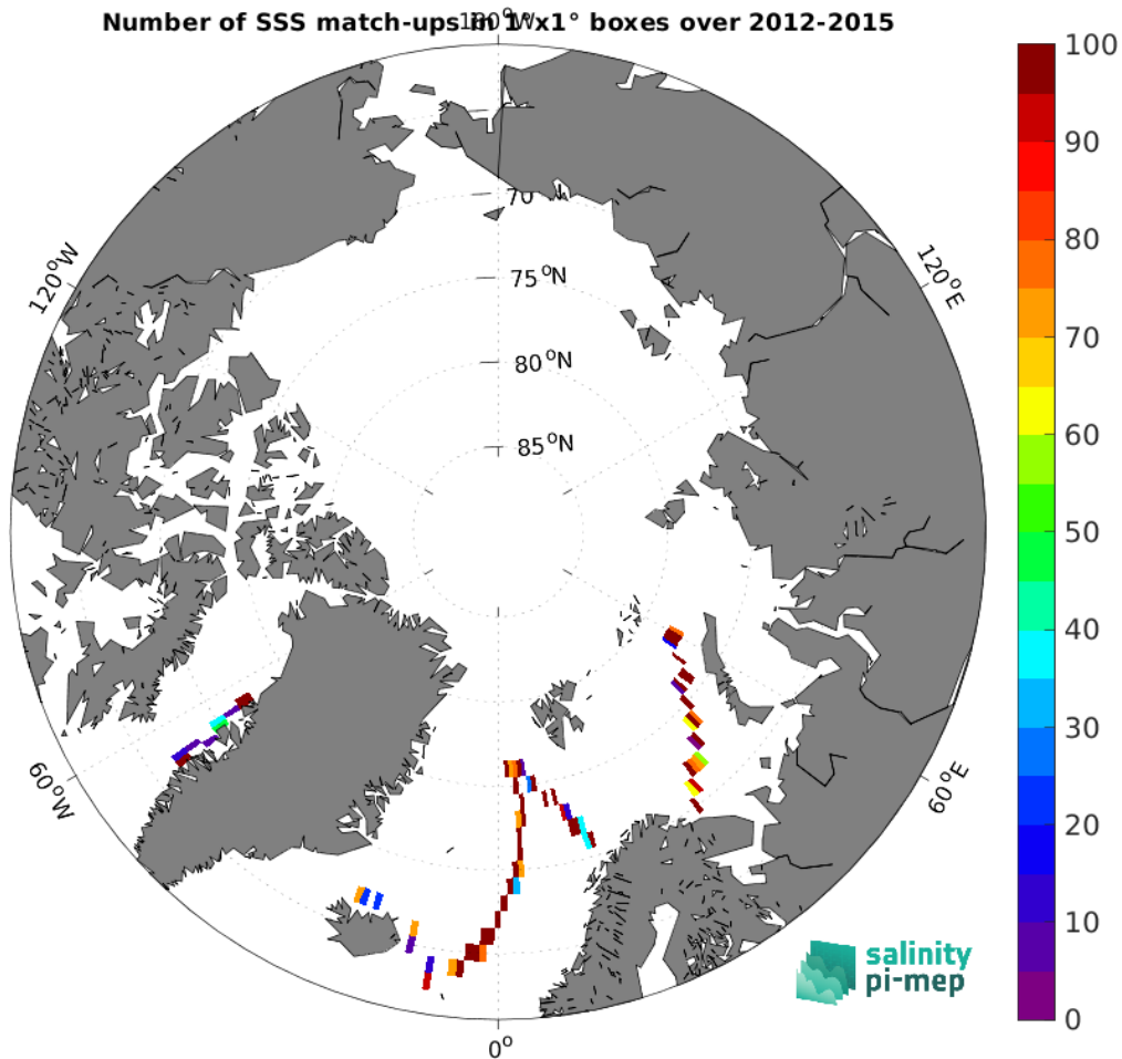
Figure 4: Number of SSS match-ups between TSG (GOSUD-Sailing-ship) SSS and the CCI SSS L4 Merged-OI v3.2 - 7-day running (ESA) SSS product for the Arctic Ocean Pi-MEP region over 1^\circ \times 1^\circ boxes and for the full satellite product period.
