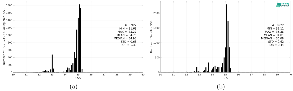
Figure 2: Histograms of SSS from TSG (GOSUD-Sailing-ship) (a) and CCI SSS L4 Merged-OI v3.2 - 7-day running (ESA) (b) considering all match-up pairs per bins of 0.1 over the Arctic Ocean Pi-MEP region and for the full satellite product period.
