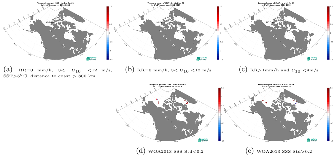
Figure 12: Temporal mean gridded over spatial boxes of size 1^{\circ}\times 1^{\circ} of \Delta\text{SSS} (CCI SSS L4 Merged-OI v3.2 - 7-day running (ESA) - TSG (Amundsen)) for 5 different subdatasets corresponding to:RR=0 mm/h, 3 < U_{10} < 12 m/s, SST > 5^{\circ}\text{C} , distance to coast > 800 km (a), RR=0 mm/h, 3 < U_{10} < 12 m/s (b), RR > 1 mm/h and U_{10} < 4 m/s (c), WOA2013 SSS Std < 0.2 (d), WOA2013 SSS Std > 0.2 (e).
