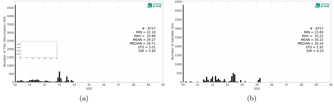
Figure 2: Histograms of SSS from TSG (Amundsen) (a) and CCI SSS L4 Merged-OI v3.2 - 7-day running (ESA) (b) considering all match-up pairs per bins of 0.1 over the Arctic Ocean Pi-MEP region and for the full satellite product period.
