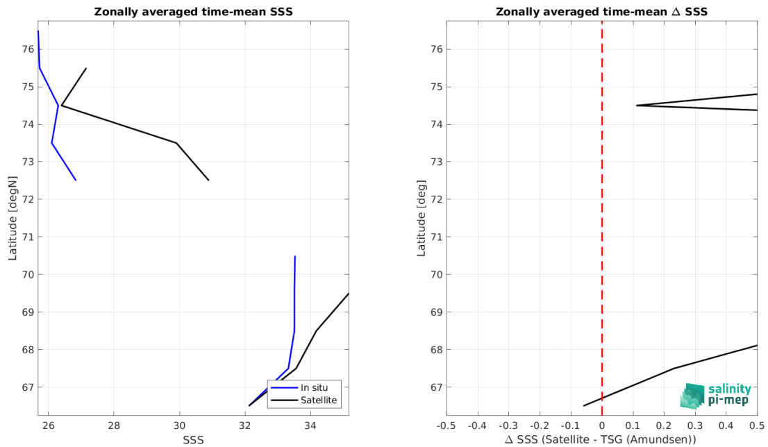
Figure 8: Left panel: Zonal mean SSS from CCI SSS L4 Merged-OI v3.2 - 7-day running (ESA) satellite product (black) and from TSG (Amundsen) (blue). Right panel: Zonal mean of \Delta SSS (Satellite - TSG (Amundsen)) for all the collected Pi-MEP match-up pairs estimated over the full satellite product period.
