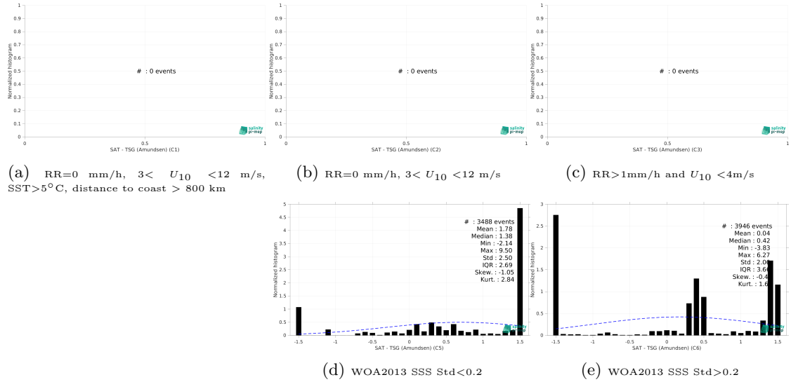
Figure 13: Normalized histogram of \Delta SSS (CCI SSS L4 Merged-OI v3.2 - 7-day running (ESA) - TSG (Amundsen)) for 5 different subdatasets corresponding to: RR=0 mm/h, 3 < U_{10} < 12 m/s, SST>5°C, distance to coast > 800 km (a), RR=0 mm/h, 3 < U_{10} < 12 m/s (b), RR>1mm/h and U_{10} < 4 m/s (c), WOA2013 SSS Std<0.2 (d), WOA2013 SSS Std>0.2 (e).
