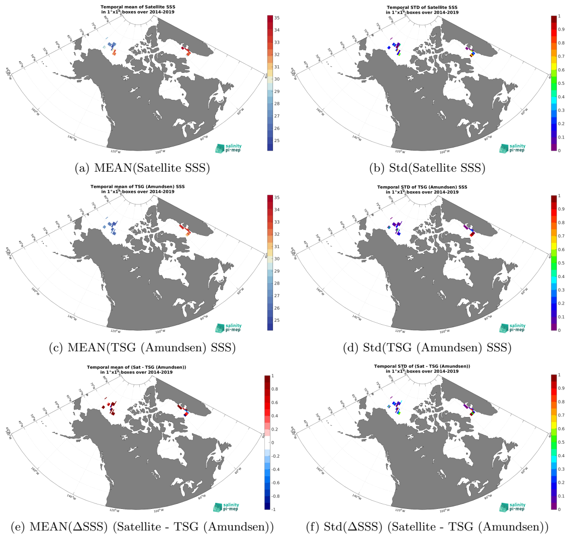
Figure 6: Temporal mean (left) and Std (right) of SSS from CCI SSS L4 Merged-OI v3.2 - 7-day running (ESA) (top), TSG (Amundsen) (middle), and of \Delta SSS (Satellite - TSG (Amundsen)). Only match-up pairs are used to generate these maps.
