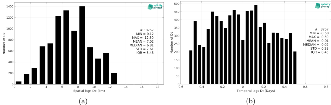
Figure 5: Histograms of the spatial (a) and temporal (b) lags between the location/time of the TSG (Amundsen) measurement and the date of the corresponding CCI SSS L4 Merged-OI v3.2 - 7-day running (ESA) SSS pixel.
