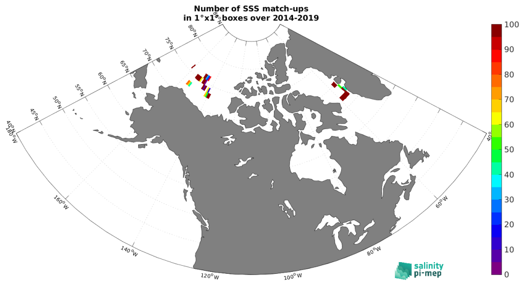
Figure 4: Number of SSS match-ups between TSG (Amundsen) SSS and the CCI SSS L4 Merged-OI v3.2 - 7-day running (ESA) SSS product for the Arctic Ocean Pi-MEP region over 1°x1° boxes and for the full satellite product period.
