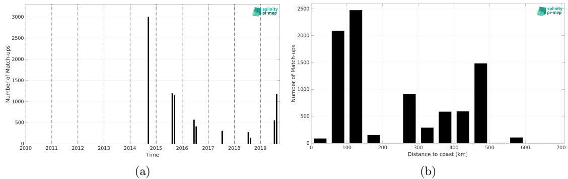
Figure 1: Number of match-ups between TSG (Amundsen) and CCI SSS L4 Merged-OI v3.2 - 7-day running (ESA) SSS as a function of time (a) and as function of the distance to coast (b) over the Arctic Ocean Pi-MEP region and for the full satellite product period.
