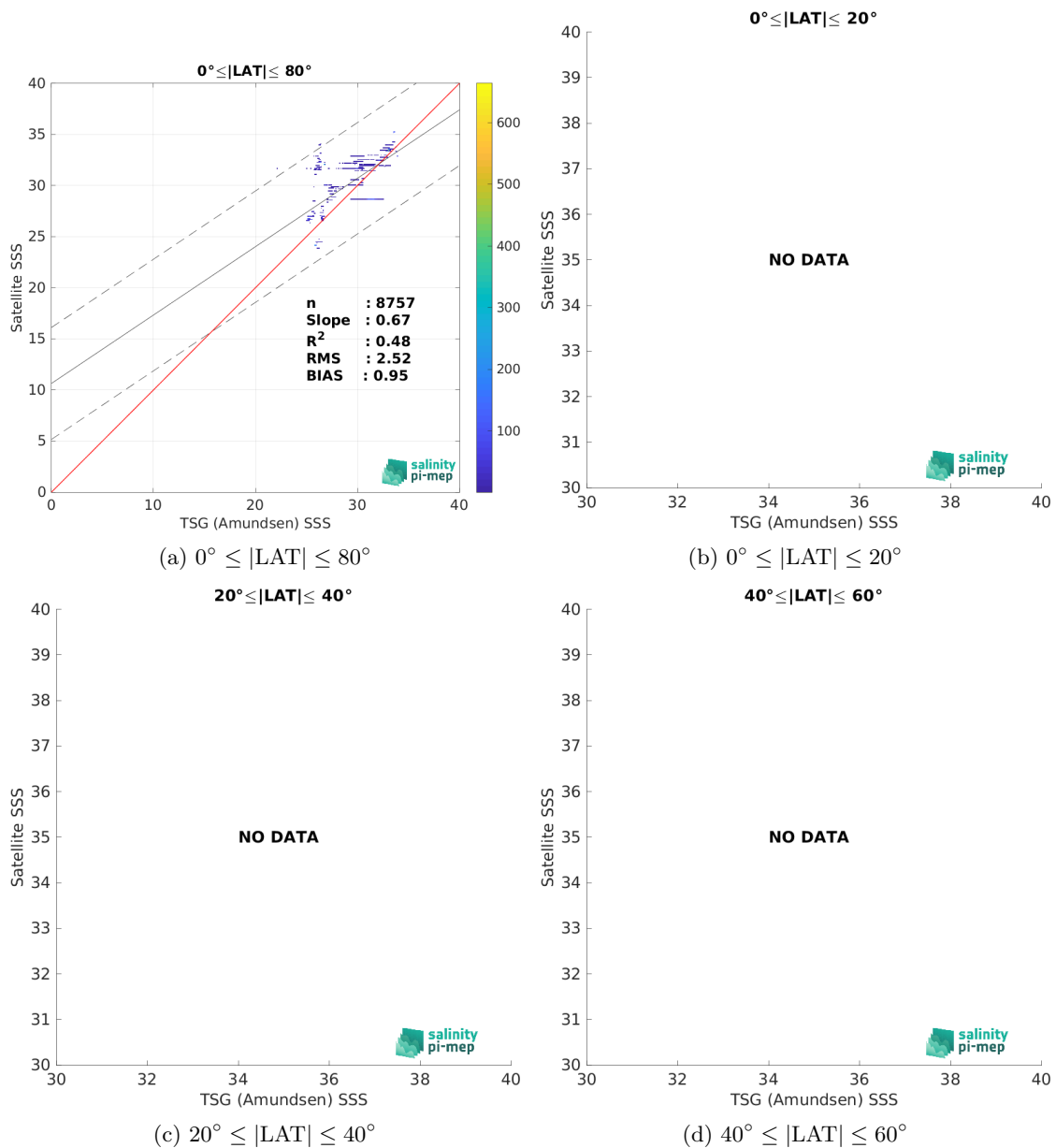
Figure 9: Contour maps of the concentration of CCI SSS L4 Merged-OI v3.2 - 7-day running (ESA) SSS (y-axis) versus TSG (Amundsen) SSS (x-axis) at match-up pairs for different latitude bands. For each plot, the red line shows x=y . The black thin and dashed lines indicate a linear fit through the data cloud and the \pm 95\% confidence levels, respectively. The number match-up pairs n , the slope and R^2 coefficient of the linear fit, the root mean square (RMS) and the mean bias between satellite and in situ data are indicated for each latitude band in each plots.
