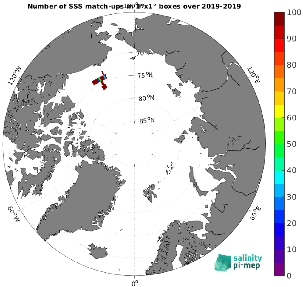
Figure 4: Number of SSS match-ups between Saildrone SSS and the CCI SSS L4 Merged-OI v3.2 - 7-day running (ESA) SSS product for the Arctic Ocean Pi-MEP region over 1^\circ \times 1^\circ boxes and for the full satellite product period.
