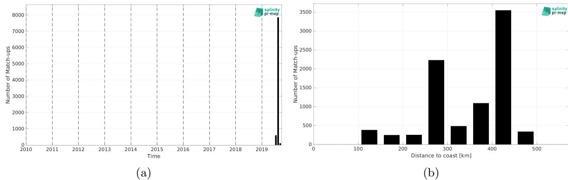
Figure 1: Number of match-ups between Saildrone and CCI SSS L4 Merged-OI v3.2 - 7-day running (ESA) SSS as a function of time (a) and as function of the distance to coast (b) over the Arctic Ocean Pi-MEP region and for the full satellite product period.
