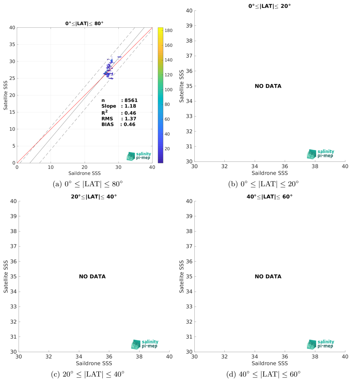
Figure 9: Contour maps of the concentration of CCI SSS L4 Merged-OI v3.2 - 7-day running (ESA) SSS (y-axis) versus Saildrone SSS (x-axis) at match-up pairs for different latitude bands. For each plot, the red line shows x=y . The black thin and dashed lines indicate a linear fit through the data cloud and the \pm 95\% confidence levels, respectively. The number match-up pairs n , the slope and R^2 coefficient of the linear fit, the root mean square (RMS) and the mean bias between satellite and in situ data are indicated for each latitude band in each plots.
