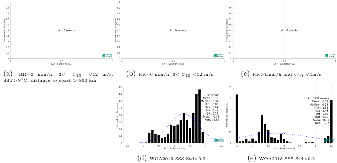
Figure 13: Normalized histogram of \Delta SSS (CCI SSS L4 Merged-OI v3.2 - 7-day running (ESA) - Saildrone) for 5 different subdatasets corresponding to: RR=0 mm/h, 3 < U_{10} < 12 m/s, SST >5^{\circ} C, distance to coast > 800 km (a), RR=0 mm/h, 3 < U_{10} < 12 m/s (b), RR >1 mm/h and U_{10} < 4 m/s (c), WOA2013 SSS Std <0.2 (d), WOA2013 SSS Std >0.2 (e).
