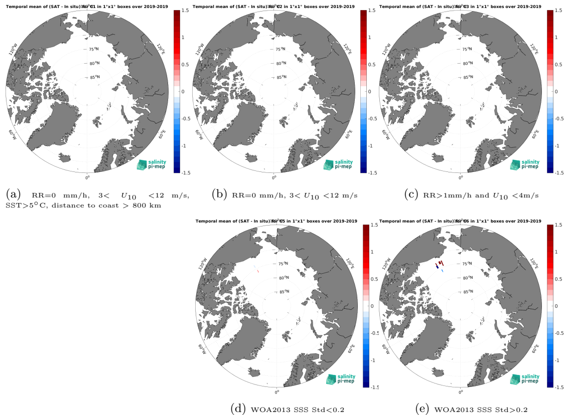
Figure 12: Temporal mean gridded over spatial boxes of size 1^{\circ}\times 1^{\circ} of \Delta\text{SSS} (CCI SSS L4 Merged-OI v3.2 - 7-day running (ESA) - Sailability) for 5 different subdatasets corresponding to: RR=0 mm/h, 3 < U_{10} < 12 m/s, SST > 5^{\circ}\text{C} , distance to coast > 800 km (a), RR=0 mm/h, 3 < U_{10} < 12 m/s (b), RR > 1 mm/h and U_{10} < 4 m/s (c), WOA2013 SSS Std < 0.2 (d), WOA2013 SSS Std > 0.2 (e).
